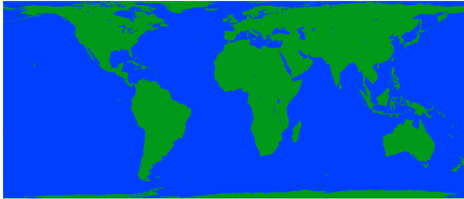
Figure 4: Global EASE-Grid 2.0.
