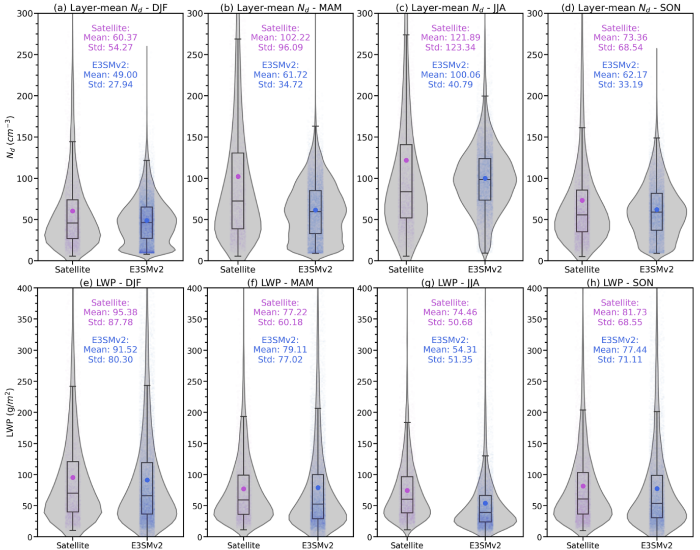
Figure 1. Violin plots of cloud droplet number concentration ( N_d , top panels) and cloud liquid water path (LWP, bottom panels) from satellite retrievals (purple) and E3SMv2 simulations (blue), during winter, DJF (a, e), spring, MAM (b, f), summer, JJA (c, g), and fall, SON (d, h). The mean value is indicated by the color-coded dot. The smoothed shape of each violin shows the Gaussian kernel density estimate (KDE). From top to bottom within each violin, the box plot lines represent the third quartile (Q3, 75th percentile), median (Q2, 50th percentile), and first quartile (Q1, 25th percentile), respectively. The upper whisker extends to Q3 + 1.5 \times \text{IQR} (interquartile range), and the lower whisker extends to Q1 - 1.5 \times \text{IQR} .
