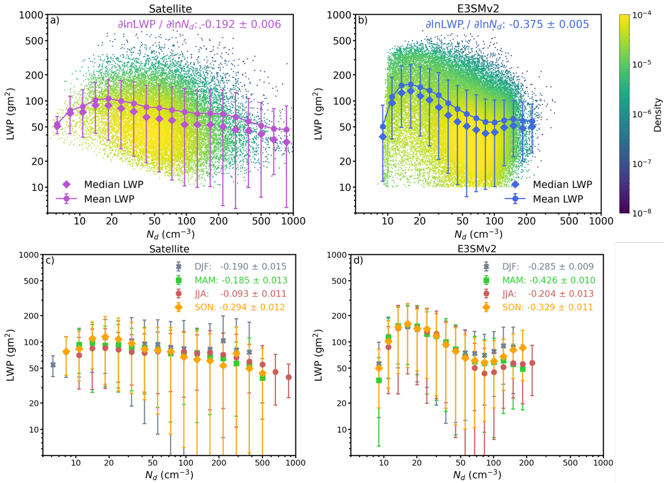
Figure 2. Top Panel: Bulk LWP binned as a function of N_d from a) satellite and b) E3SMv2, the Gaussian kernel density estimate (KDE) is shown as color-shaded scatter points area; Bottom panel: seasonality of the LWP dependences from c) satellite and d) E3SMv2.
