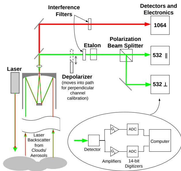
Figure 3.2. Functional block diagram of CALIOP
