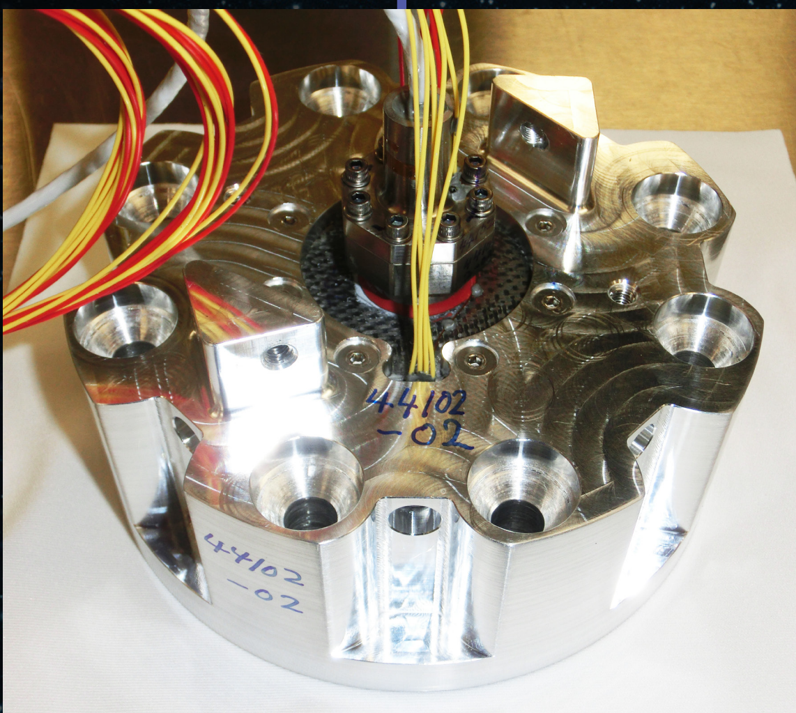
Optical Recession Sensor
