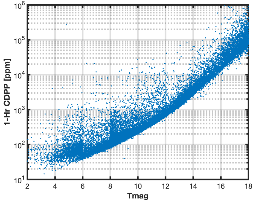
Figure 3: 1-hour CDPP. The points are RMS CDPP measurements for the 27374 light curves from the Sectors 14 – 78 multi-sector search plotted as a function of TESS magnitude.
