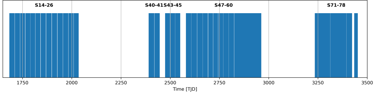
Figure 2: Observation times for sectors included in this multi-sector transit search run. Note: most targets were observed for only a subset of these sectors.
