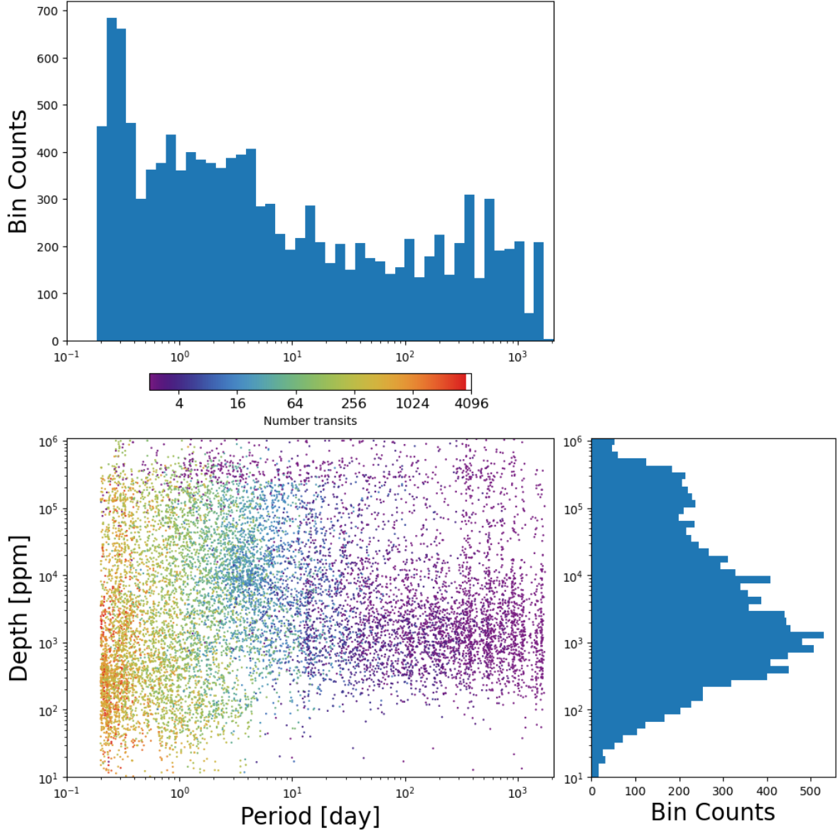
Figure 4: Lower Left Panel: Transit depth as a function of orbital period for the 12595 TCEs identified for the Sectors 14 – 78 multi-sector search. The color of the points indicates the number of transit events that were observed for the TCE. Reported depth comes from the DV limb darkened transit fit depth when available (or the DV trapezoid model fit depth if the limb darkened transit fit is not available). Top Panel: Orbital period distribution of the TCEs shown in the lower left panel. Right Panel: Transit depth distribution for the TCEs shown in the lower left panel.
