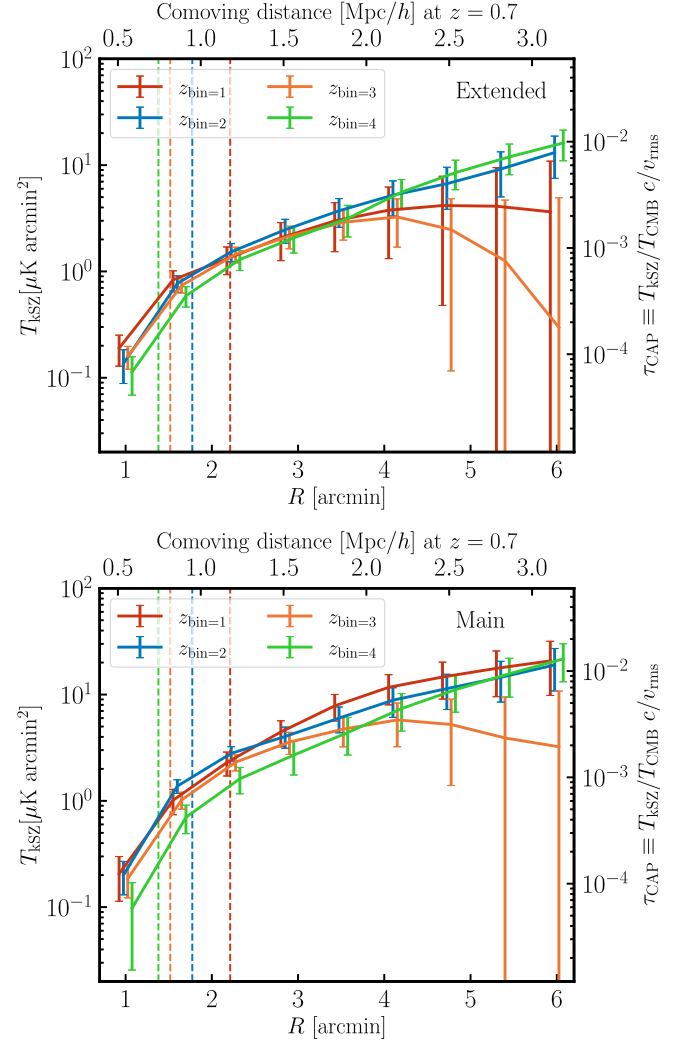
FIG. 1. Stacked kSZ signal in each redshift bin of the photometric LRG sample (top: Extended, bottom: Main) as a function of radius of the CAP filter, which approximately corresponds to the distance from the galaxy group center associated with the LRGs. The kSZ signal is obtained by stacking the hILC ACT DR6 map (with an effective FWHM = 1.6') and is detected at >10\sigma relative to dark matter in each bin (see Table I). The vertical dashed line indicates the mean virial radius of the host halos for each bin. We show the full covariance of the data in Appendix B and note that the points at large aperture are significantly correlated. We see that the gas profile is well-extended beyond the virial radius, suggesting that the feedback activity in LRG halos is strong enough to push much of the gas away from the galaxy group center. The top x -axis and the right y -axis show the comoving distance and \tau_{\text{CAP}} at the mean redshift.
