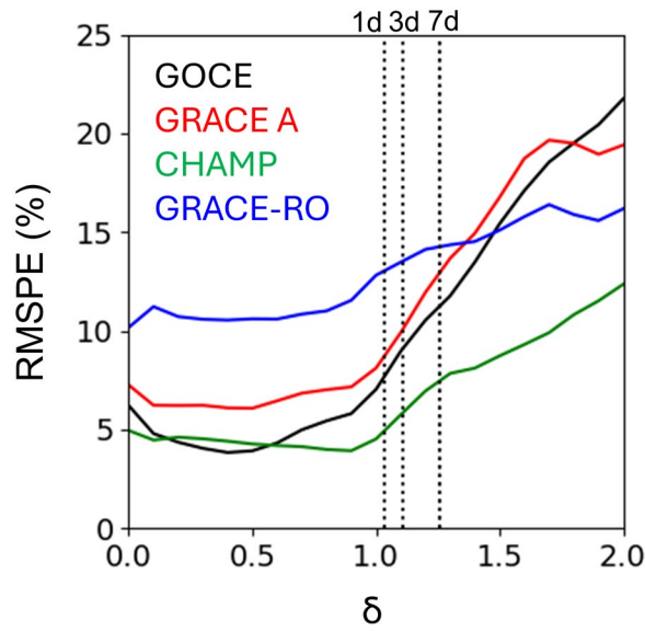
Figure 4. RMSPE as a function of \delta for the GOCE-CHAMP-GRACE satellites for the intervals shown in Figure 3. The more accurate parameterization fit occurs near the time-centered case of \delta \approx 0.5 . The \delta values corresponding to 1-day, 3-day, and 7-day prediction intervals are indicated as vertical dotted lines.
