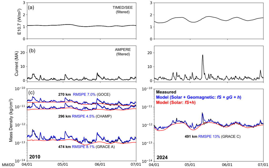
Figure 3. (a) low-pass-filtered E10.7 index (i.e., S in equation (3)) from TIMED/SEE integrated EUV irradiance from 1 to 105nm, (b) low-pass-filtered total field-aligned current (i.e., G in equation (3)) from AMPERE, (c) thermospheric mass density (i.e., \langle \rho \rangle in equation (3)) from GOCE, CHAMP, and GRACE for two four month intervals (4/1/2010-7/1/2010 (left) and 4/1/2024-7/1/2024 (right)). The results of the model fit to equation (3) are included using intervals of \tau = 27 days. The orbit-averaged variations of neutral mass density (black curve) at different altitudes are well captured by the combination of solar and geomagnetic terms (blue curve), even during extreme geomagnetic storms such as the Gannon storm on May 10-11, 2024 observed by GRACE-FO. Solar-only contributions to the neutral mass density are indicated by the red curves. Root Mean Square Percentage Error (RMSPE) calculated between the blue and black curves are included for each satellite.
