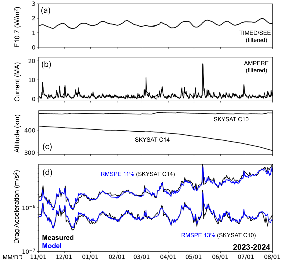
Figure 5. (a) low-pass-filtered E10.7 index (i.e., S in equation (3)) from TIMED/SEE integrated EUV irradiance from 1 to 105nm, (b) low-pass-filtered total field-aligned current (i.e., G in equation (3)) from AMPERE, and (c) altitude and (d) drag acceleration ( \langle a_{\text{drag}} \rangle ) for two commercial LEO satellites (SKYSAT C10 and SKYSAT C14). The orbit-averaged variations of drag acceleration (black curve) at different altitudes are well captured by the combination of solar and geomagnetic terms (blue curve). Root Mean Square Percentage Error (RMSPE) calculated between the blue and black curves are included for each satellite. No independent of determination of the total thermospheric mass density or the satellite B -factor was needed to accurately parameterize variations in \langle a_{\text{drag}} \rangle in terms of solar and geomagnetic drivers.
