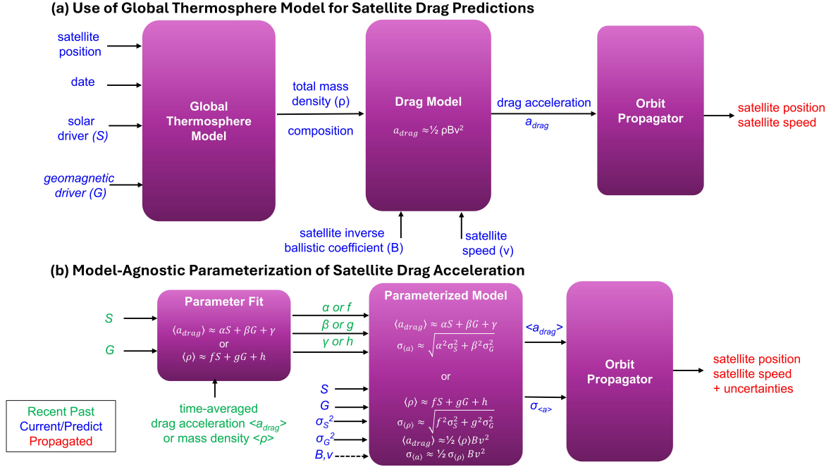
Figure 1. (a) Traditional approach to estimating satellite drag utilizing a global thermospheric model (adapted from Bruinsma et al. [2023]) for the case of a stable satellite B -factor not strongly driven by composition). (b) Alternative approach presented in this work that parameterizes past observations of drag acceleration or thermospheric mass density and energy source terms to generate predictions with readily quantified uncertainties.
