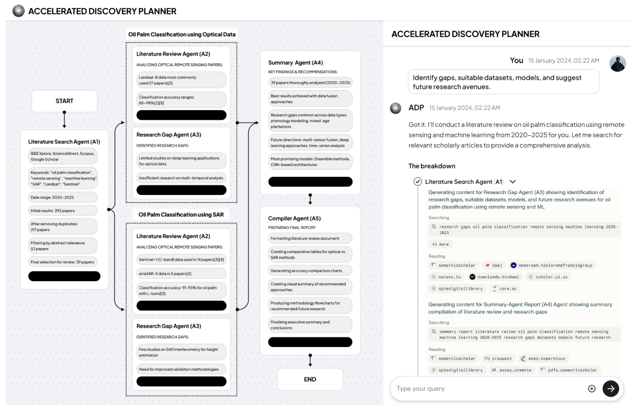
Figure 1. Illustrative mockup of an accelerated knowledge discovery (AKD) system in use. In this scenario, a researcher is investigating oil palm classification and engages the AKD system to identify current knowledge gaps, recommend suitable datasets and models, and suggest new avenues for future research. This example highlights how AKD can intelligently orchestrate the research process by synthesizing existing knowledge, surfacing relevant resources, and proposing actionable next steps to expedite scientific discovery. Researchers have control over
