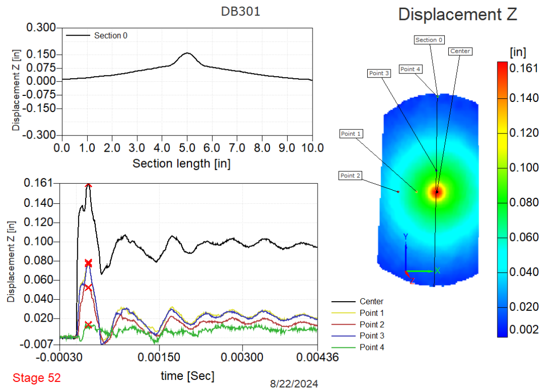
Figure C.83.—DB301: Out-of-plane displacement at time of maximum displacement.
