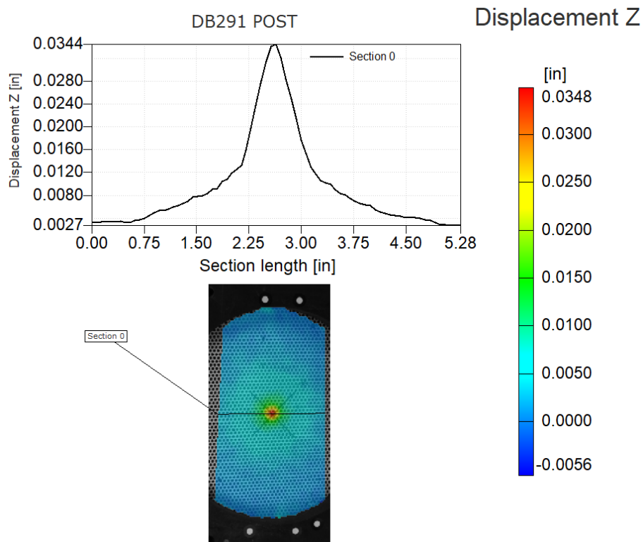
Figure C.58.—DB291: Posttest panel deformation.
