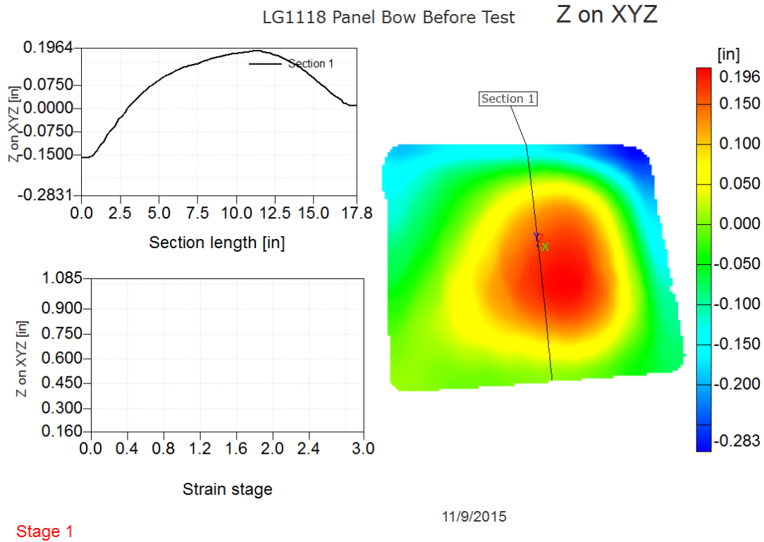
Figure D.4.—LG1118: Panel deformation from heat treatment before test.
