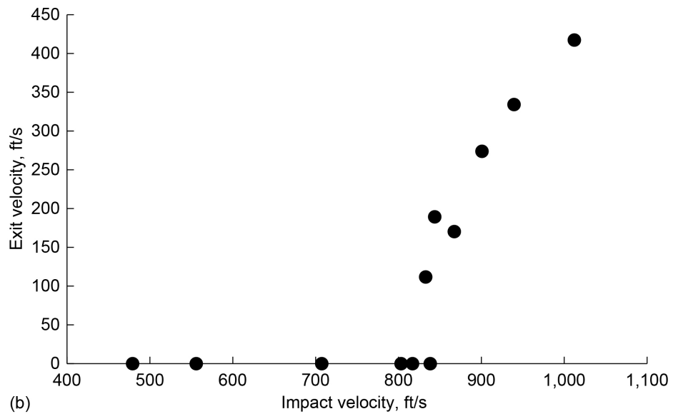
Figure 13.—Penetration results for 0.125-in. (nominal) small panels. (a) Penetration (1 = yes, 0 = no). (b) Exit velocity versus impact velocity.
