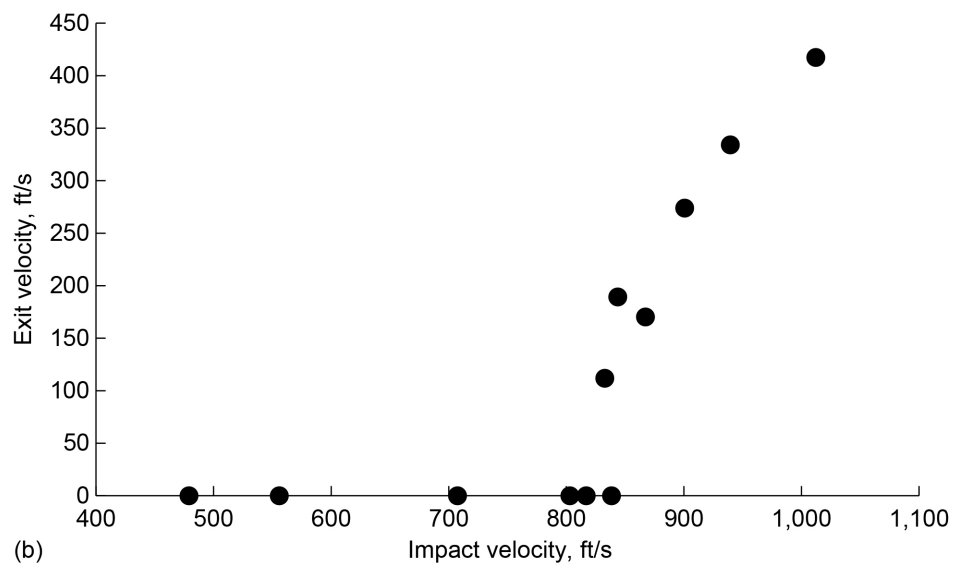
Figure 14.—Penetration results for 0.25-in. (nominal) small panels. (a) Penetration (1 = yes, 0 = no); (b) Exit velocity versus impact velocity.
