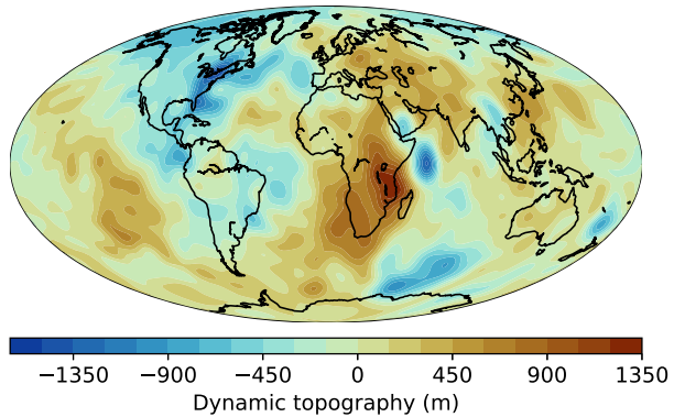
Fig. 2 The dynamically-supported component of Earth's topography as calculated by Straume et al. (2024), based on the SMEAN2 seismic tomography model. Data are available at https://doi.org/10.5281/zenodo.8262689 . Note topography supported by compositional isostasy (e.g., continents), which is excluded from this map, makes up an additional component to the total topography
