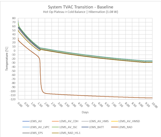
Figure 12: Temperature transition estimates in high-vacuum environment
