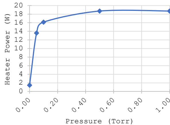
Figure 13: Heater Power vs. GN2 backfill pressure
