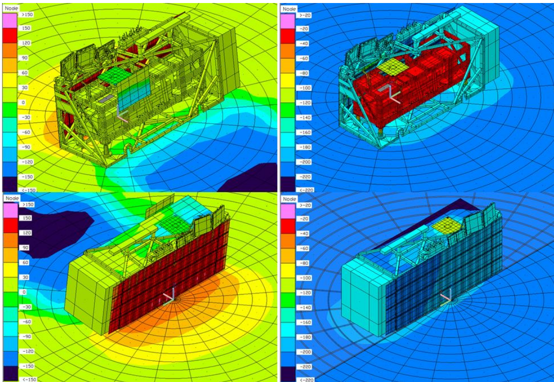
Figure 6: (left) Hot operational temperature plot at solar noon with 5° inclination. (right) Cold operational temperature plot during lunar night.
