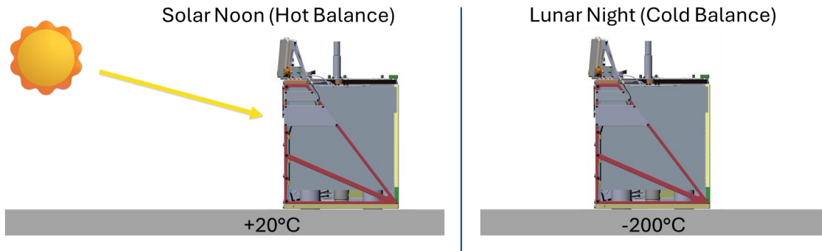
Figure 5: Thermal Environment Boundary Conditions for Hot and Cold Balance
