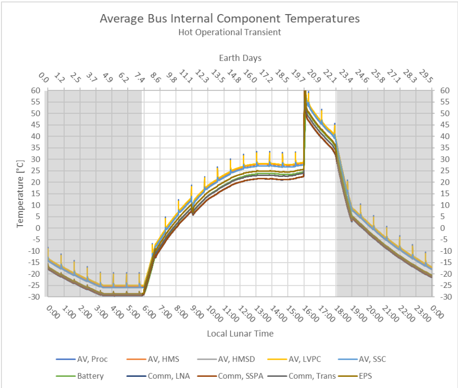
Figure 7: Bus Structure Component Temperatures over a Lunation
