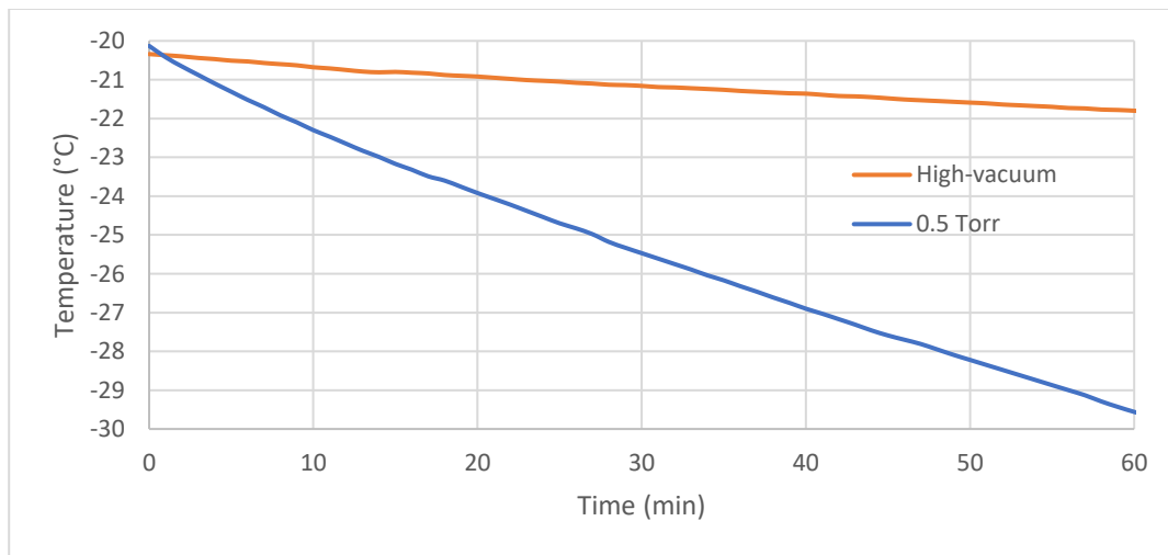
Figure 14: Temperature drop vs. time for high-vacuum and 0.5 torr pressure
