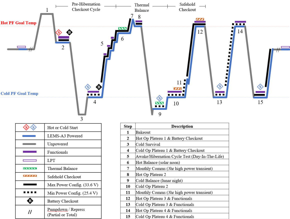
Figure 11: TVAC Test Profile
