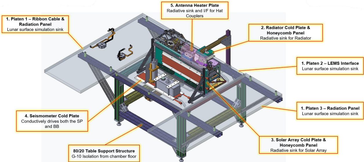
Figure 9: TVAC Test Configuration
