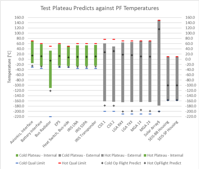
Figure 17: System TVAC Plateau Predictions Compared to Flight Predictions
