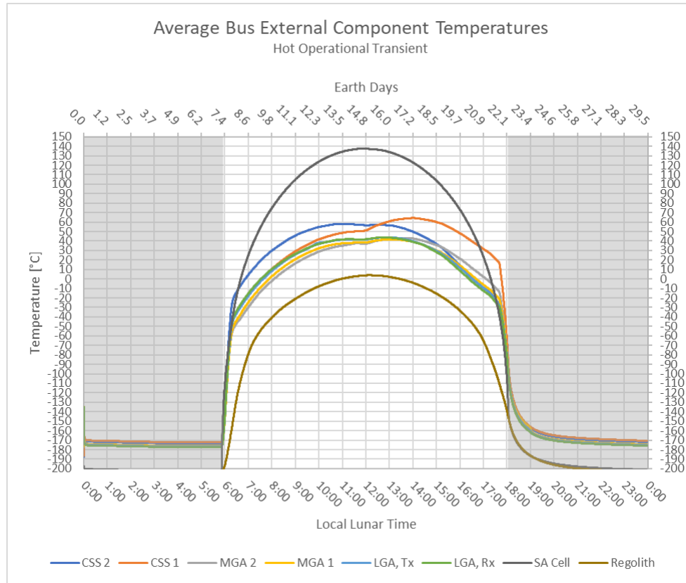
Figure 8: Superstructure Component Temperatures over a Lunation
