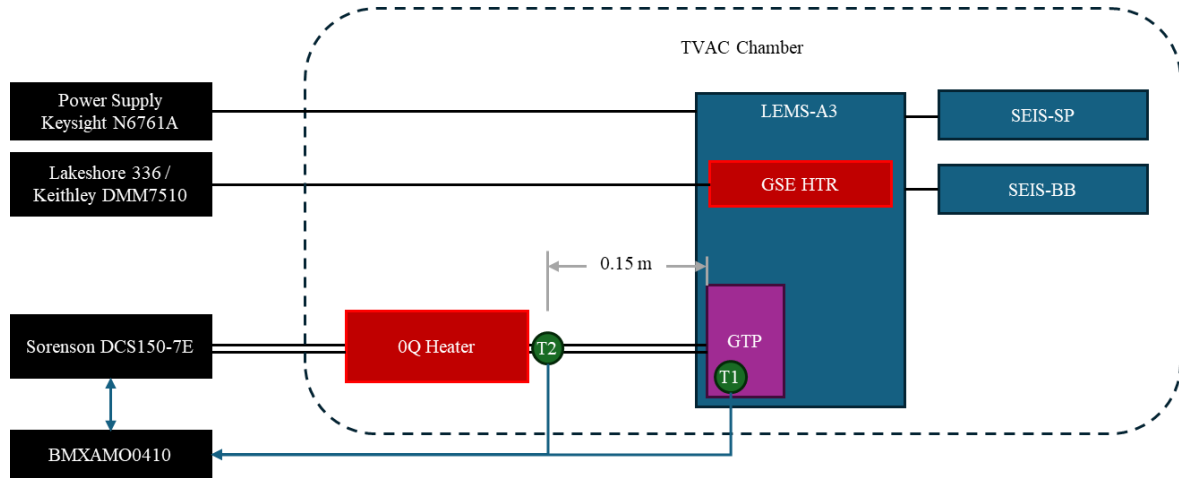
Figure 15: Thermal Balance Ground Support Equipment (to be updated for Final Submission)
