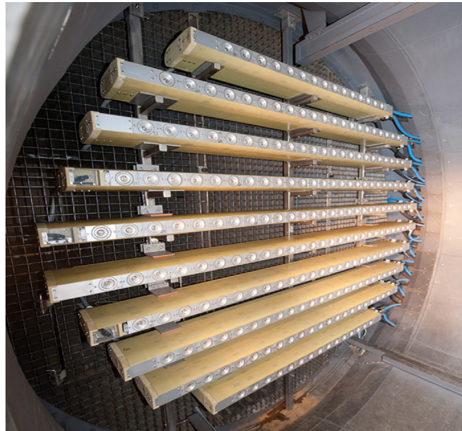
Figure 32.—Spray bars mounted in PSL-3 inlet plenum.
