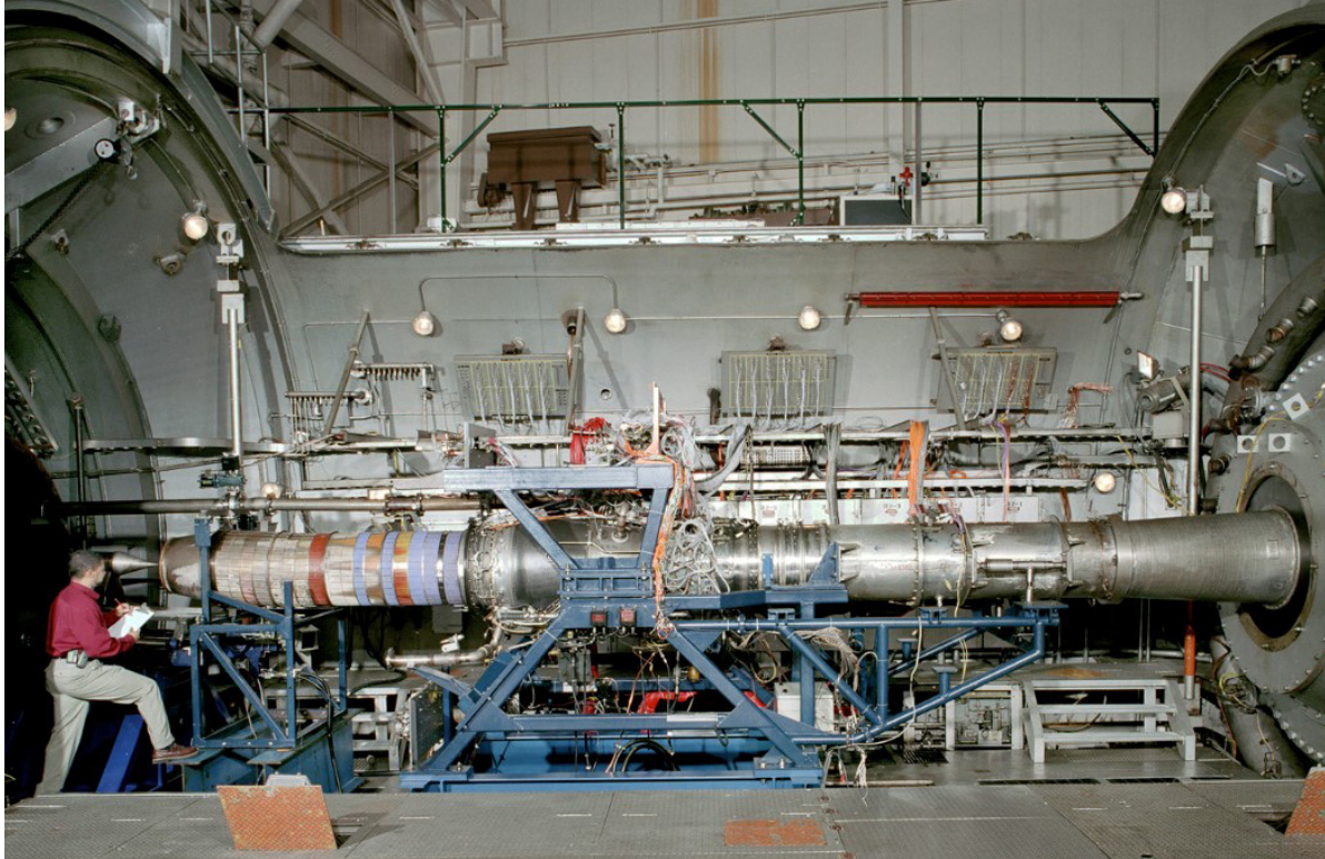
Figure 42.—Engine operability and stall resistance test.
