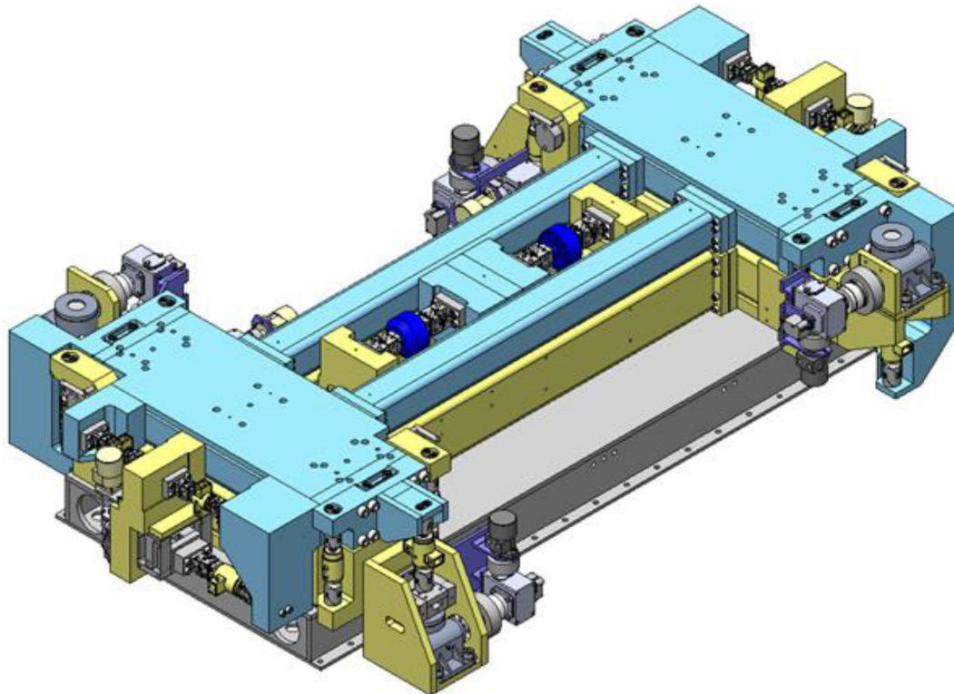
Figure 17.—Isometric view of PSL Ormond three-dimensional thrust measurement system.
