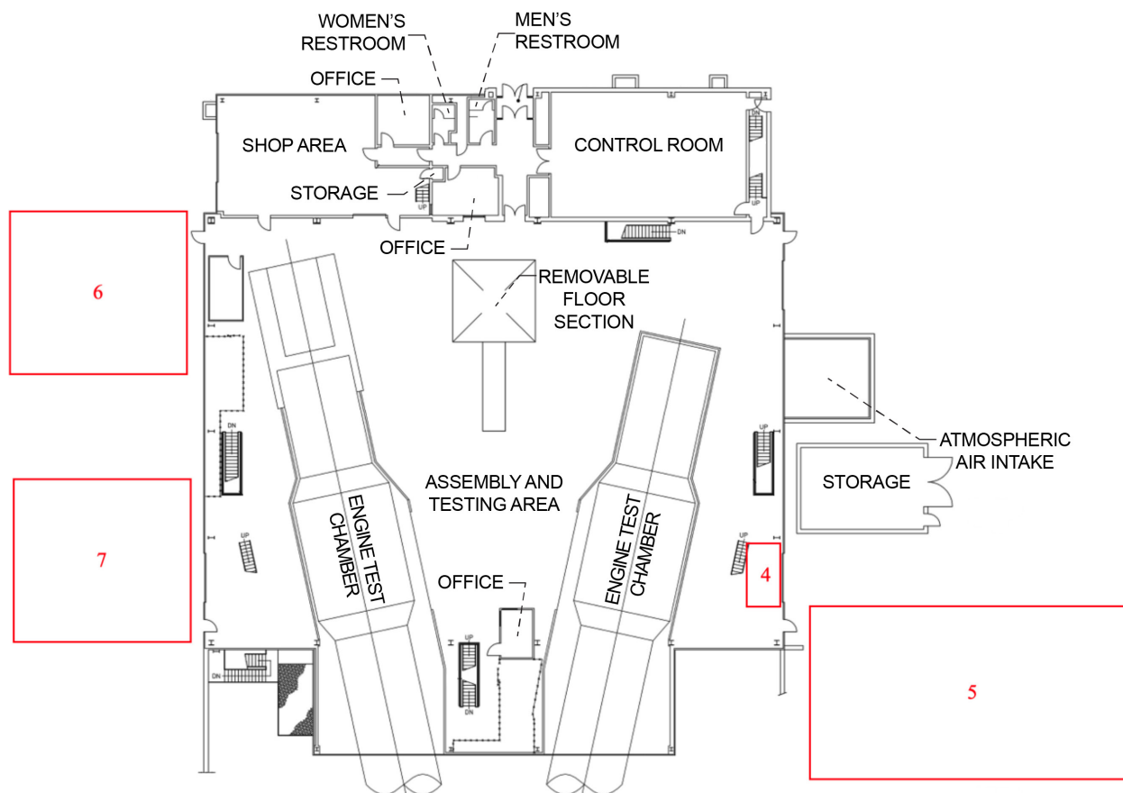
Figure 13.—Test-cell-level PSL customer support equipment areas.
