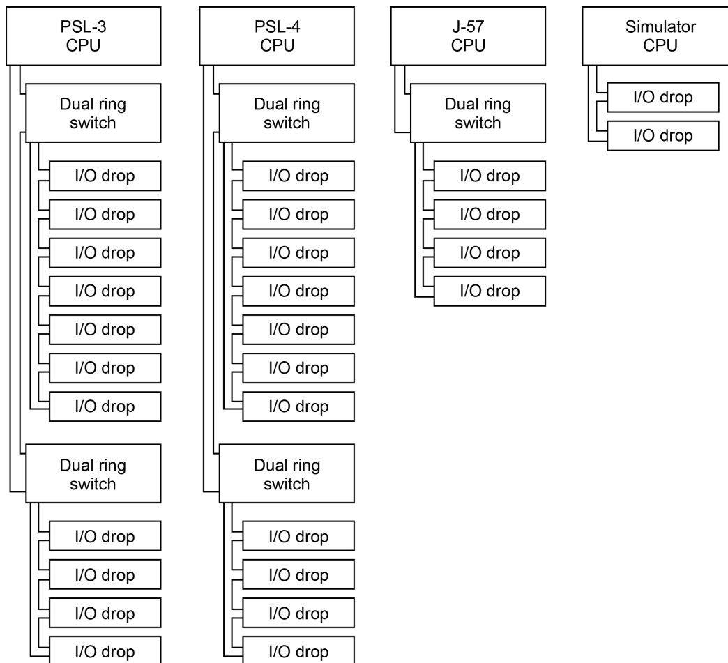
Figure 29.—Test cell PLC control system input/output (I/O).
