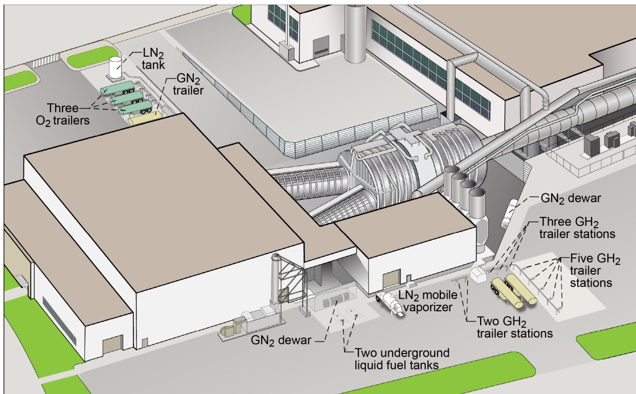
Figure 16.—Location of PSL propellant supplies.
