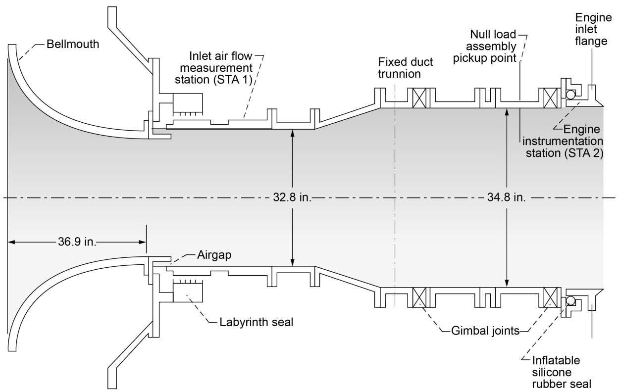
Figure 21.—Typical inlet ducting arrangement.
