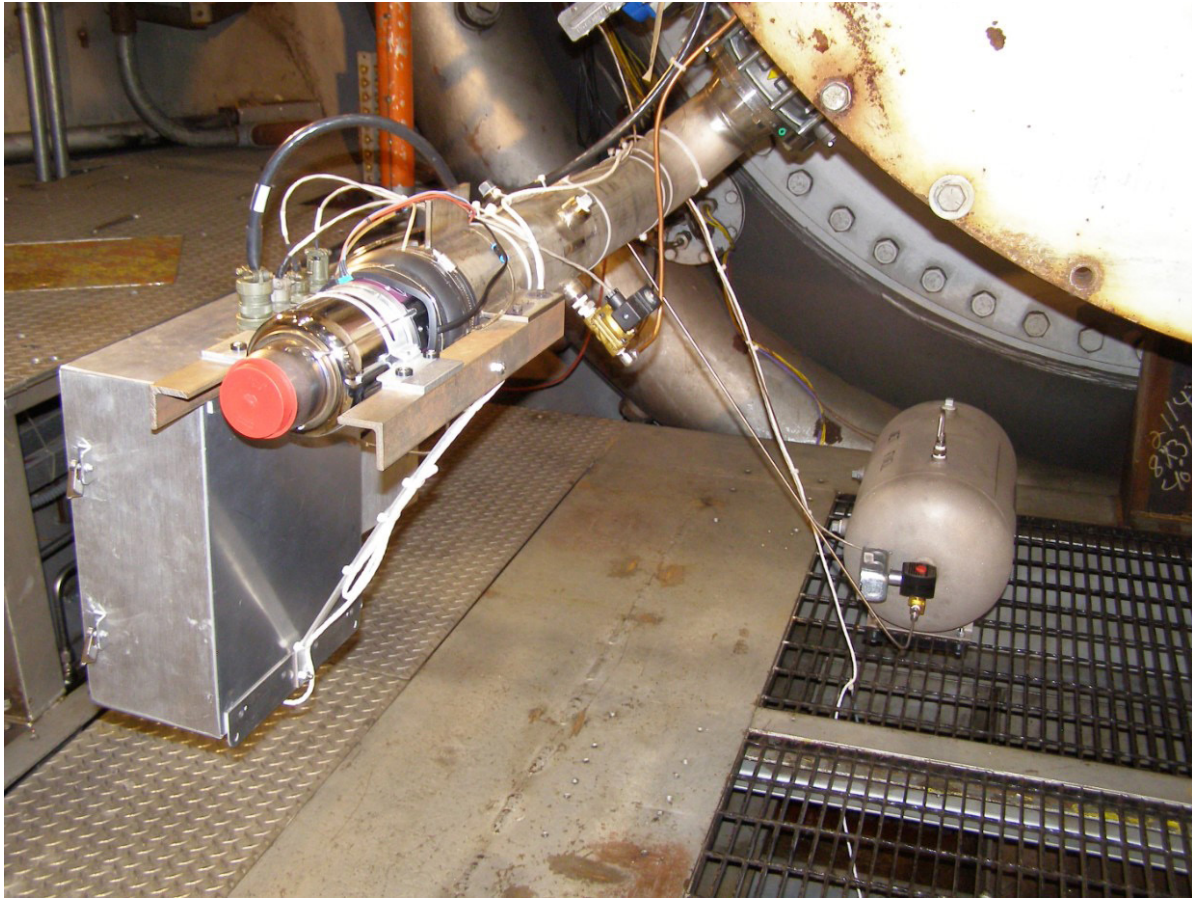
Figure 44.—Unmanned aerial vehicle/missile engine test.
