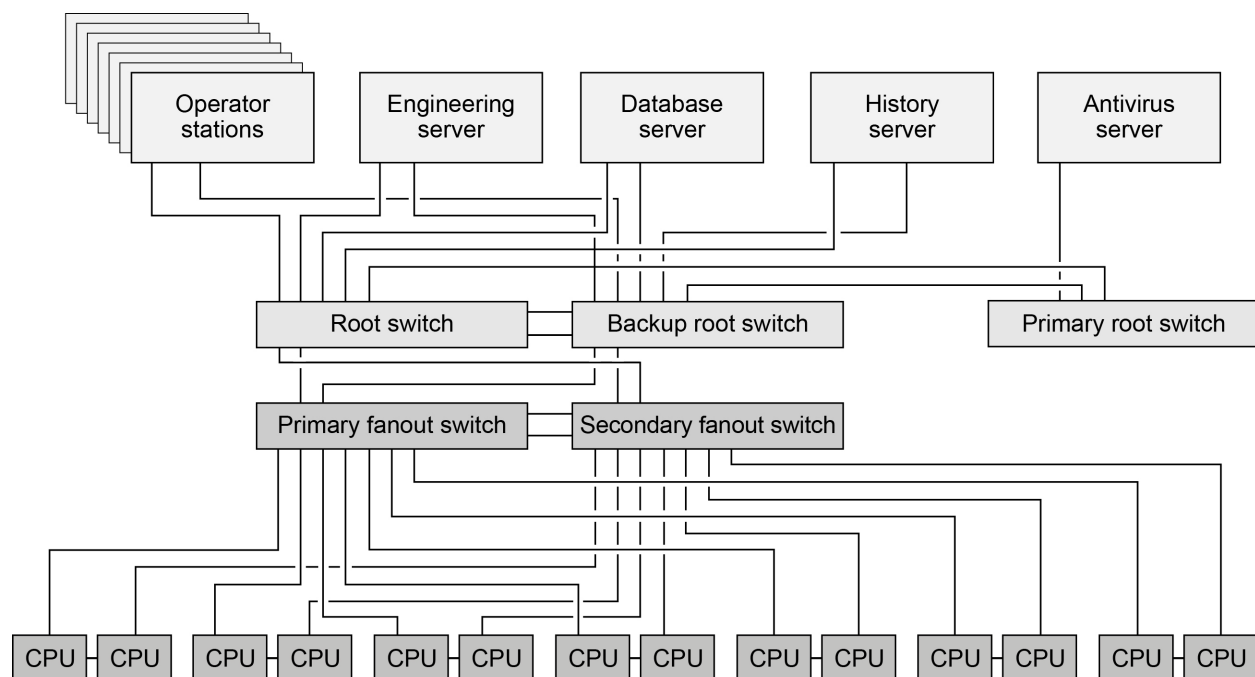
Figure 26.—Facility Ovation™ (Emerson Electric Co.) DCS network.
