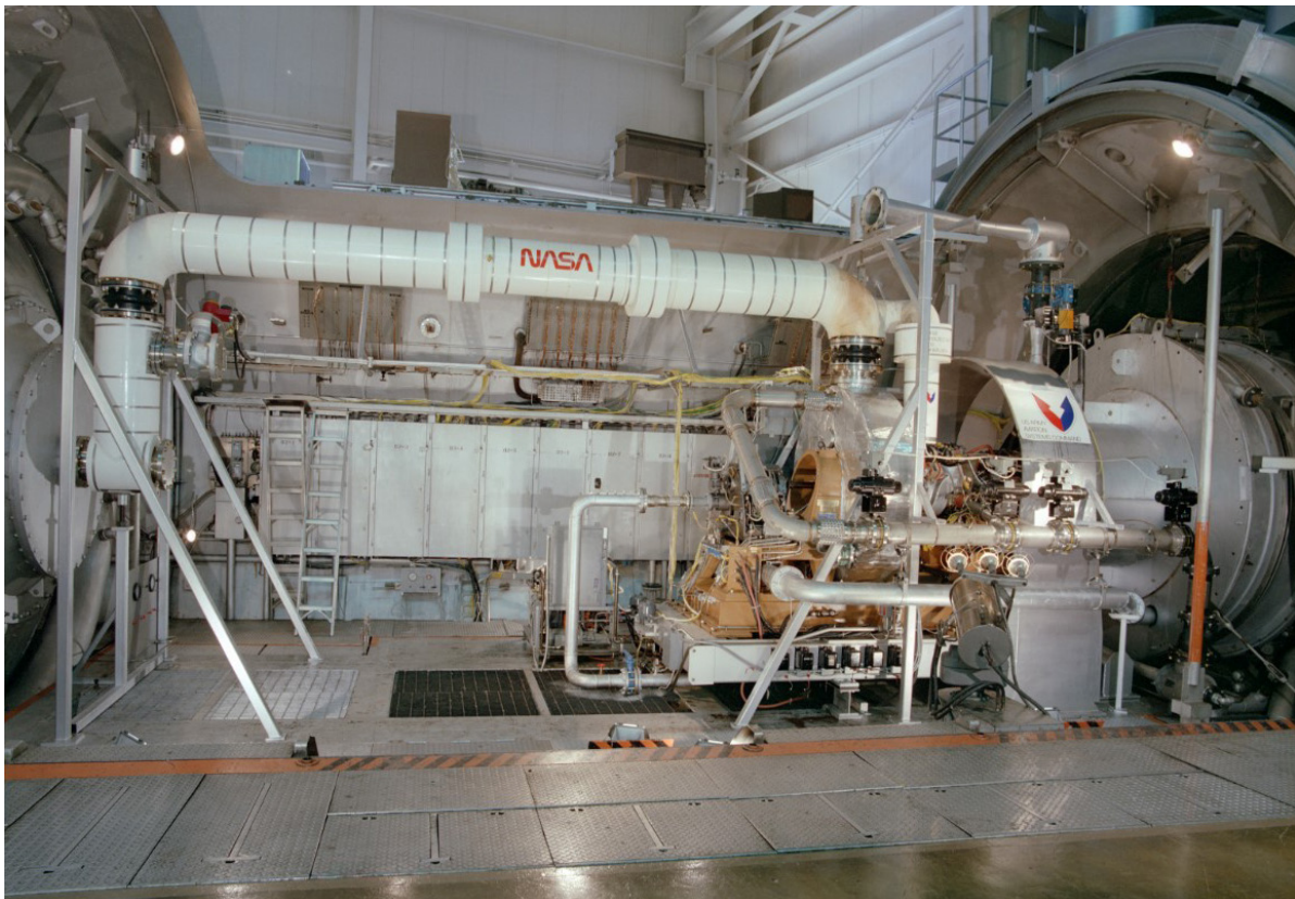
Figure 43.—Helicopter turboshaft engine test.
