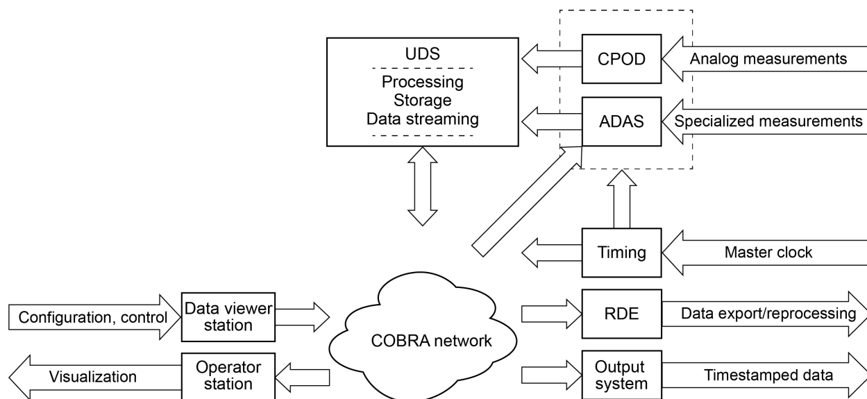
Figure 35.—COBRA data system. Universal data server, UDS; control pod, CPOD; auxiliary data acquisition system, ADAS; reprocessing data export, RDE.
