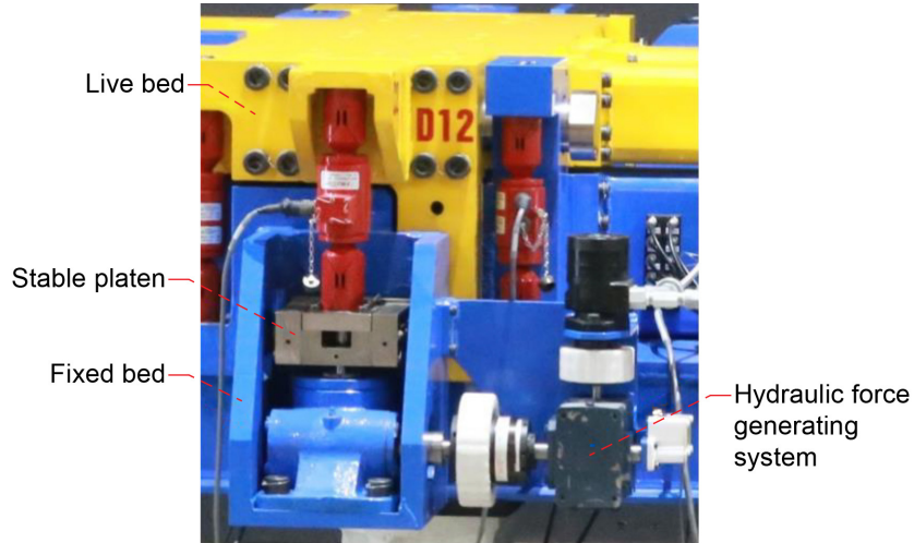
Figure 19.—Annotated view of structure connecting fixed bed to live bed.
