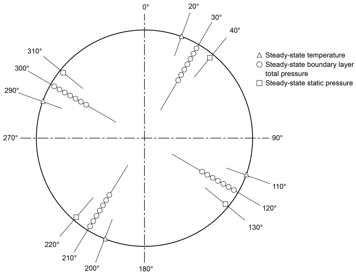
Figure 22.—Typical steady-state airflow measurement instrumentation at Station 1.
