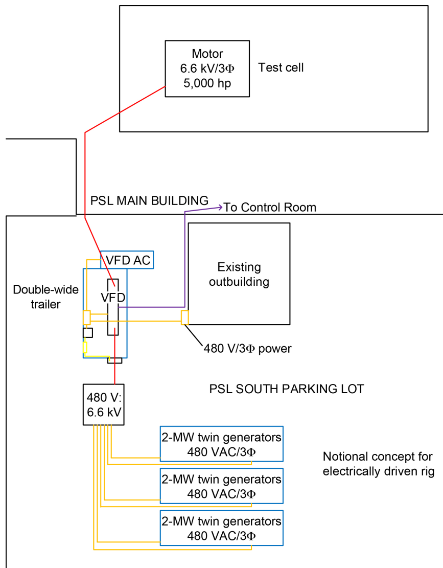
Figure 45.—Electrically driven rig test.
