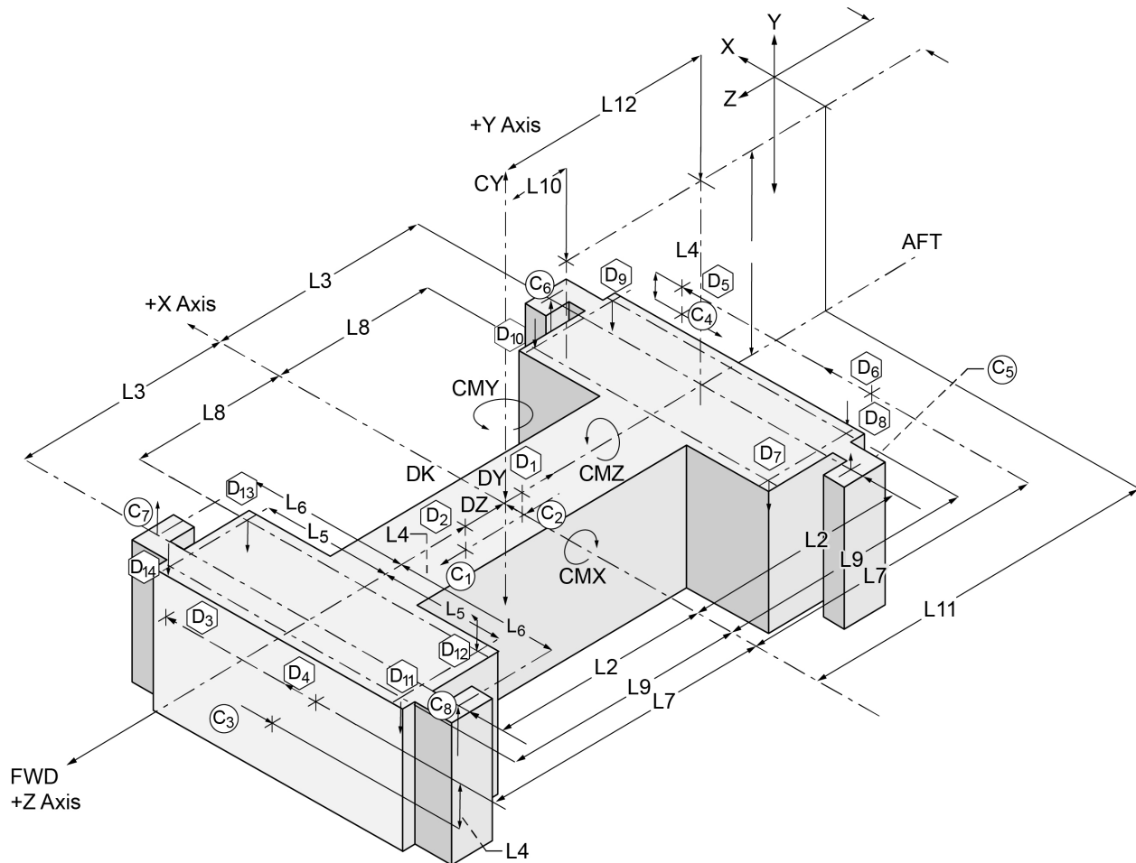
Figure 20.—Schematic of a typical Ormond three-dimensional thrust stand used in PSL.
