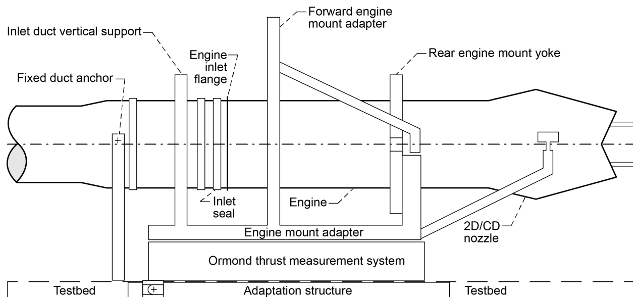
Figure 18.—Position of engine equipped with two-dimensional converging/diverging (2D/CD) nozzle in relation to Ormond multi-axis thrust stand.
