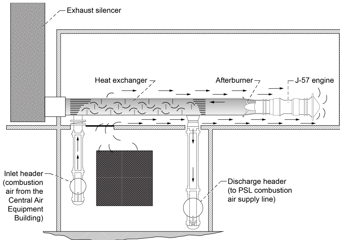
Figure 15.—Combustion air heater system.
