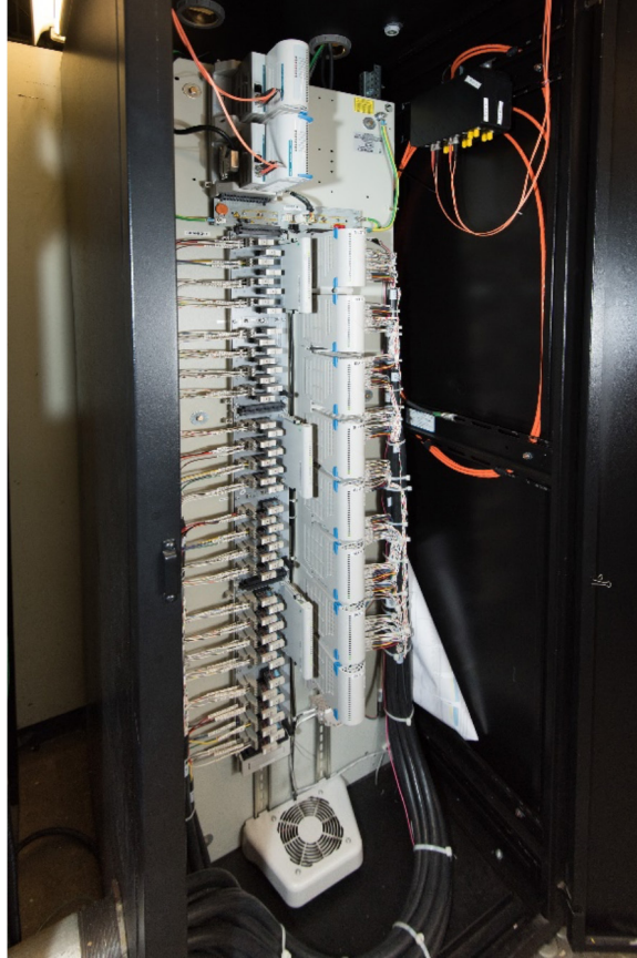
Figure 27.—Facility Ovation™ (Emerson Electric Co.) DCS typical input/output modules.
