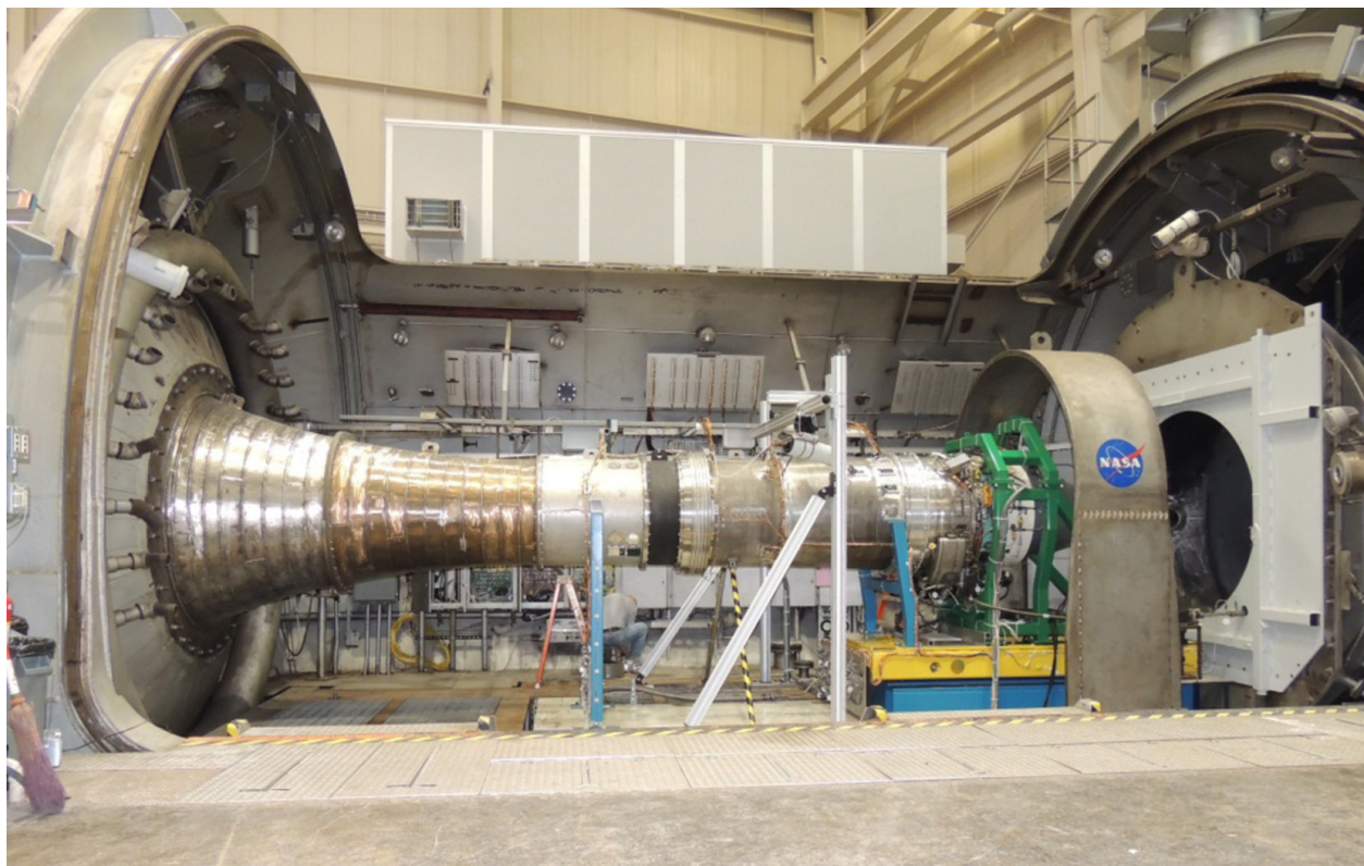
Figure 39.—Honeywell ALF502-R5 (serial number LF01) engine test.
