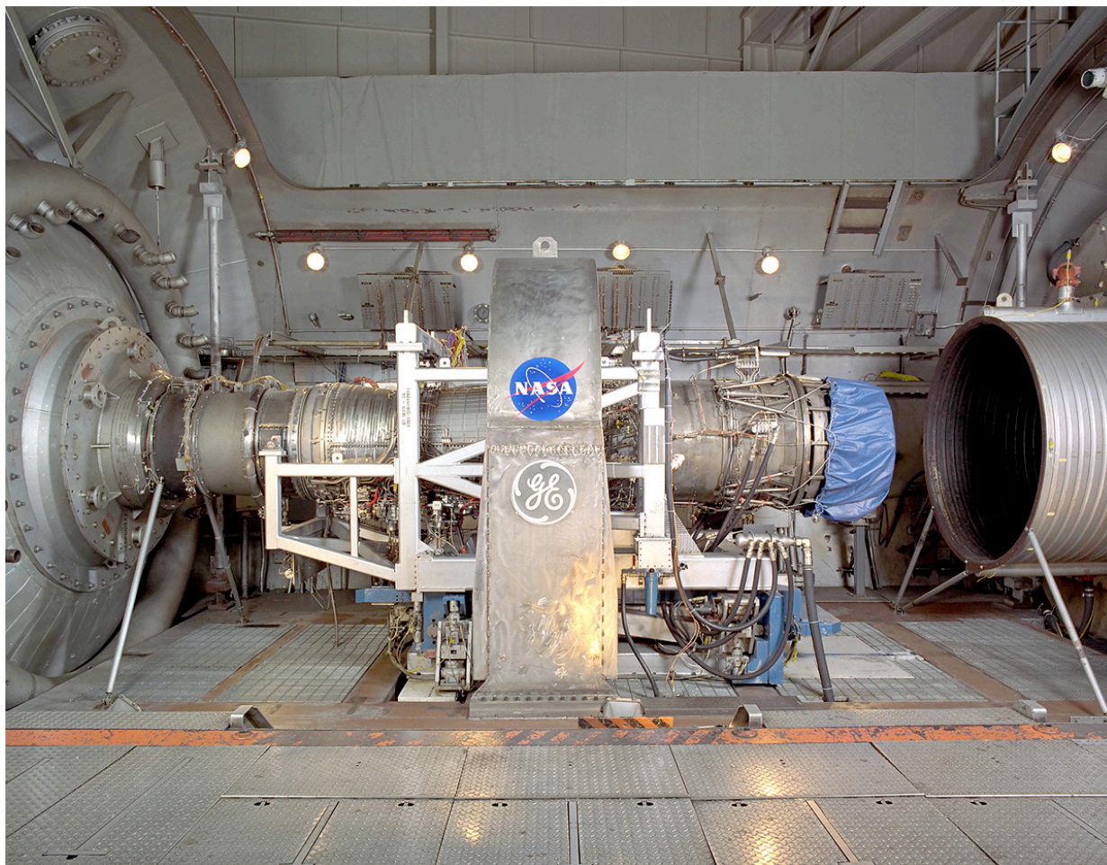
Figure 41.—Military fighter engine test.
