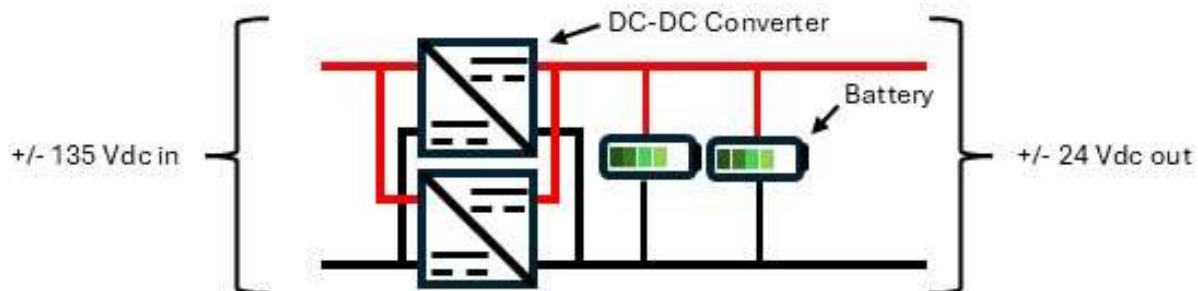
Figure 6. Wing power subsystem.
