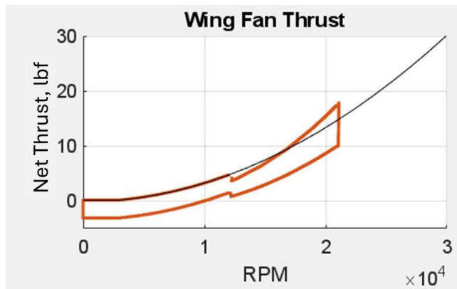
Figure 10. Wingfan thrust vs speed plot. The black curve comes from wind tunnel testing [7], the orange represents two cases: upper is zero velocity (no drag) and lower is nonzero velocity (includes drag). Above about 12,000 rpm is the T-MATS model, below 12,000 rpm is the static model.
