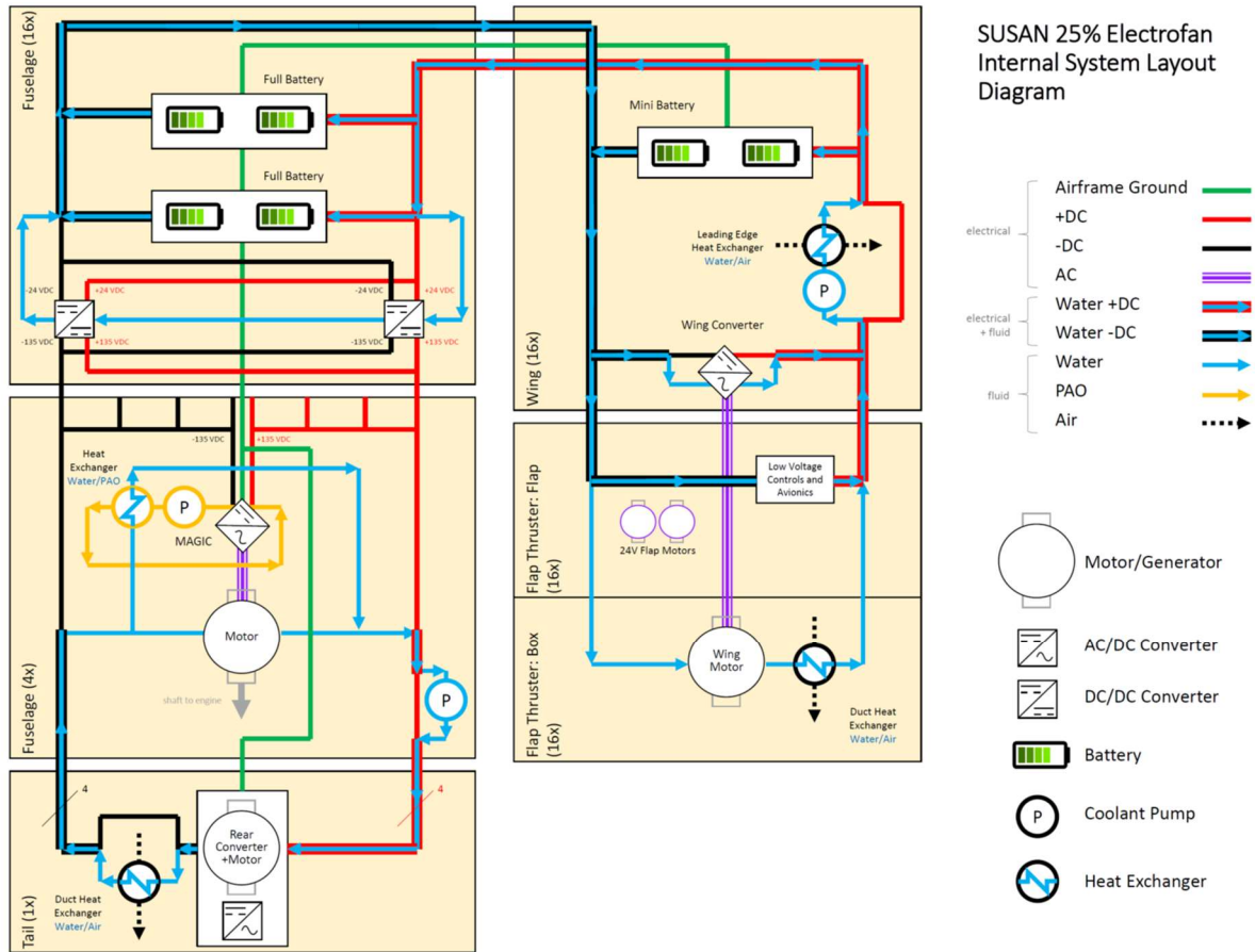
Figure 9. Quarter-scale distributed propulsion thermal management system diagram.
