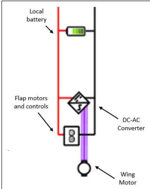
Figure 7. Wing electric engine and control subsystem.
