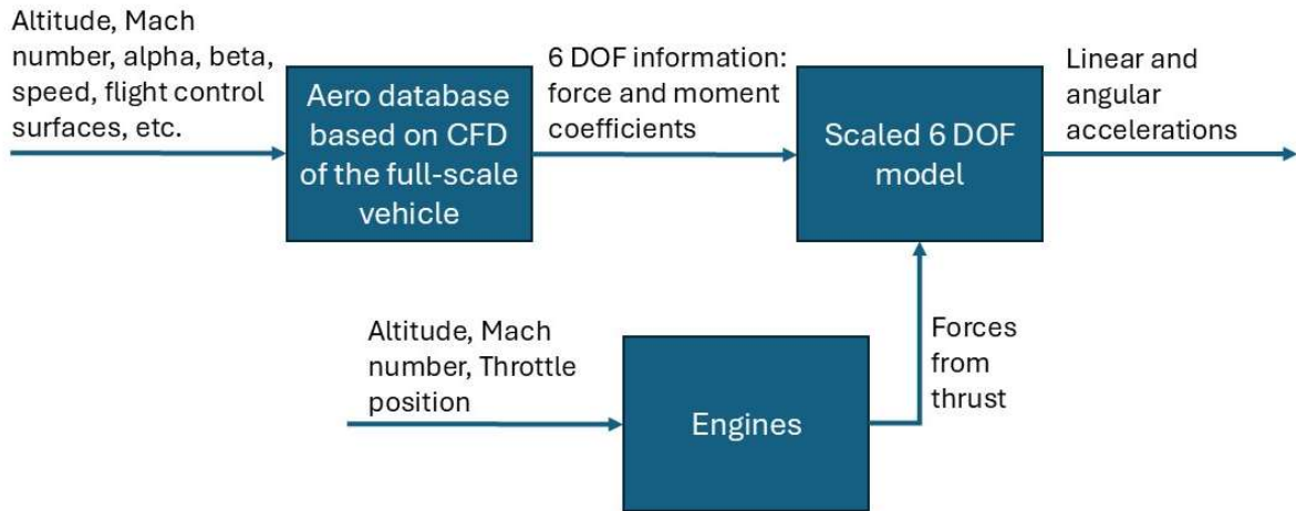
Figure 4. Simplified block diagram of the model implementation.
