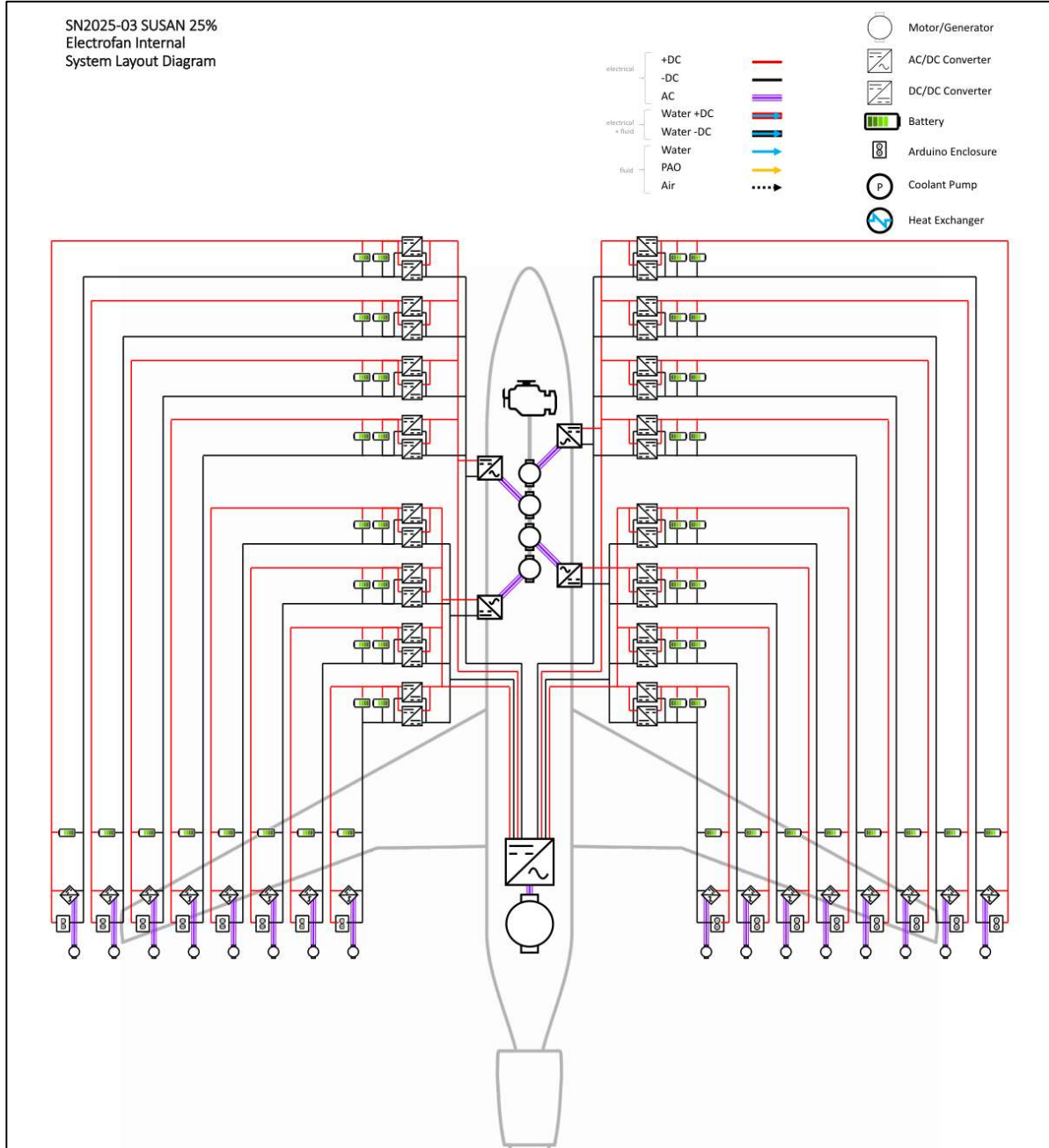
Figure 8. Quarter-scale distributed propulsion electrical power system.
