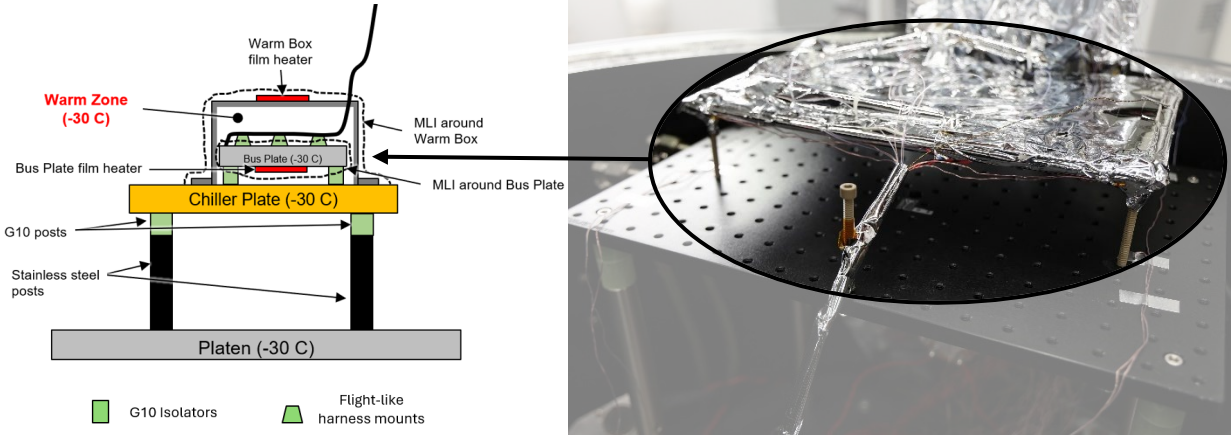
Figure 4: (left) Warm zone configuration. (right) As-built bus plate mounting showing Polyether Ether Ketone (PEEK) bolts.
