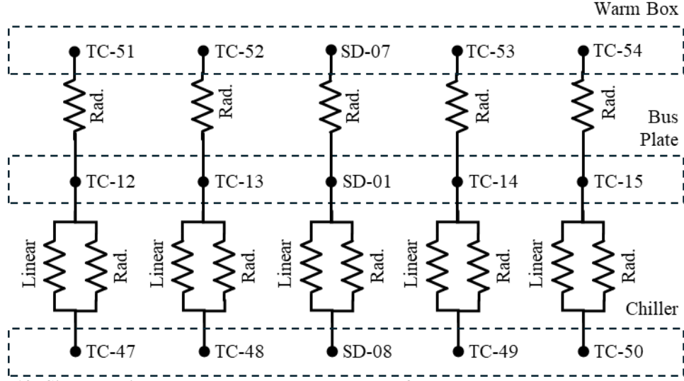
Figure 12: Simple resistor network to evaluate the heat flow error due to temperature uncertainty
