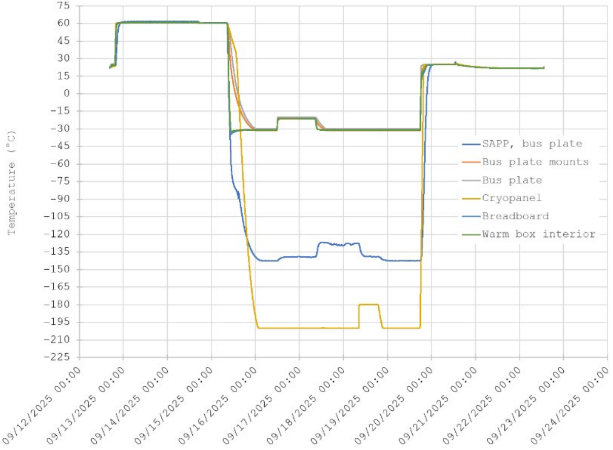
Figure 9: As-Run Test Profile
