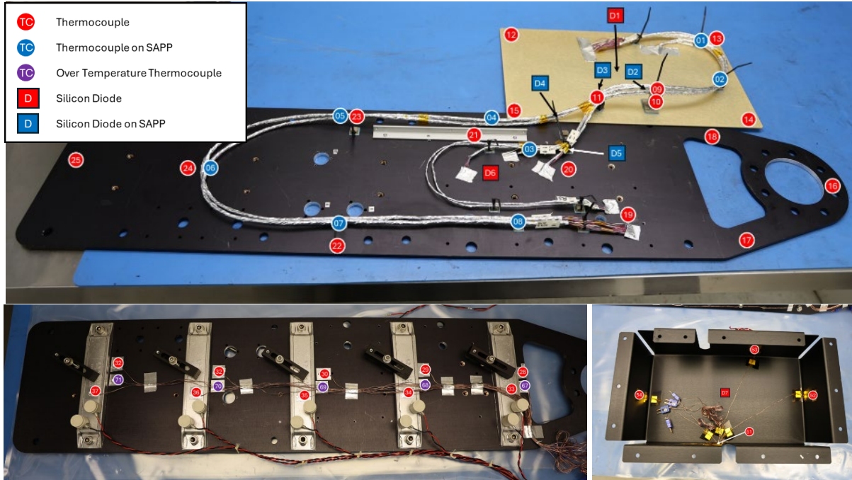
Figure 5: (upper) Test sensors on Cryopanel (cold zone) front, Bus Plate, and SAPP RRU. (bottom left) Test sensors on Cryopanel rear. (bottom right) Test sensors on warm box.
