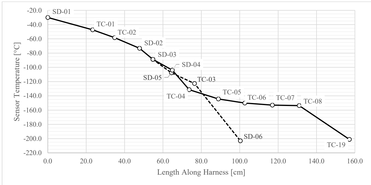
Figure 10: Balance #1 temperature gradient in the SAPP harness. The dashed line ( - - ) notes the main fork where the SAPP exits the warm box.
