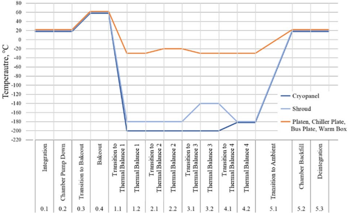
Figure 8: Test Profile
