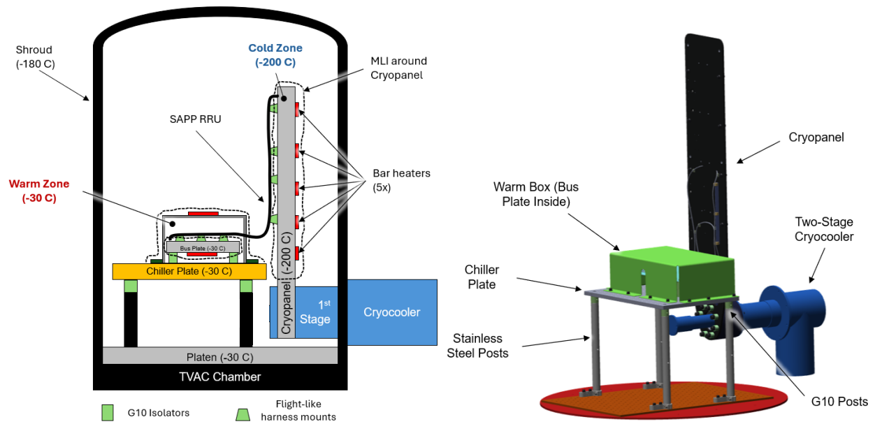
Figure 2: (left) Test block diagram. (right) Model of the test configuration.
