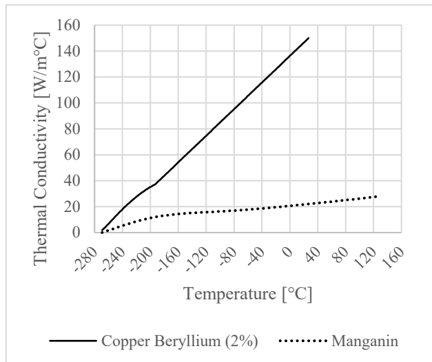
Figure 11: SAPP Harness Material Thermal Conductivities [2]
