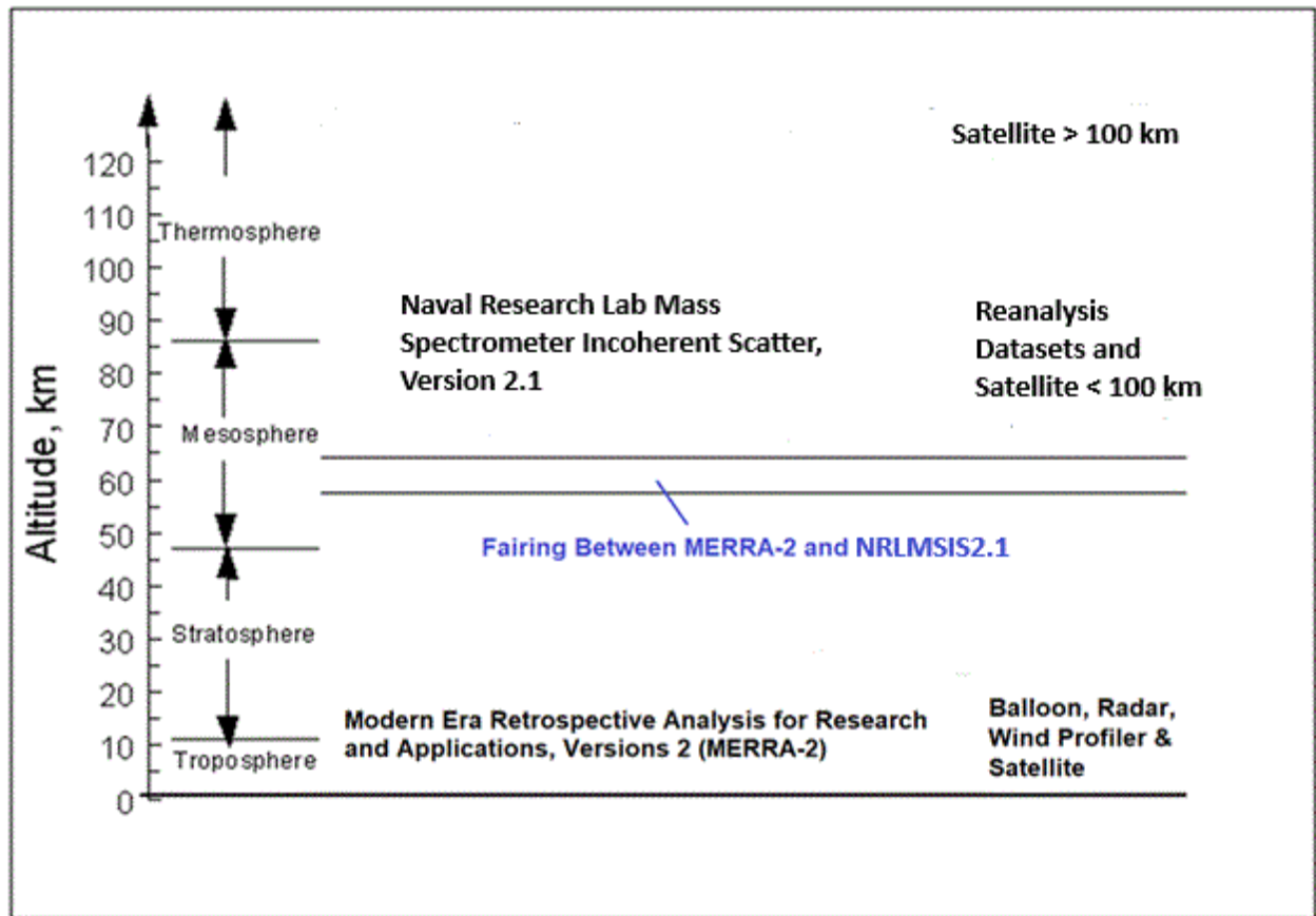
Figure 7. Schematic summary of the atmospheric regions in the Earth-GRAM program, sources for the model, and data on which the mean monthly Earth-GRAM values are based when NRLMSIS 2.1 and MERRA-2 are selected.
