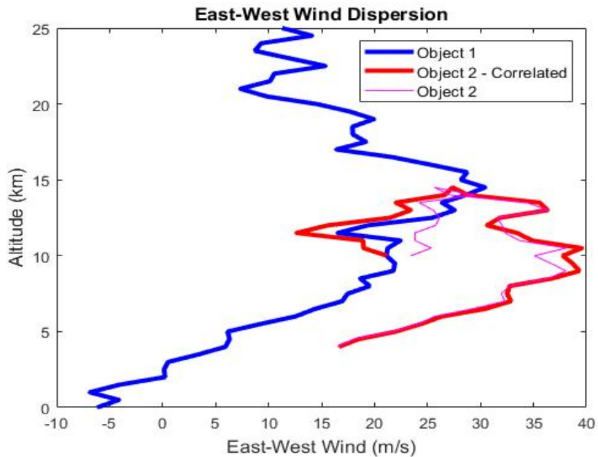
Figure 19. East-West Wind Dispersions Generated from Two Trajectory Objects Generated by Earth-GRAM.
