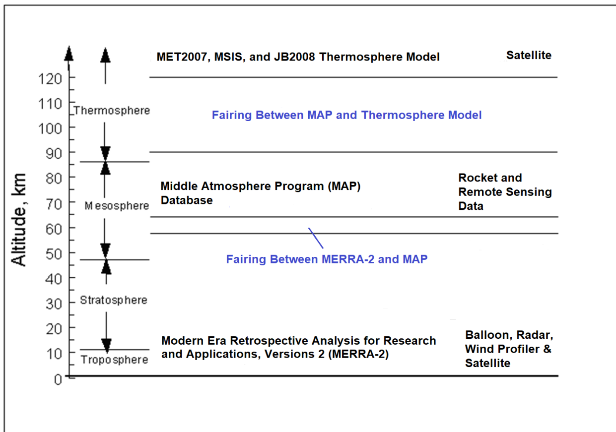
Figure 1. Schematic summary of the atmospheric regions in the Earth-GRAM program, sources for the model, and data on which the mean monthly Earth-GRAM values are based.
