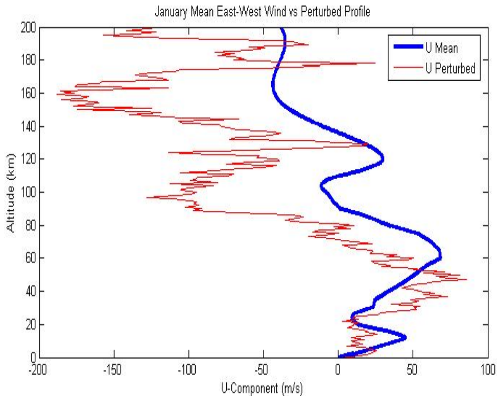
Figure 12. January Mean and Dispersed Profile of East-West Wind.
