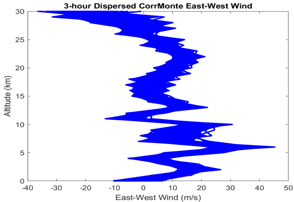
Figure 15. 1000 3-hour East-West Wind Dispersions about a Dispersed Profile Generated by CorrMonte.
