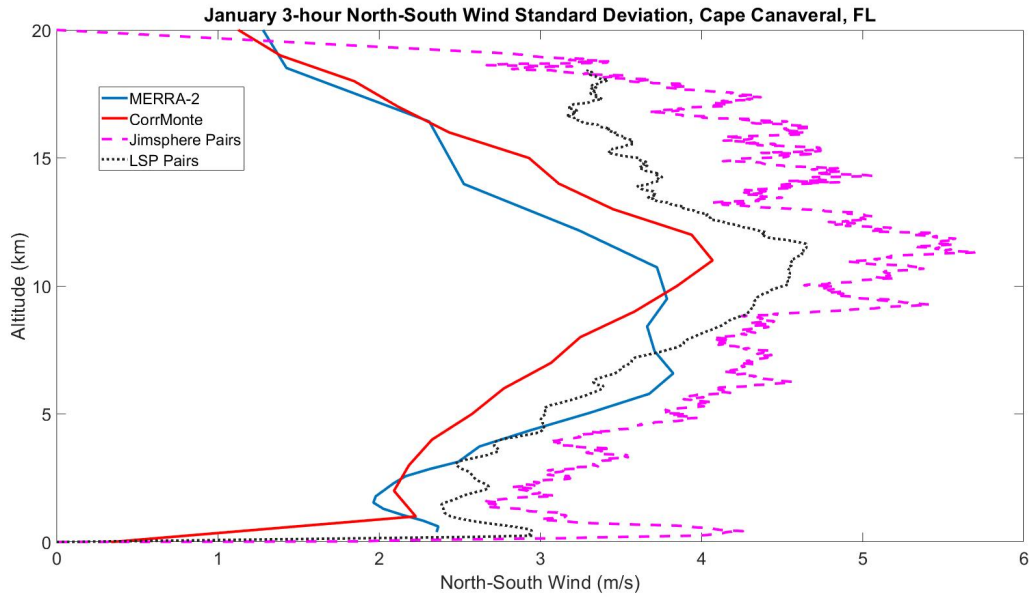
Figure 9. January 3-hour Comparison of North-South Wind Standard Deviation.
