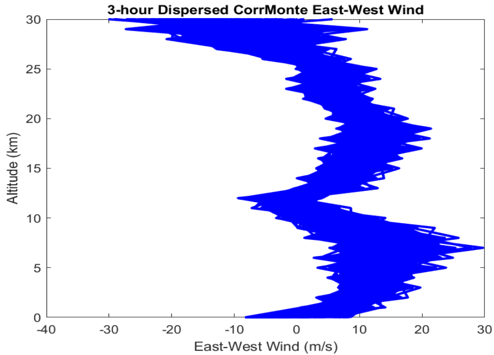
Figure 16. 1000 3-hour East-West Wind Dispersions about the Mean Generated by CorrMonte.
