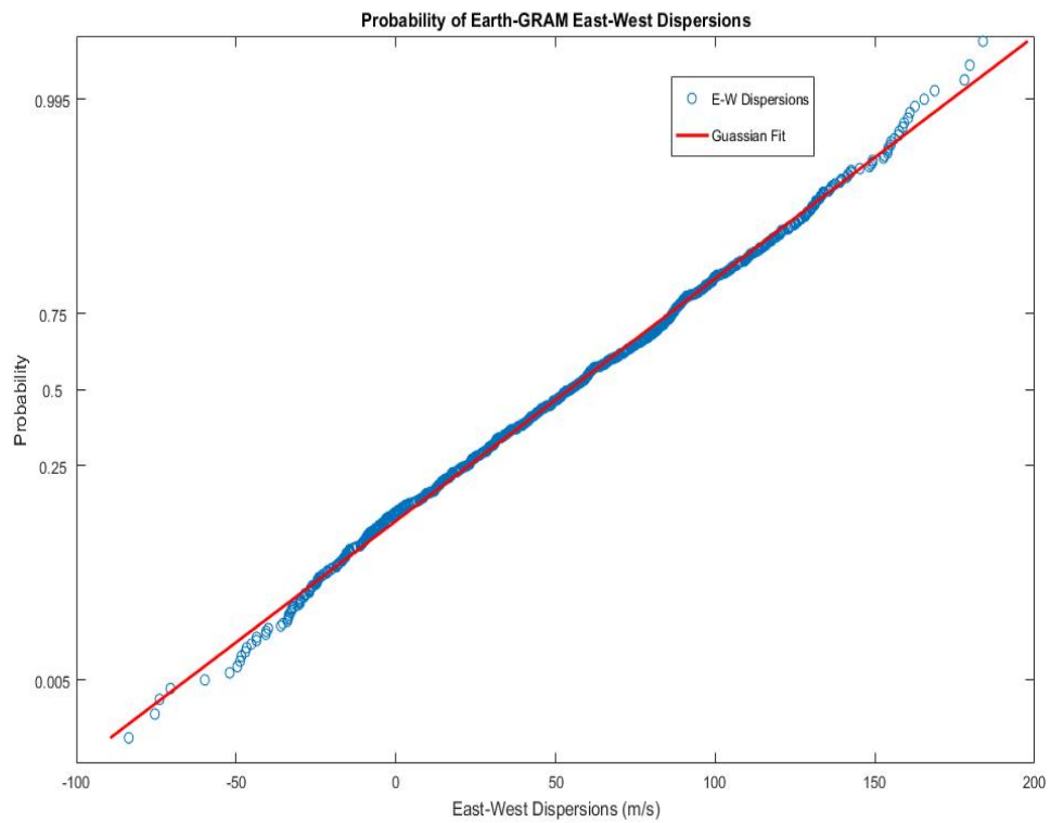
Figure 14. Cumulative Probability of East-West Wind Dispersion with a Gaussian distribution fit.
