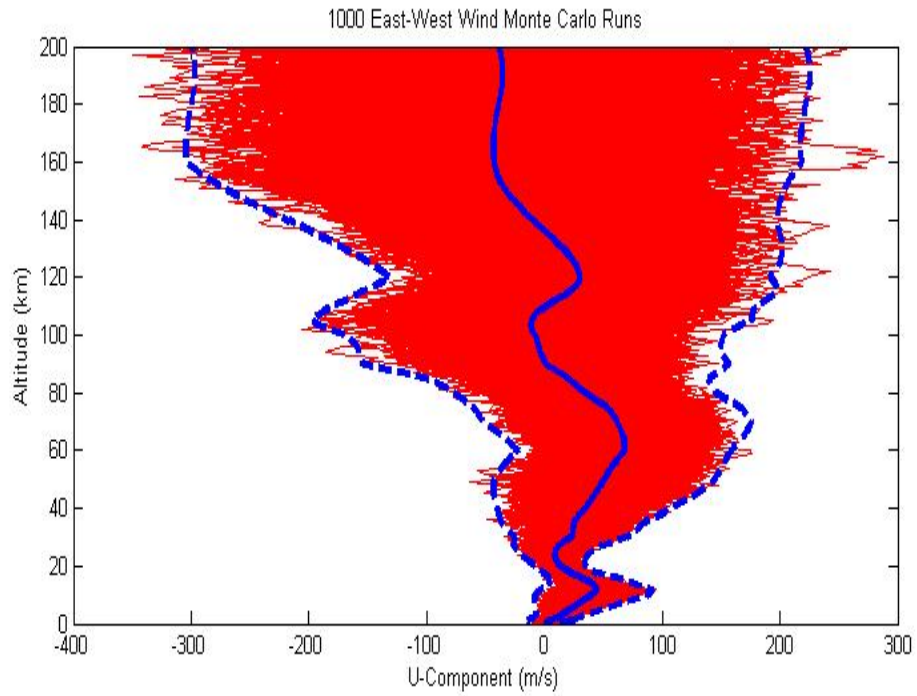
Figure 13. 1000 January East-West Wind Monte Carlo Dispersions with Mean and 3-sigma.
