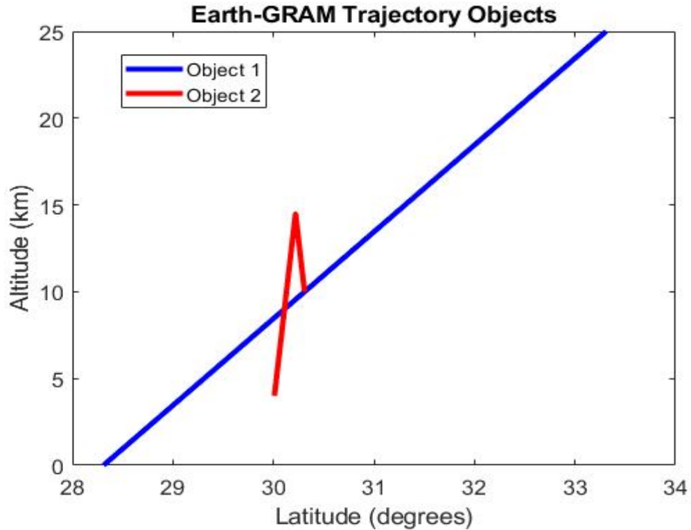
Figure 18. Positional Information Regarding Two Trajectory Objects Generated by Earth-GRAM.
