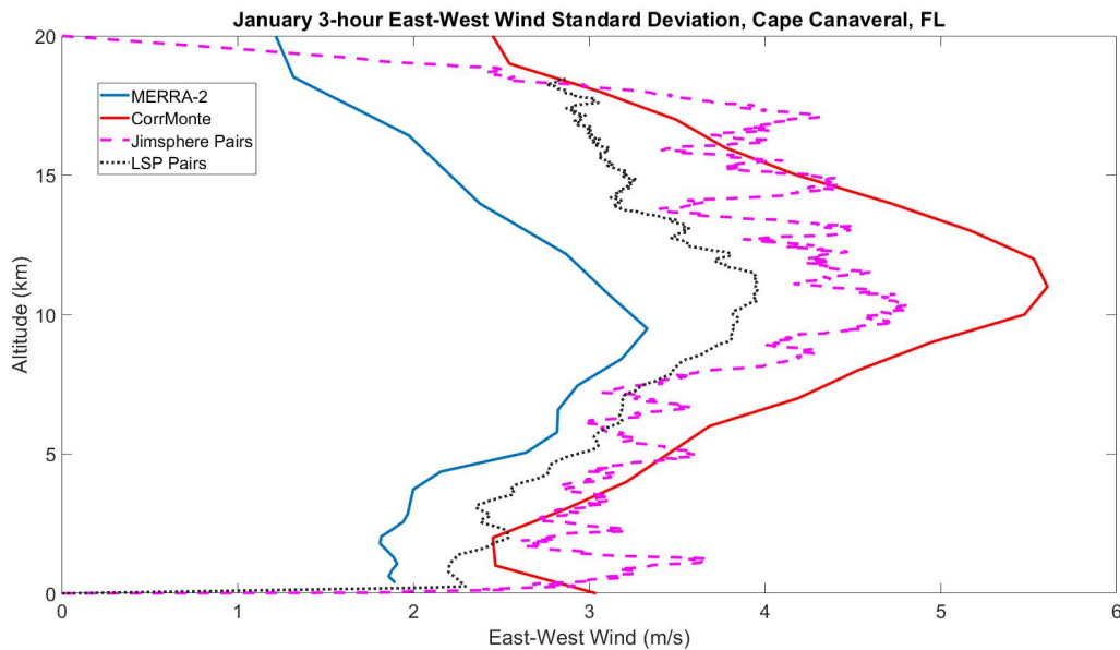
Figure 8. January 3-hour Comparison of East-West Wind Standard Deviation.
