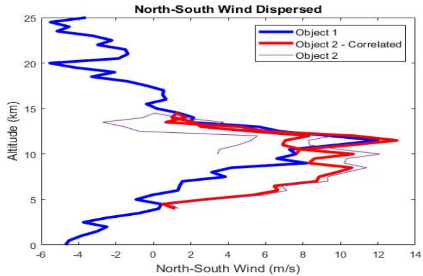
Figure 20. North-South Wind Dispersions Generated from Two Trajectory Objects Generated by Earth-GRAM.
