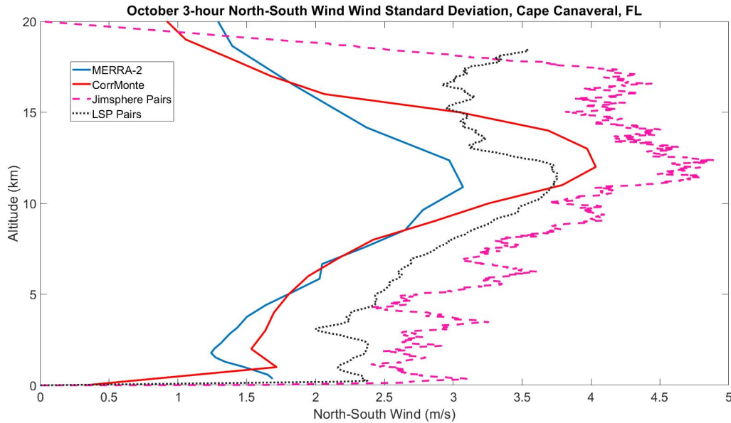
Figure 11. October 3-hour Comparison of North-South Wind Standard Deviation.
