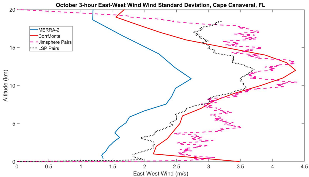
Figure 10. October 3-hour Comparison of Earth-West Wind Standard Deviation.
