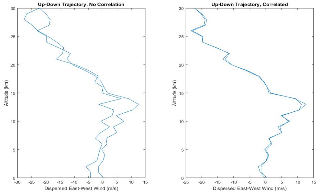
Figure 17. East-West Wind Dispersions Generated by Earth-GRAM (left) and the Ballistic Trajectory Feature (right).
