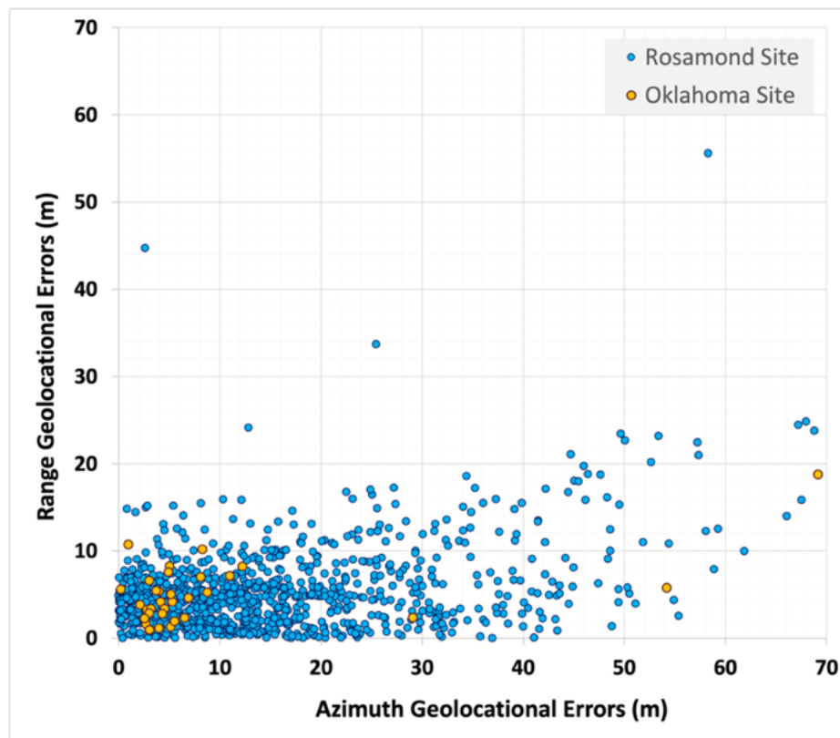
Figure 5. Geolocation errors in range and azimuth directions derived from corner reflectors at Rosamond and Oklahoma sites.
