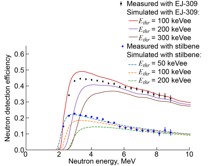
Figure 4.— 252 Cf Neutron detection efficiency of large 50- by 75-mm EJ-309 detector and small 25- by 25-mm stilbene detector at different thresholds, E_{thr} .
