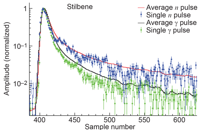
Figure 6.— ^{252}\text{Cf} neutron and \gamma -ray signatures recorded using stilbene and the ADC. Time (ns) = 2 \times \text{sample number} . Note: The average pulse is created adding 10,000 single pulses and normalized the peak value to 1. So, a given single pulse can deviate from the average.
