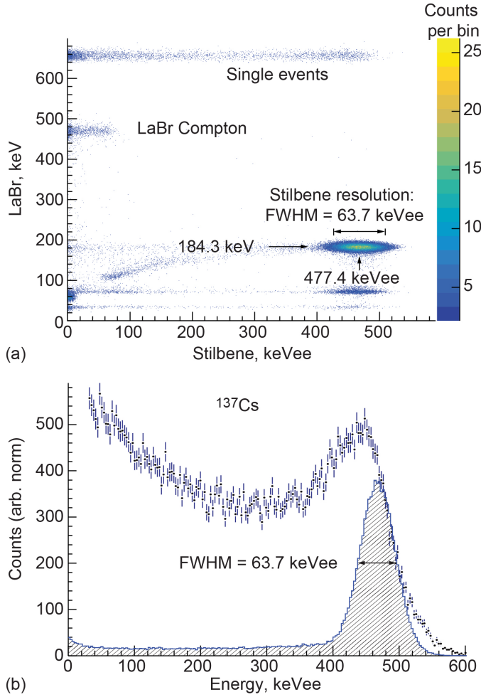
Figure 1.—LaBr and stilbene coincidence spectra for the case of 180^\circ Compton backscattering. (a) LaBr versus stilbene two-dimensional (2-D) spectra. FWHM is the full width at half maximum. (b) Comparison of ^{137}\text{Cs} single-hit spectrum and the coincidence spectrum (striped area) that is created by projecting the 2-D spectrum around 183 \pm 10 keV energy bins.
