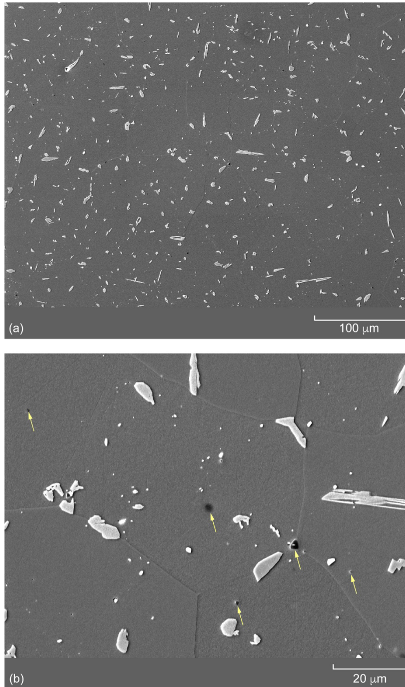
Figure 1.—SEM micrographs at (a) low- and (b) high-magnification showing the parent phase (grey) and secondary phases (light grey) in the studied alloy. Pores are visible in the microstructure, as indicated with arrows.
