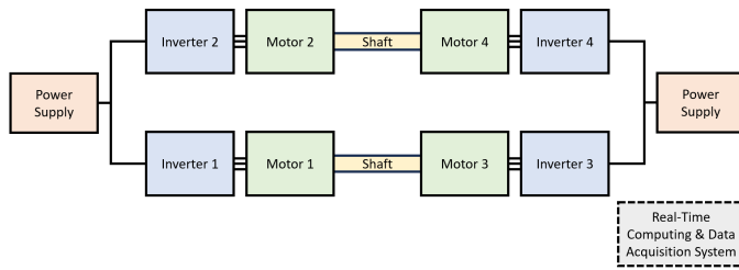
Figure 2. Architecture and naming convention for the HyPER testbed
