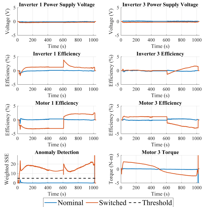
Figure 8. Health parameter estimates when test data were organized correctly vs. when switched across shaft systems before being sent to the Kalman filter.
