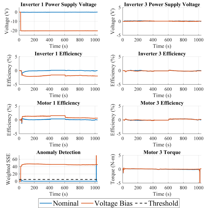
Figure 7. Health parameter estimates and calculated anomaly detection signals for nominal and induced voltage anomaly tests.
