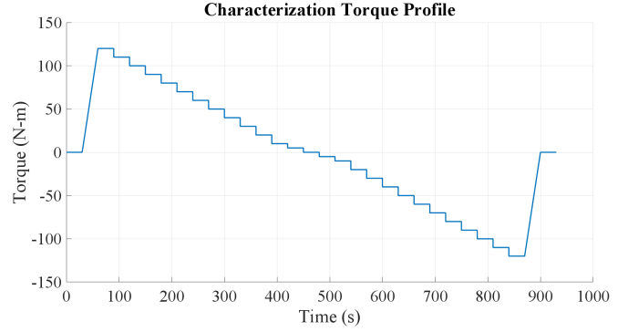
Figure 4. Torque command profile for the ‘torque mode’ motor during characterization tests.
