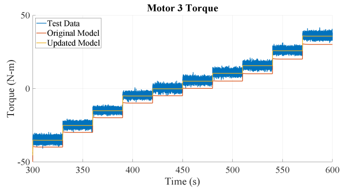
Figure 5. Comparison of previous and updated HyPER models when real test data were used as model inputs.
