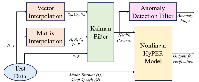
Figure 6. Digital twin block diagram showing the flow of information throughout the Kalman filter, the nonlinear HyPER model, and the anomaly detection filter.
