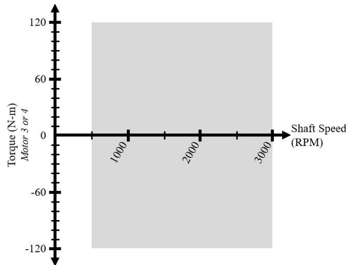
Figure 3. Operating envelope (shaded) exercised during characterization testing.
