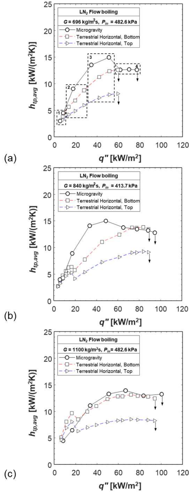
Fig. 13 Effects of gravity on average heat transfer coefficient for near-saturated inlet and mass velocities of G = (a) 695, (b) 840, and (c) 1100 kg/m 2 s.
