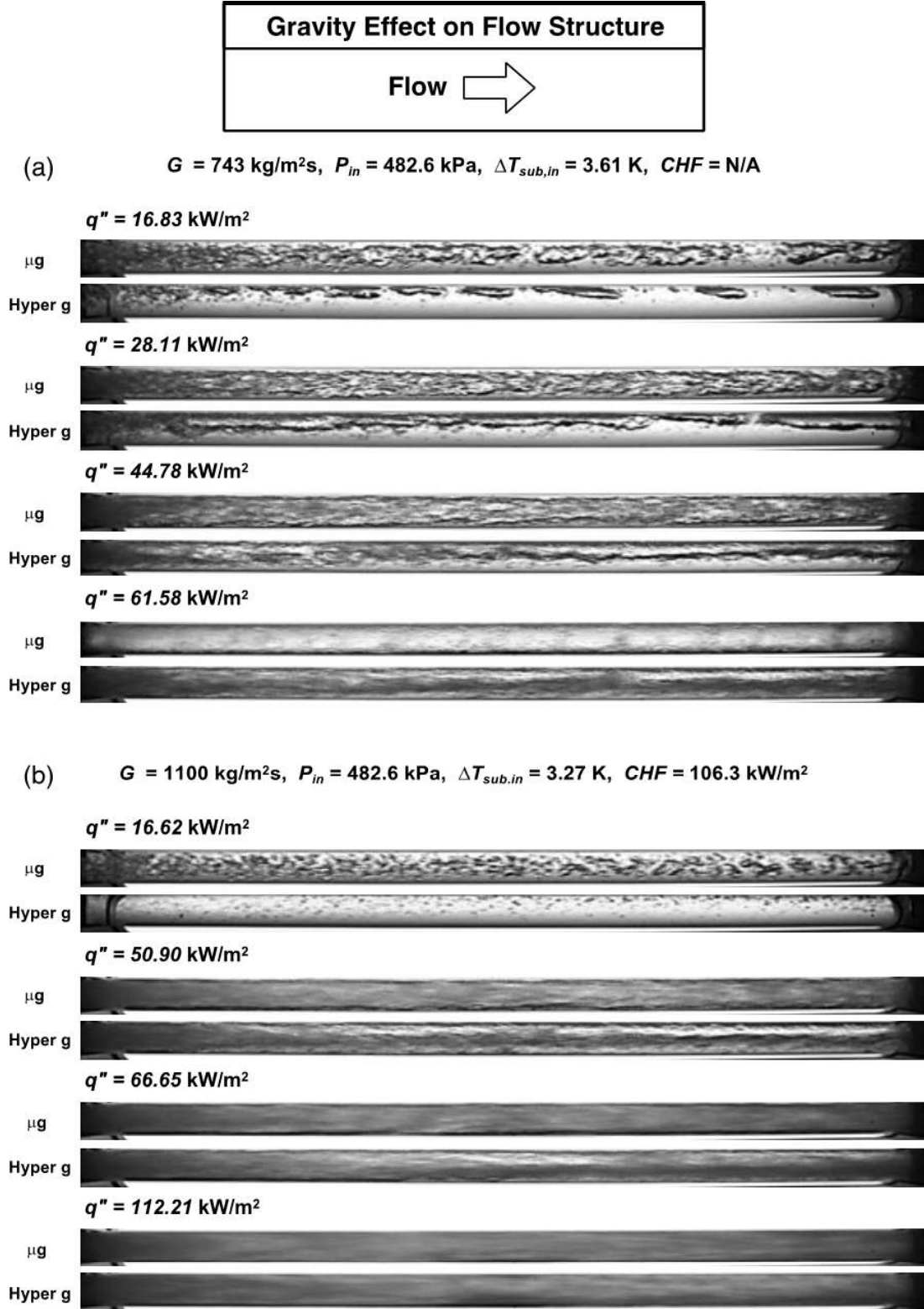
Fig. 6 Effects of gravity on two-phase flow structure for near-saturated inlet with (a) mass velocity of G = 743 \text{ kg/m}^2\text{s} and heat fluxes of q'' = 16.83, 28.11, 44.78 , and 61.58 \text{ kW/m}^2 , and (b) mass velocity of G = 1100 \text{ kg/m}^2\text{s} and heat fluxes of q'' = 16.62, 50.90, 66.65 , and 112.21 \text{ kW/m}^2 .
