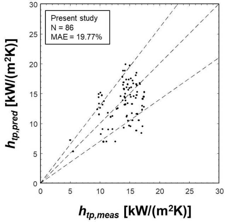
Fig. 16 Performance of new flow boiling HTC correlation against present measured microgravity HTC data.
