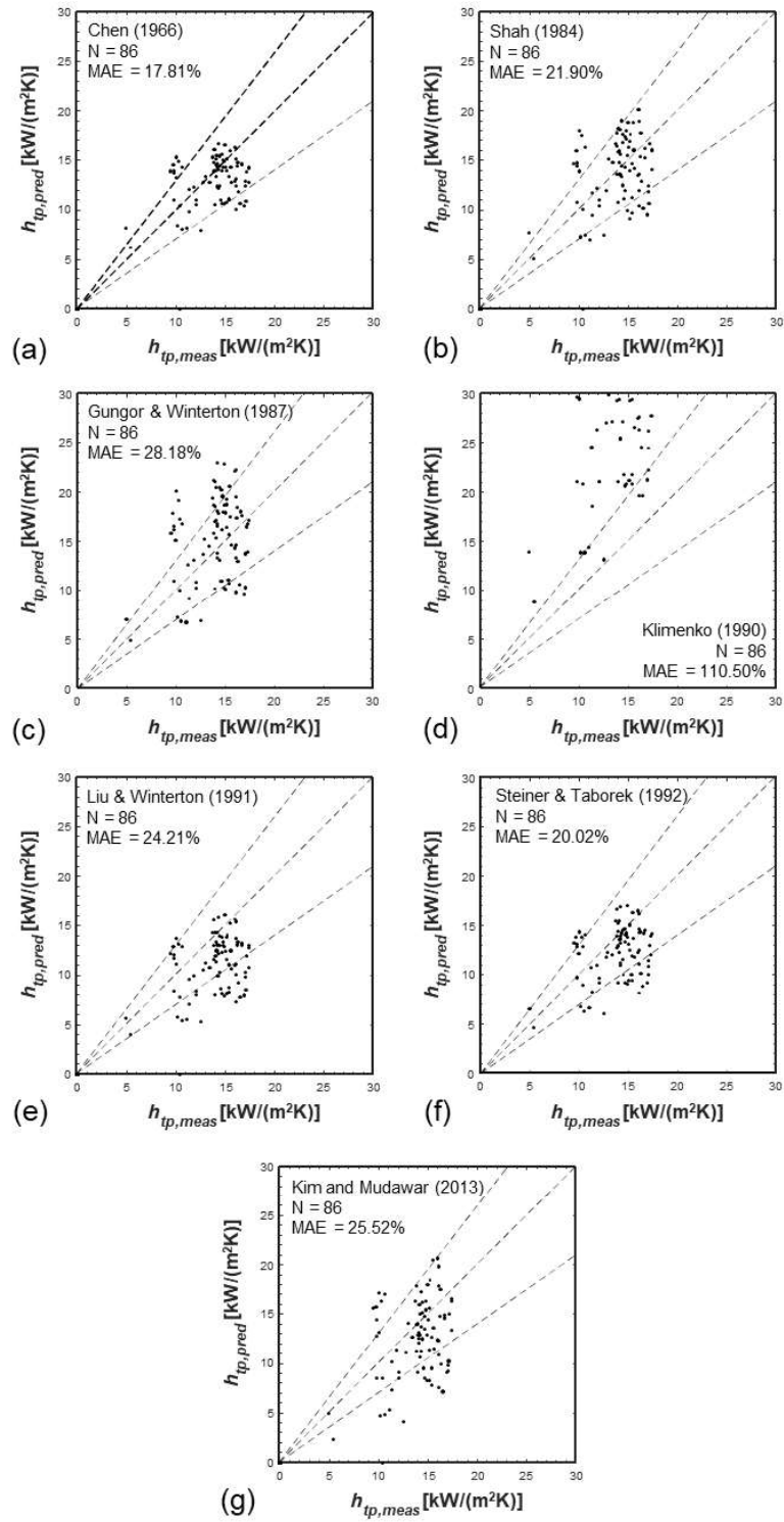
Fig. 14 Performance of seminal flow boiling HTC correlations against present measured microgravity HTC data.
