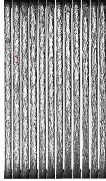
Fig. 4 Flow visualization image sequences for near-saturated inlet, mass velocity of G = 400 \text{ kg/m}^2\text{s} , and q'' = (a) 2.76 \text{ kW/m}^2 , (b) 4.21 \text{ kW/m}^2 , (c) 5.59 \text{ kW/m}^2 , and (d) 11.26 \text{ kW/m}^2 .
