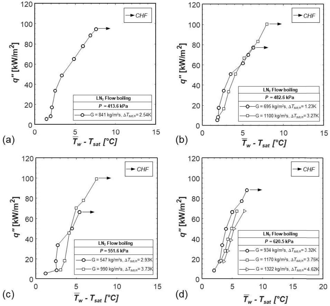
Fig. 9 Microgravity boiling curves for different operating conditions: (a) P_{in} = 413.6 kPa, G = 841 kg/m 2 s, (b) P_{in} = 482.6 kPa, G = 695 and 1100 kg/m 2 s, (c) P_{in} = 551.6 kPa, G = 547 and 990 kg/m 2 s, and (d) P_{in} = 620.5 kPa, G = 934 , 1170 , and 1322 kg/m 2 s.
