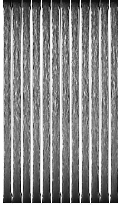
Fig. 5 Flow visualization image sequences for near-saturated inlet, mass velocity of G = 1300 \text{ kg/m}^2\text{s} , and q'' = (a) 17.53 \text{ kW/m}^2 , (b) 28.09 \text{ kW/m}^2 , (c) 38.73 \text{ kW/m}^2 , and (d) 50.02 \text{ kW/m}^2 .
