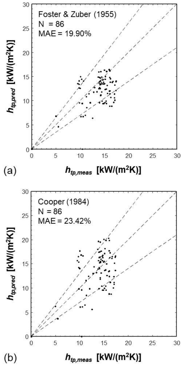
Fig. 15 Performance of seminal pool boiling HTC correlations against present measured microgravity HTC data.
