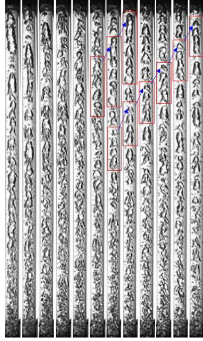
Fig. 4 Flow visualization image sequences for near-saturated inlet, mass velocity of G = 400 \text{ kg/m}^2\text{s} , and q'' = (a) 2.76 \text{ kW/m}^2 , (b) 4.21 \text{ kW/m}^2 , (c) 5.59 \text{ kW/m}^2 , and (d) 11.26 \text{ kW/m}^2 .
