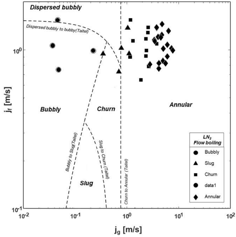
Fig. 8 Flow regime map based on superficial velocities, along with experimentally discerned flow patterns and transition lines predicted by Taitel et al. [49].
