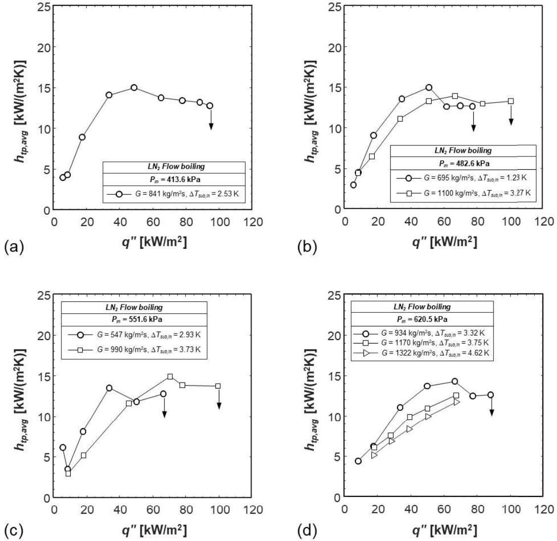
Fig. 12 Variation of average heat transfer coefficient with heat flux for (a) P_{in} = 413.6 \text{ kPa} , G = 841 \text{ kg}/\text{m}^2\text{s} , (b) P_{in} = 482.6 \text{ kPa} , G = 695 \text{ kg}/\text{m}^2\text{s} and G = 1100 \text{ kg}/\text{m}^2\text{s} , (c) P_{in} = 551.6 \text{ kPa} , G = 547 and 990 \text{ kg}/\text{m}^2\text{s} , (d) P_{in} = 620.5 \text{ kPa} , G = 934 , 1170 , and 1322 \text{ kg}/\text{m}^2\text{s} .
