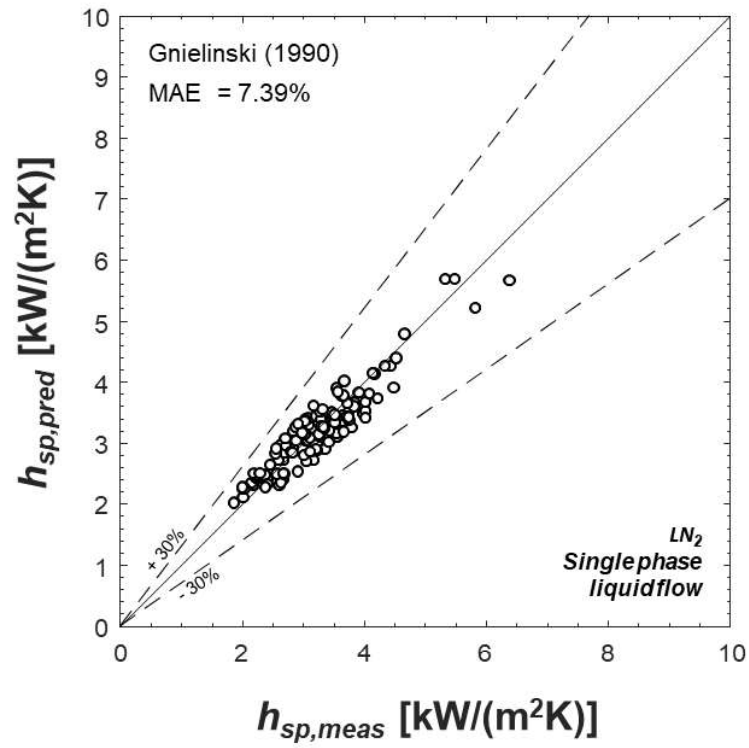
Fig. 6 Comparison of single phase heat transfer coefficients measured in terrestrial environment against predicted single phase heat transfer coefficients calculated by Gnielinski [43] correlation.
