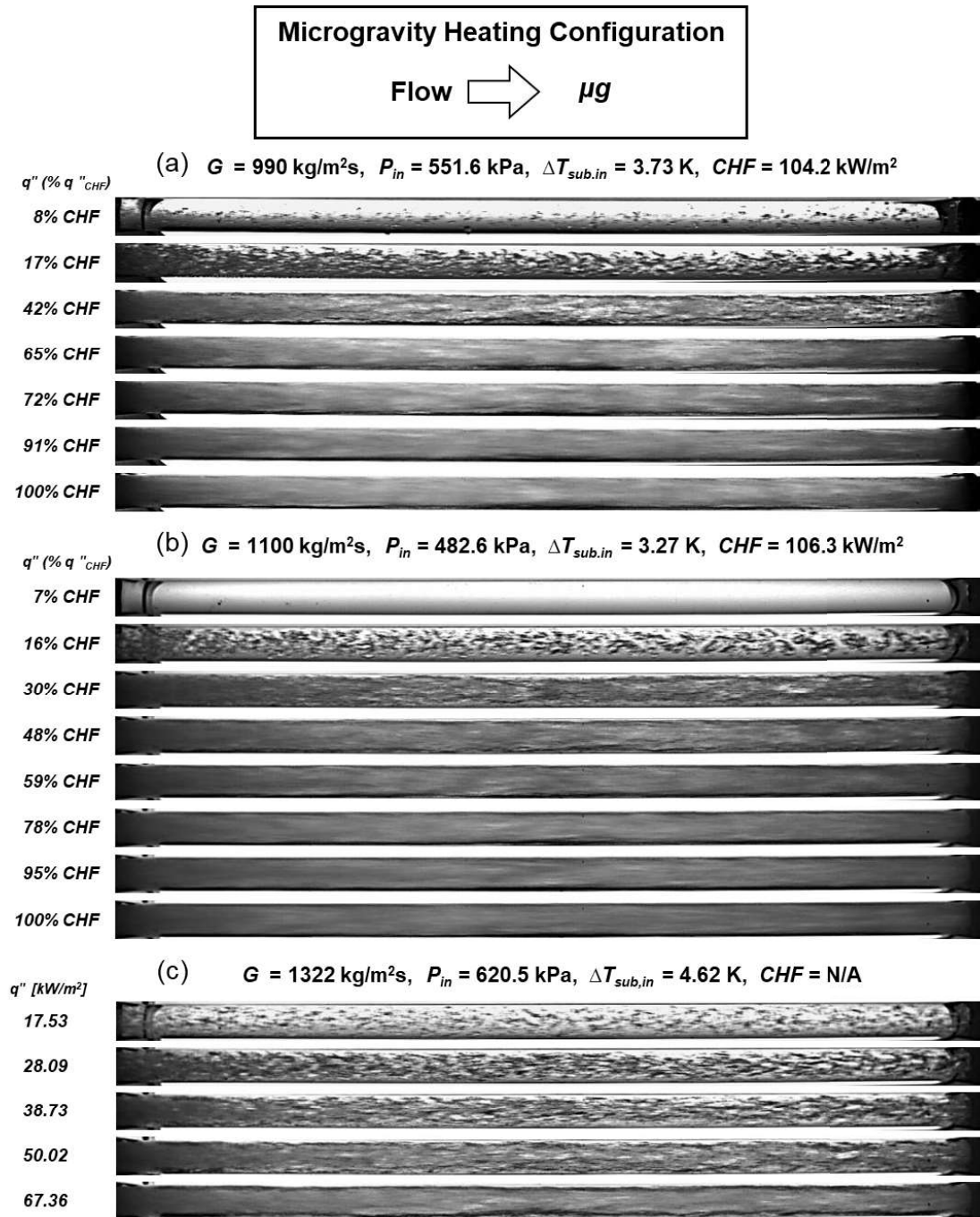
Fig. 3 Two-phase flow structure development along the boiling curve for near-saturated inlet at mass velocities of G = (a) 990, (b) 1100, and (c) 1322 \text{kg/m}^2\text{s} .
