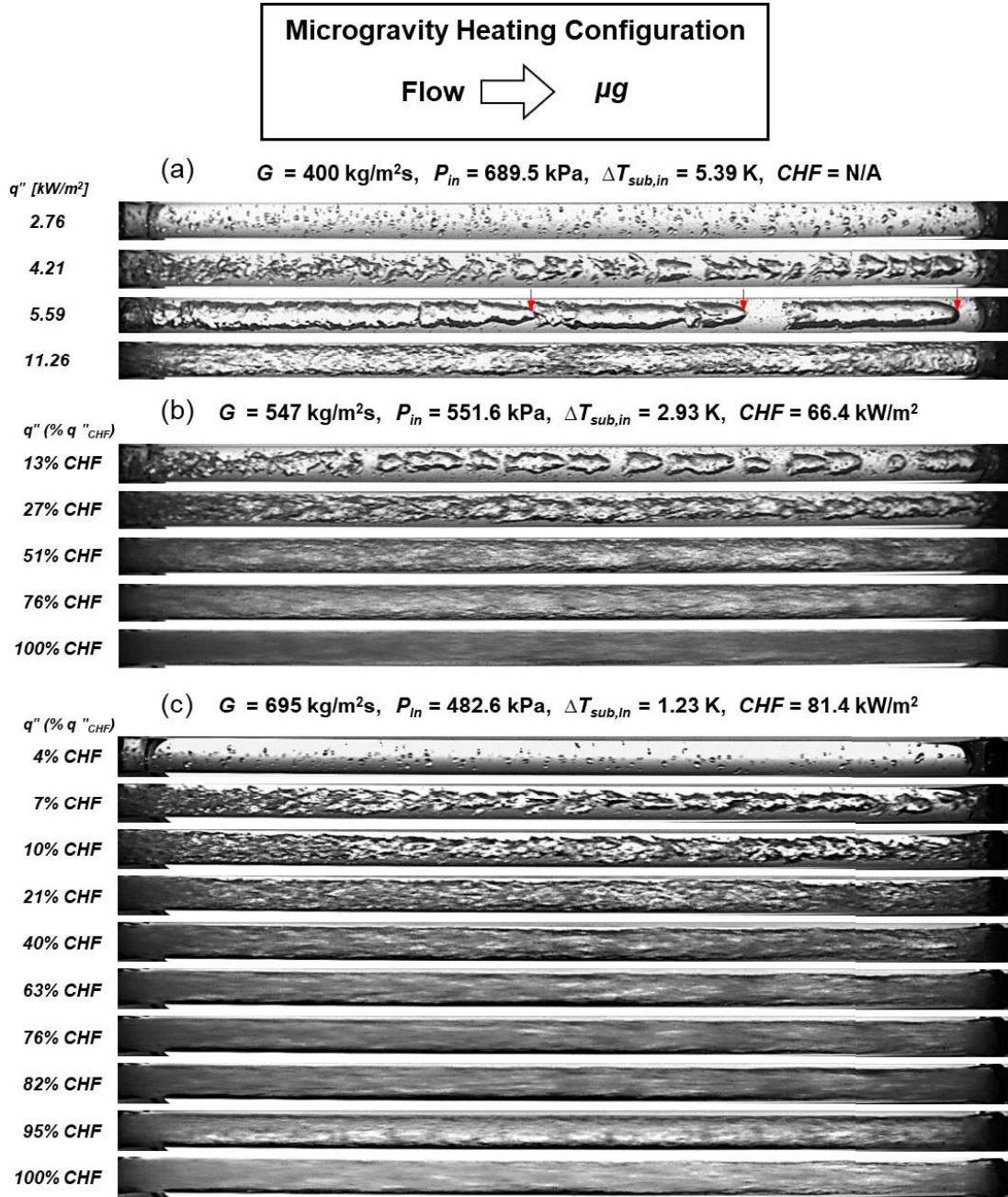
Fig. 1 Two-phase flow structure development along the boiling curve for near-saturated inlet at mass velocities of G = (a) 400, (b) 547, and (c) 695 \text{kg/m}^2\text{s} .
