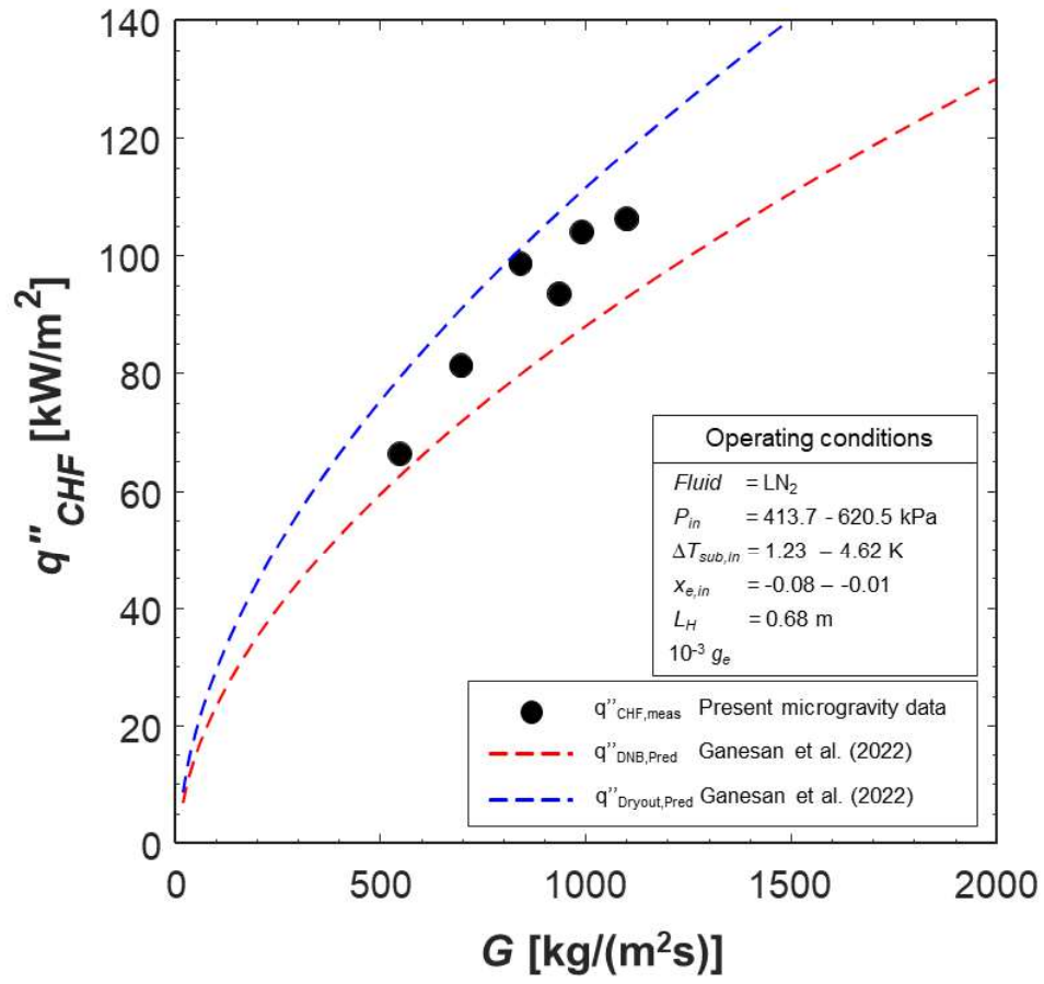
Fig. 10 Variation of measured microgravity CHF with mass velocity compared to predictions of terrestrial-based CHF correlations corresponding to Dryout and DNB.
