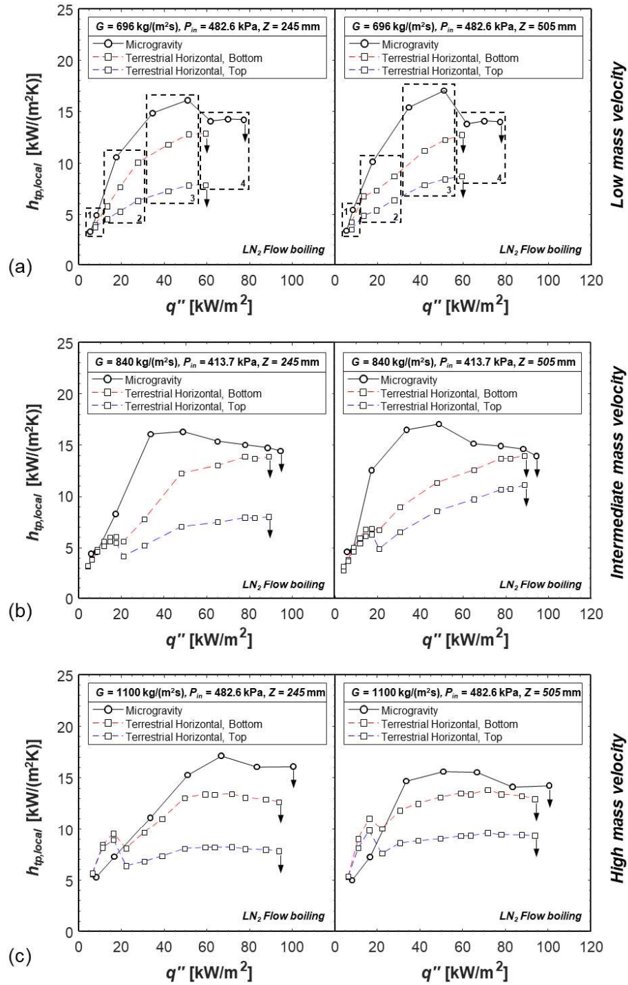
Fig. 24 Effects of gravity on local heat transfer coefficient for near-saturated inlet and mass velocities of G = (a) 695 , (b) 840 , and (c) 1100 \text{ kg/m}^2\text{s} at two different axial location of z = 245 and 505 \text{ mm} .
