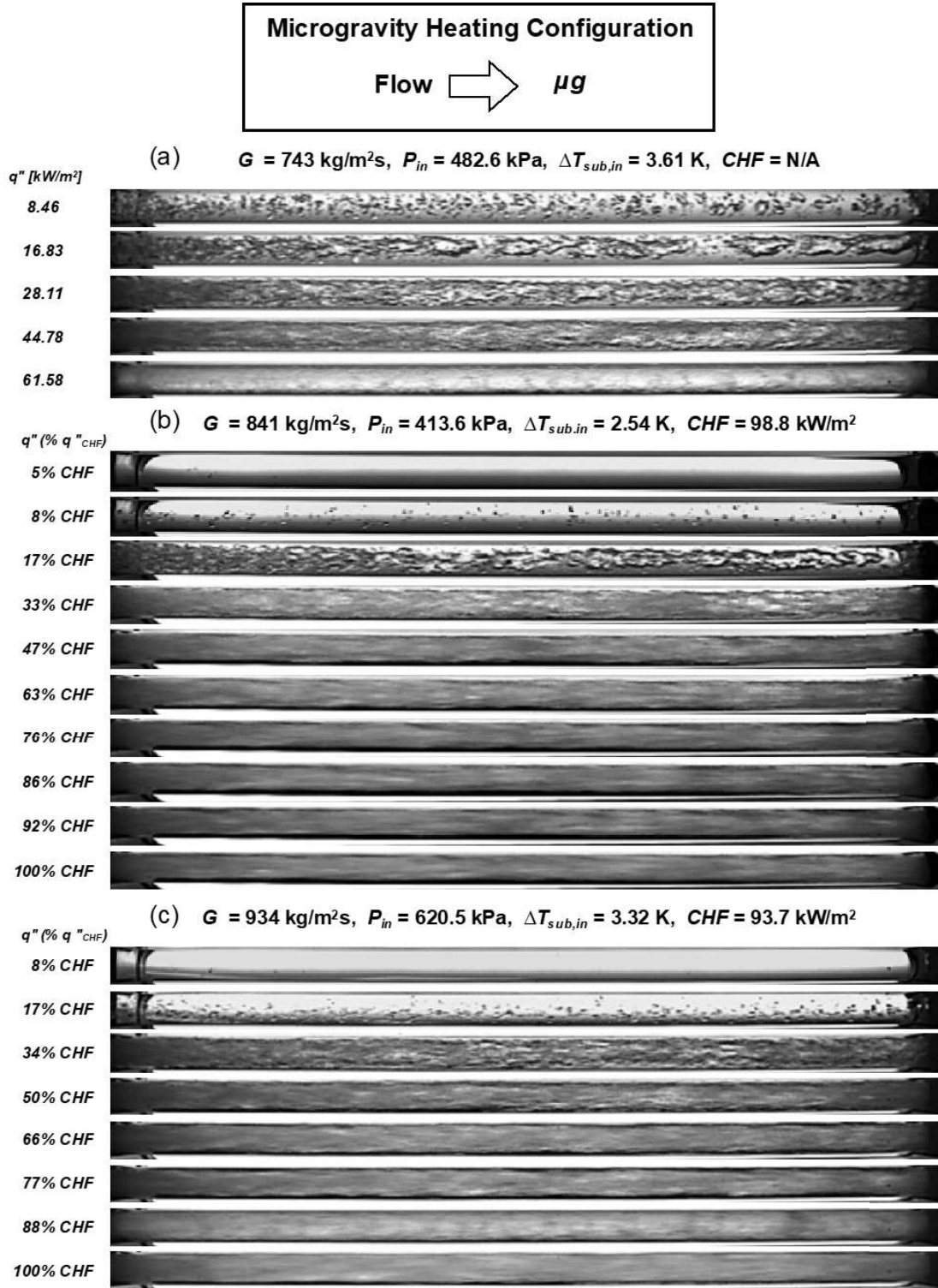
Fig. 2 Two-phase flow structure development along the boiling curve for near-saturated inlet at mass velocities of G = (a) 743, (b) 841, and (c) 934 kg/m 2 s.
