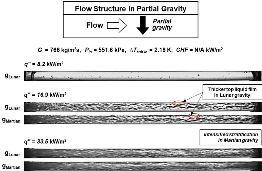
Fig. 7 Two-phase flow patterns in Lunar gravity and Martian gravity for near-saturated inlet, mass velocity of G = 766 \text{ kg/m}^2\text{s} , and different heat fluxes.
