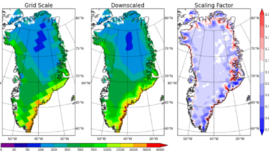
GEOS precipitation downscaling scheme.
