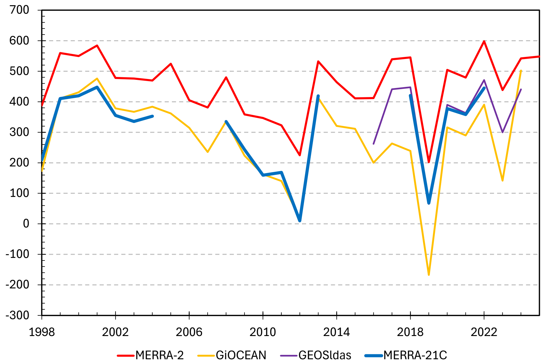
Annual Surface Mass Balance [ Gt ]
