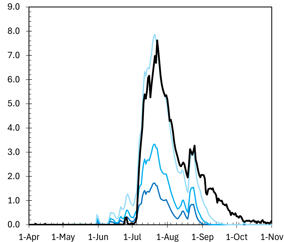
Meltwater Content, Southwest GrIS, 2023 [ Gt ]
