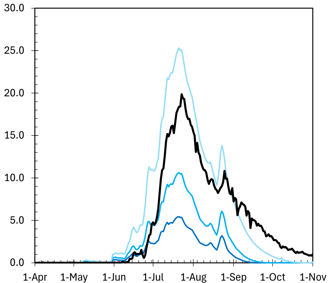
Meltwater Content, Pan-GrIS, 2023 [ Gt ]
