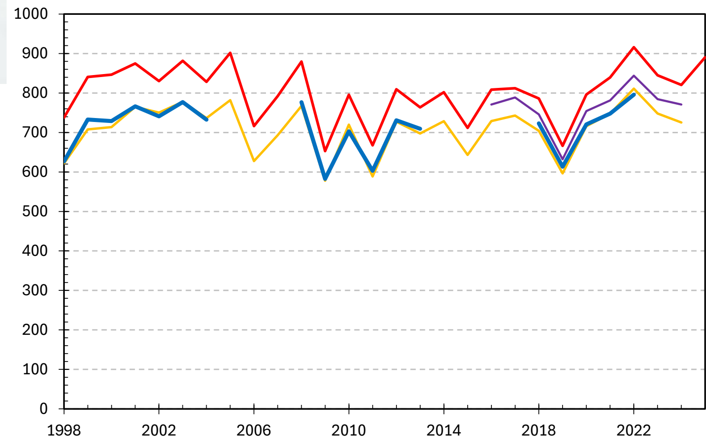
Annual Runoff [ Gt ]
