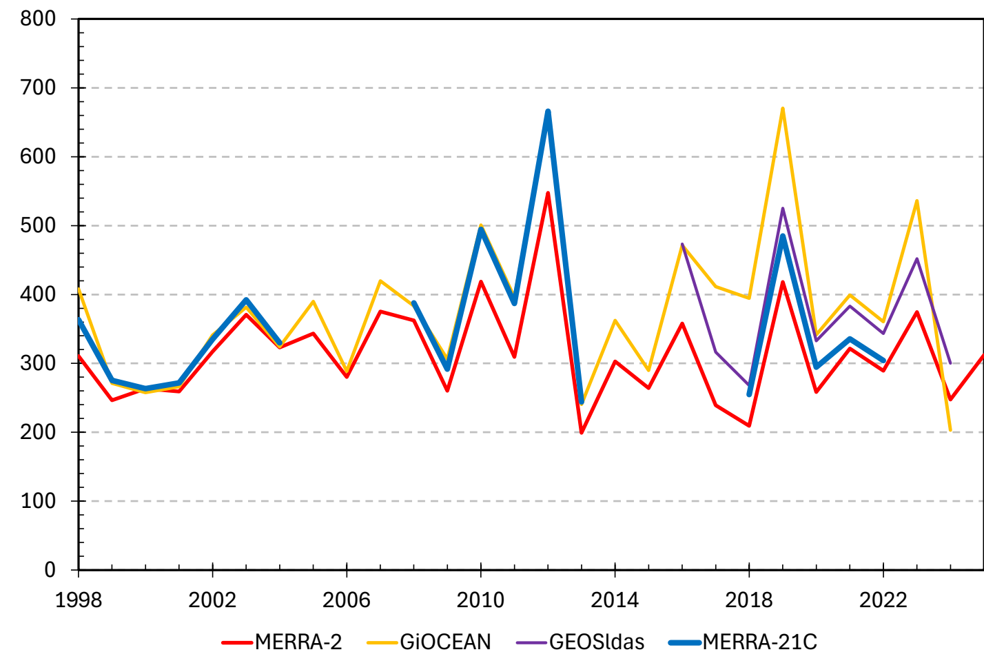
Annual Runoff [ Gt ]
