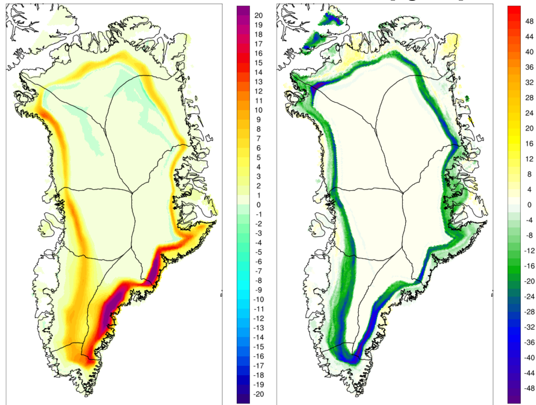
Runoff [kg m -2 ]
