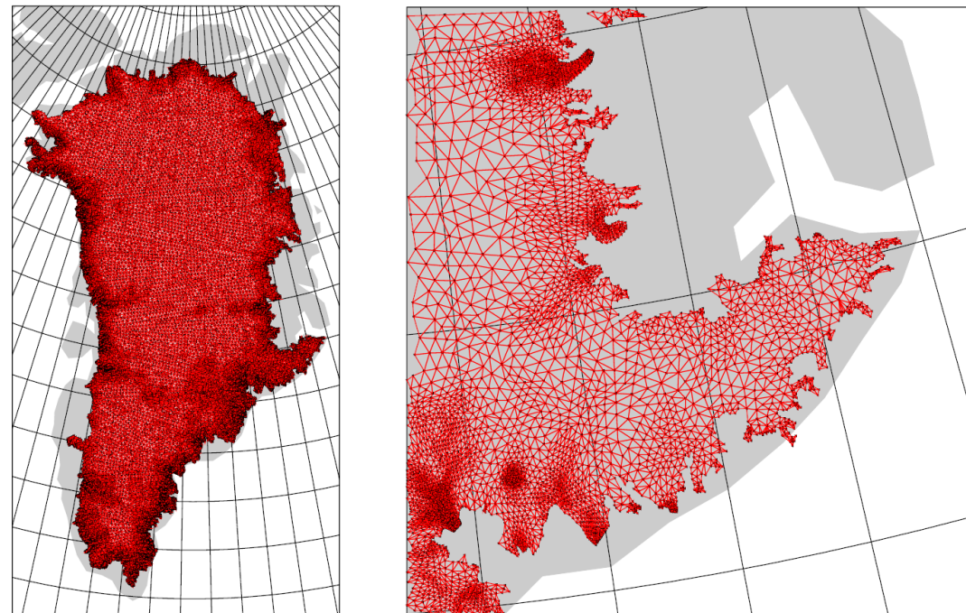
ISSM mesh, and GEOS AGCM grid.
