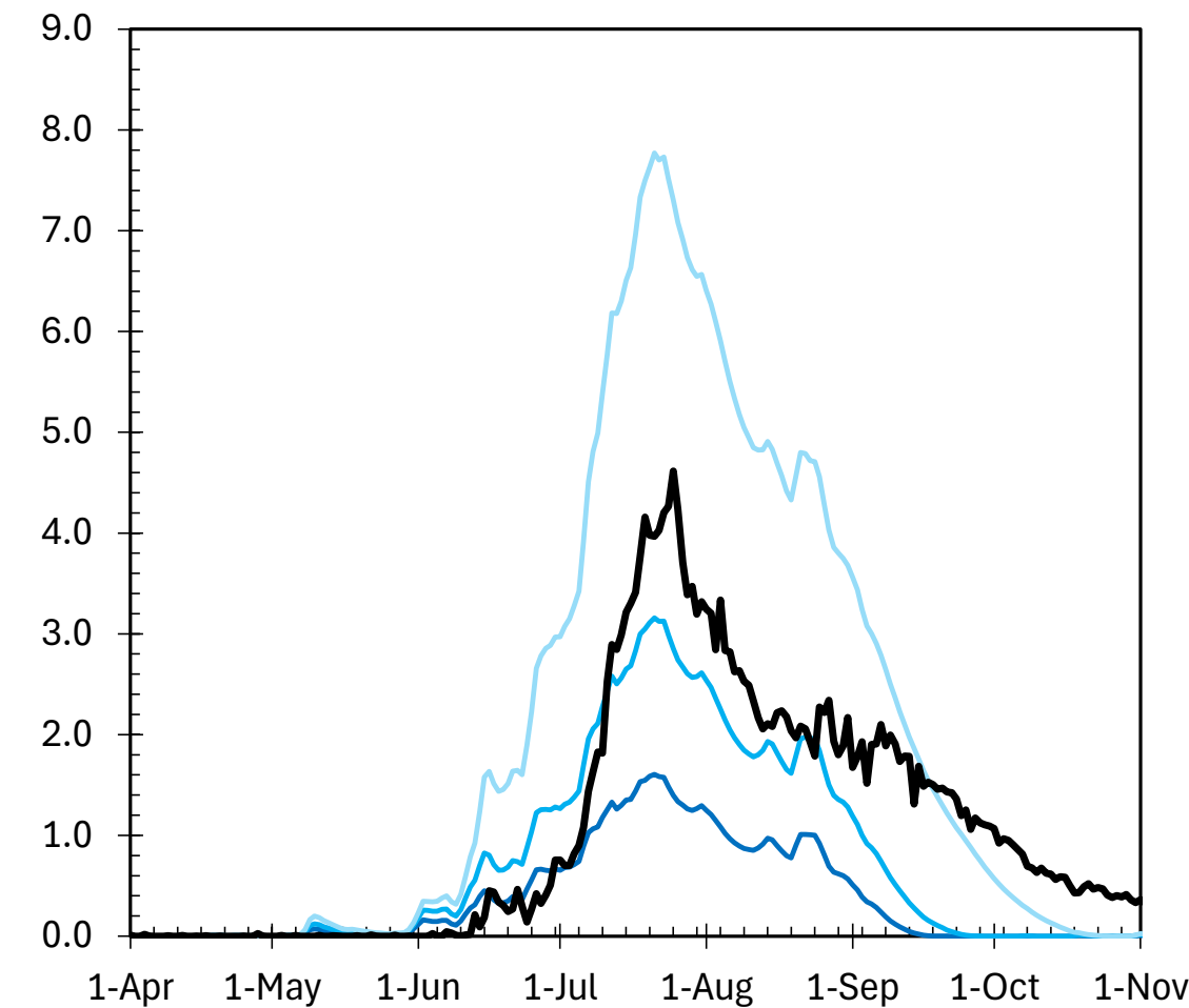
Meltwater Content, Southeast GrIS, 2023 [ Gt ]
