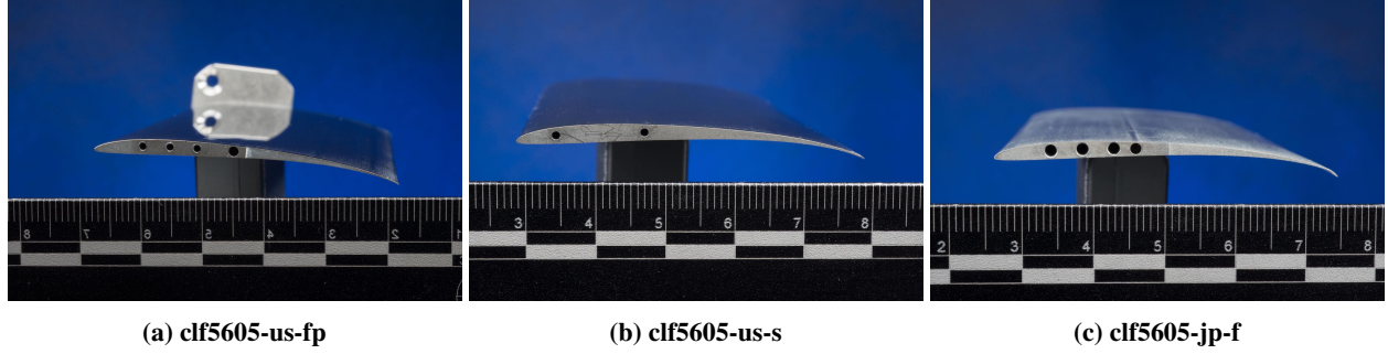
Fig. 6 Images of CLF5605 models (scale shown in cm).
