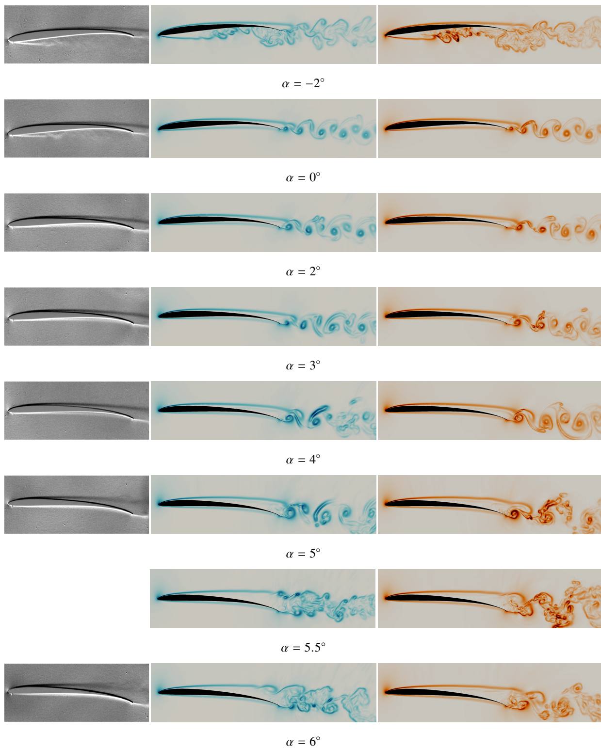
Fig. 33 Schlieren images for MWT experiments on model clf5605-us-s (left) and images of instantaneous density gradient magnitude |\nabla\rho| for 3D-SP OVERFLOW (middle) and PyFR (right) on CLF5605 for different \alpha .
