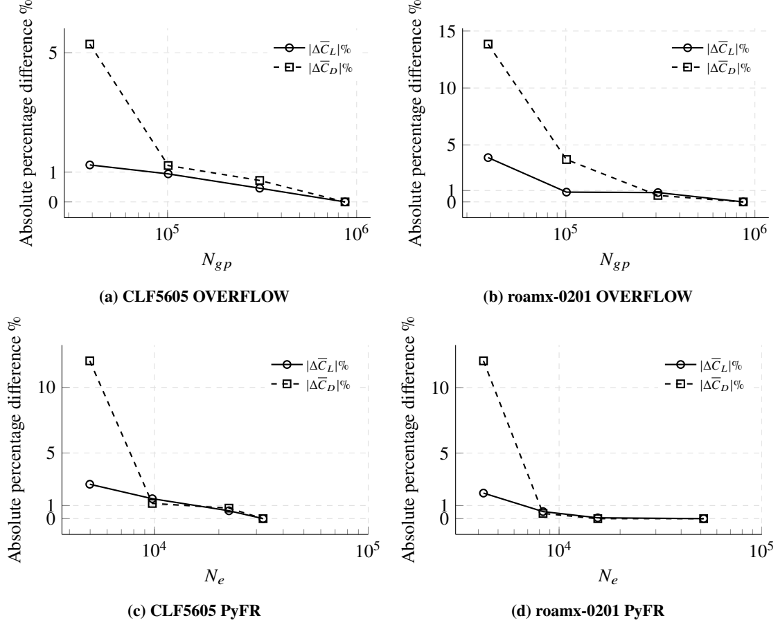
Fig. 23 Absolute percentage differences in time-averaged lift and drag coefficients with respect to the finest mesh, |\Delta \bar{C}_L| \% and |\Delta \bar{C}_D| \% , plotted as a function of the number of grid points N_{gp} for 2D OVERFLOW and number of elements N_e for 2D PyFR to assess grid convergence of CLF5605 and roamx-0201 at \alpha = 6^\circ .
