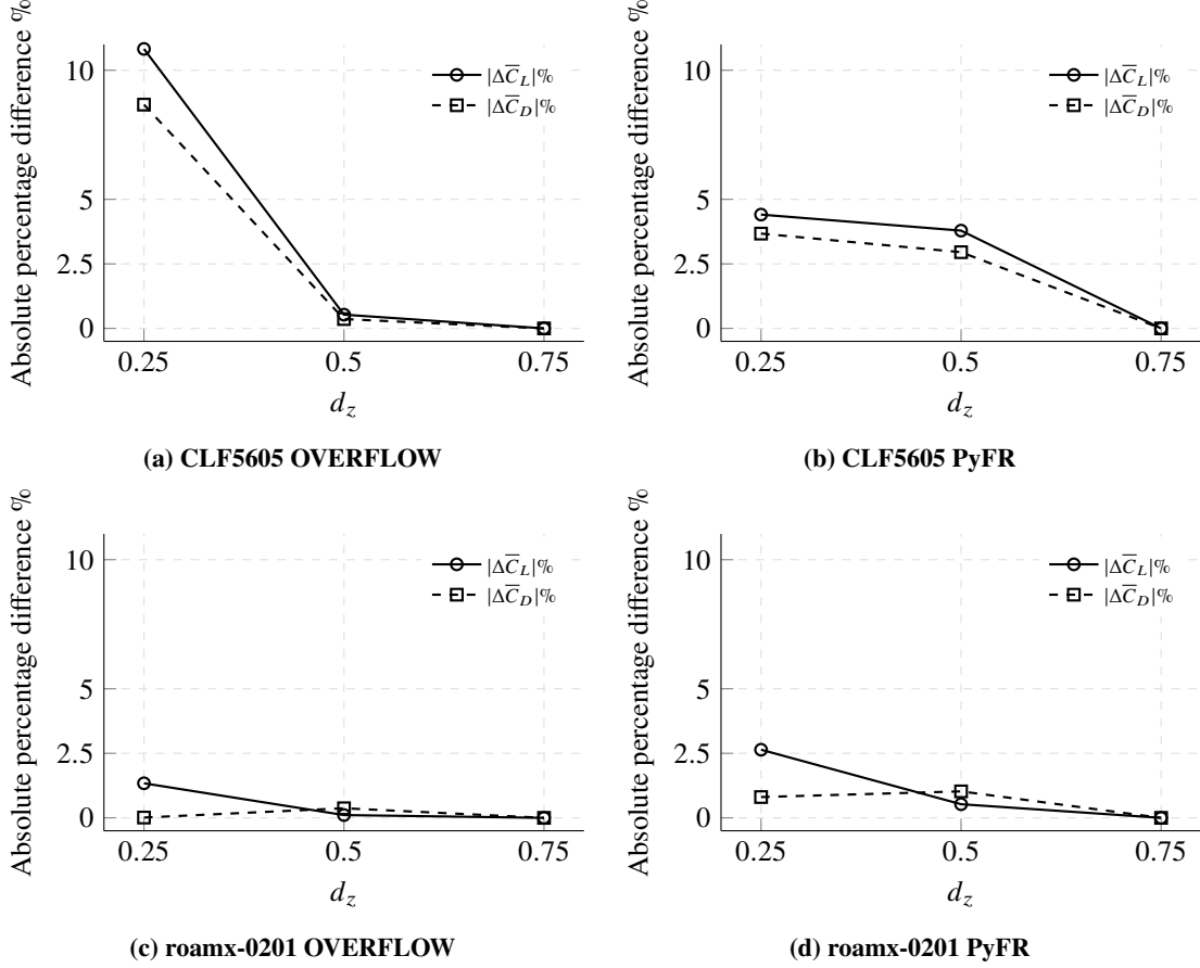
Fig. 25 Absolute percentage differences in time-averaged lift and drag coefficients with respect to the largest spanwise extent of the domain d_z = 0.75 , |\Delta \bar{C}_L| \% and |\Delta \bar{C}_D| \% , plotted as a function of d_z for 3D-SP OVERFLOW and 3D-SP PyFR to assess the required spanwise extent of the domain for CLF5605 and roamx-0201 at \alpha = 6^\circ .
