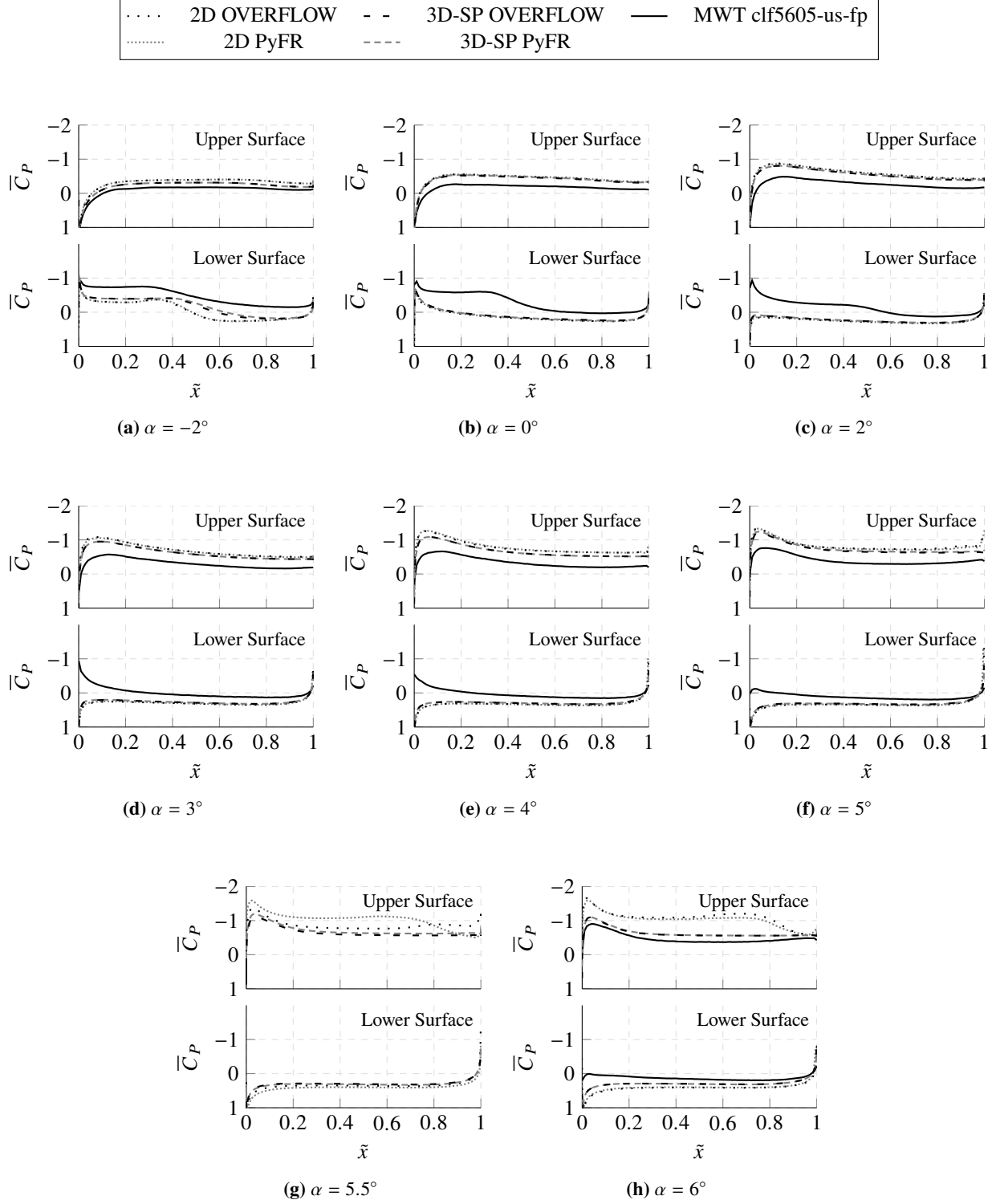
Fig. 31 Plots of time-averaged pressure coefficient \bar{C}_P as a function of \tilde{x} for different angles of attack \alpha for the CLF5605 airfoil.
