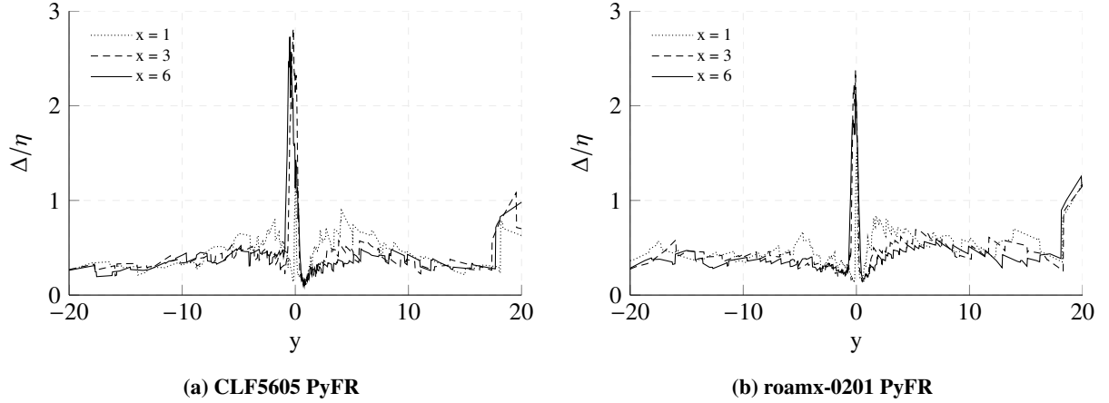
Fig. 27 Plots of \Delta/\eta in the mid-span plane as a function of y at x = 1 , x = 3 and x = 6 for 3D-SP PyFR at \alpha = 6^\circ .
