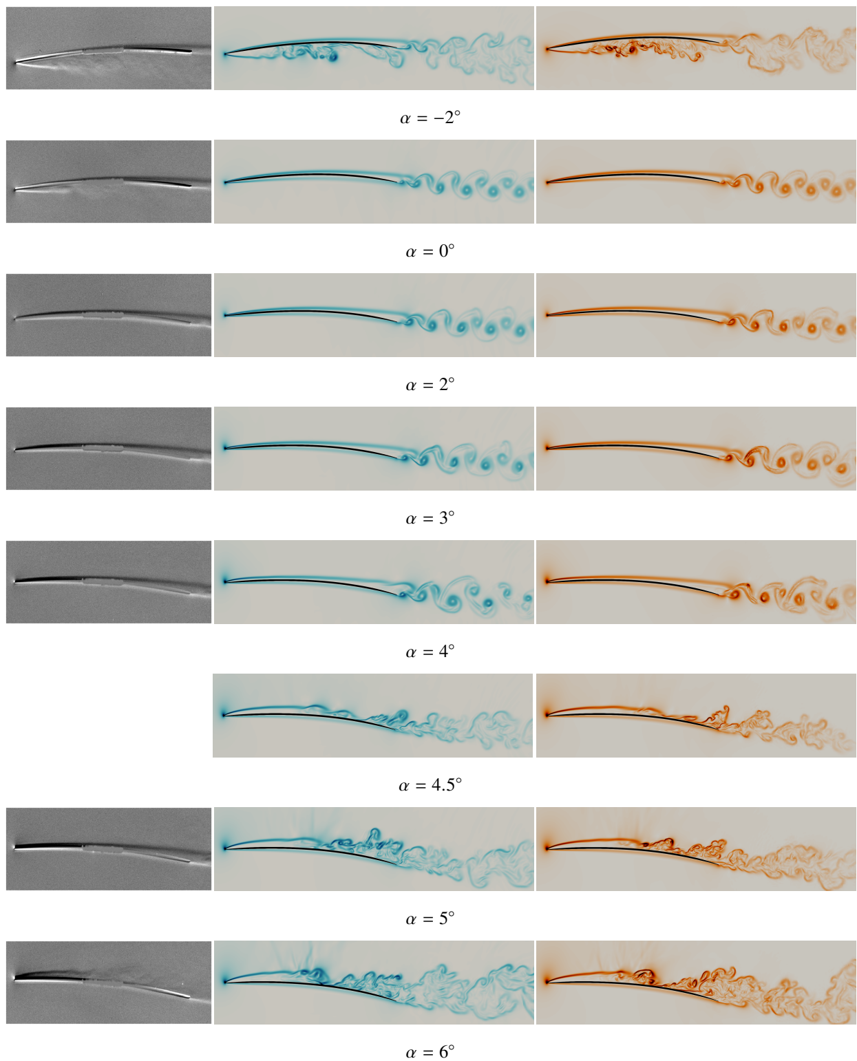
Fig. 34 Schlieren images for MWT experiments on model roamx-0201-jp-s (left) and images of instantaneous density gradient magnitude |\nabla\rho| for 3D-SP OVERFLOW (middle) and PyFR (right) on roamx-0201 for different \alpha .
