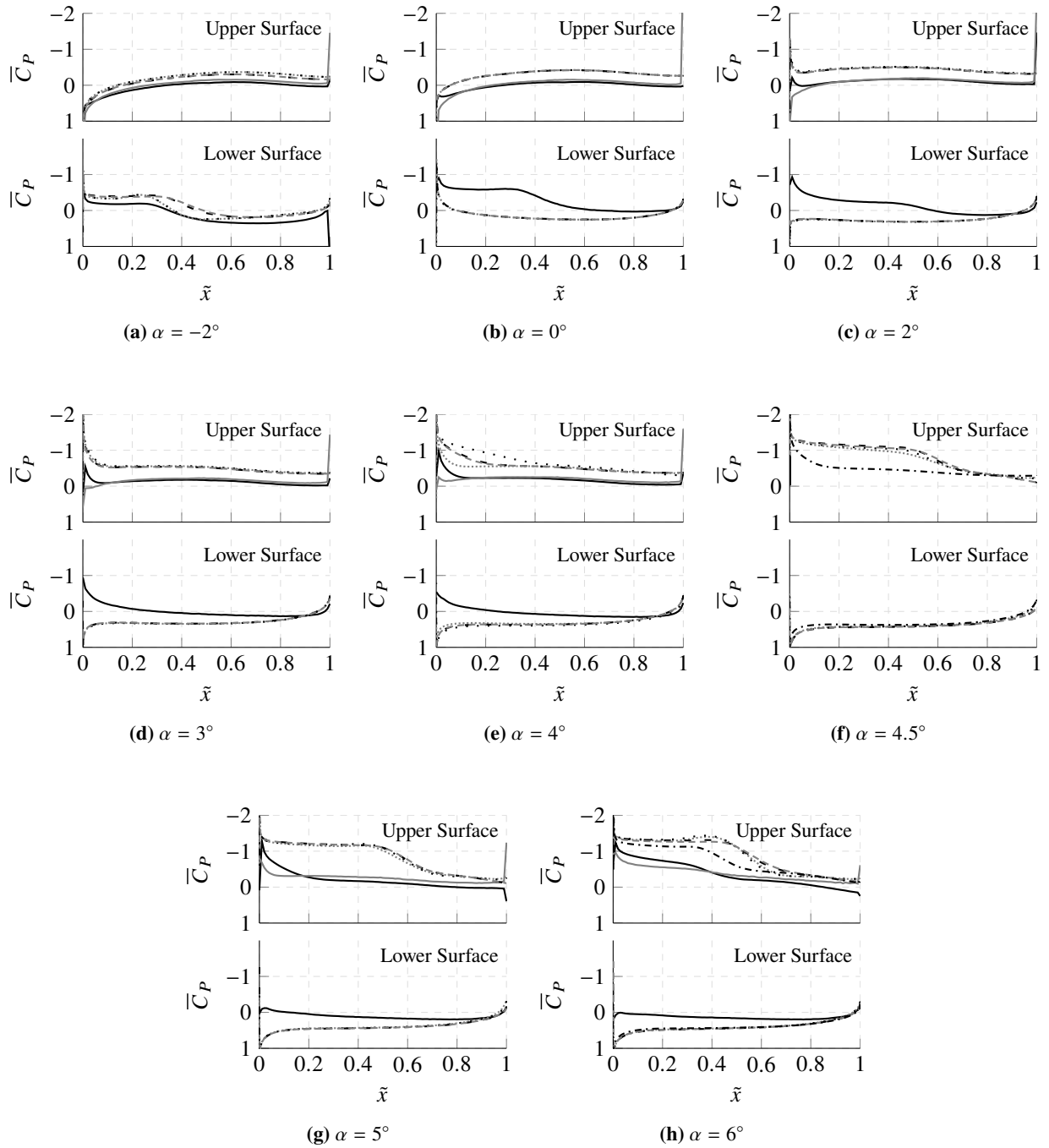
Fig. 32 Plots of time-averaged pressure coefficient \bar{C}_P as a function of \tilde{x} for different angles of attack \alpha for the roamx-0201 airfoil.
