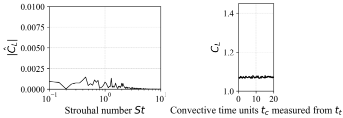
(c) VWT PyFR
