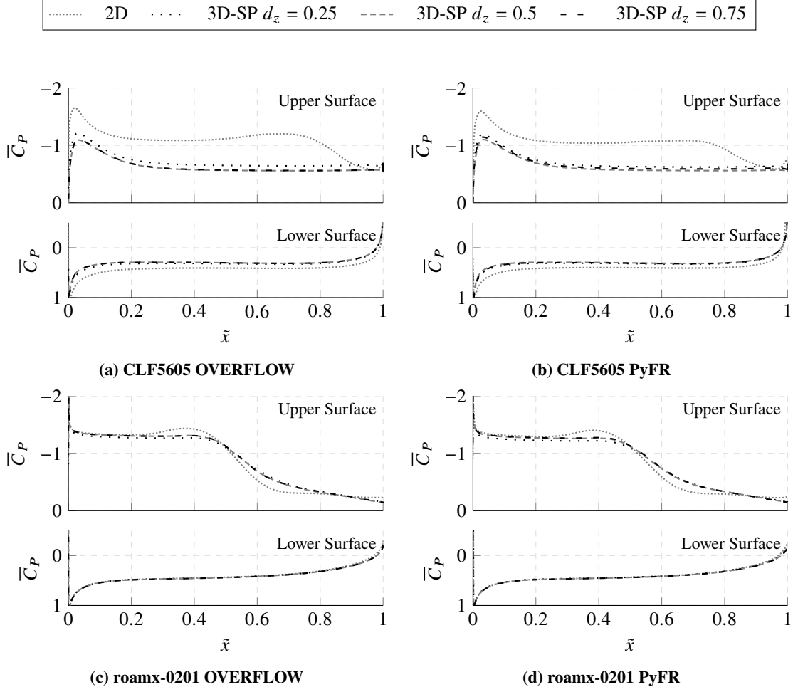
Fig. 24 Plots of time-averaged pressure coefficient \bar{C}_P as a function of \tilde{x} for different span lengths of the domain d_z to assess domain span length independence for 3D-SP OVERFLOW and PyFR simulations of CLF5605 and roamx-0201 at \alpha = 6^\circ .
