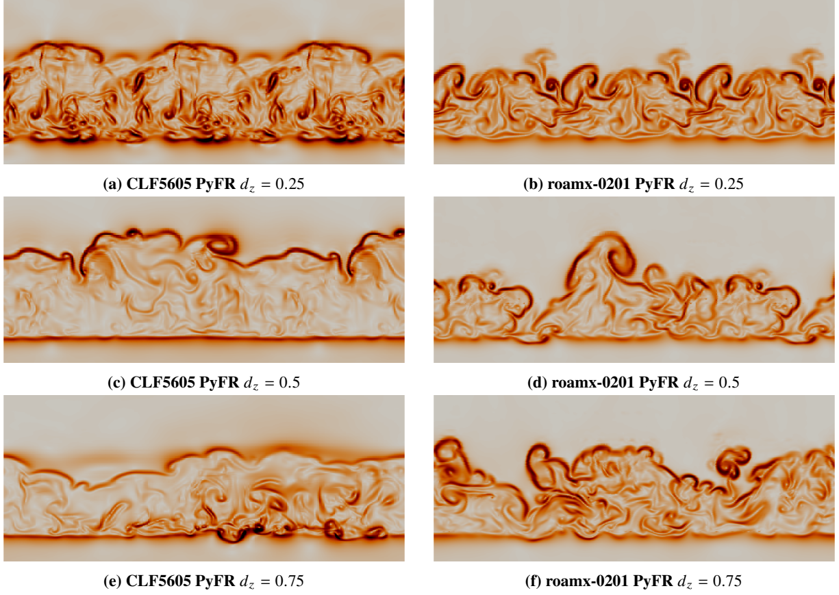
Fig. 26 Images of instantaneous density gradient magnitude |\nabla\rho| in the y-z plane at a distance of 0.05 chord lengths from the trailing edge for 3D-SP PyFR on CLF5605 (left) and roamx-0201 (right) at \alpha = 6^\circ with domain span lengths of d_z = 0.25 , d_z = 0.5 and d_z = 0.75 chord lengths. Note that for d_z = 0.25 and d_z = 0.5 chord lengths the periodic data is repeated 3 and 1.5 times, respectively, to facilitate comparison.
