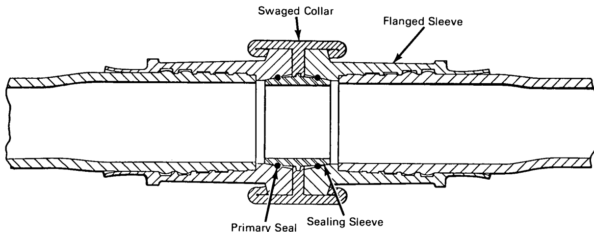
Assembled X-Connector; 0.5-in. Tubing
