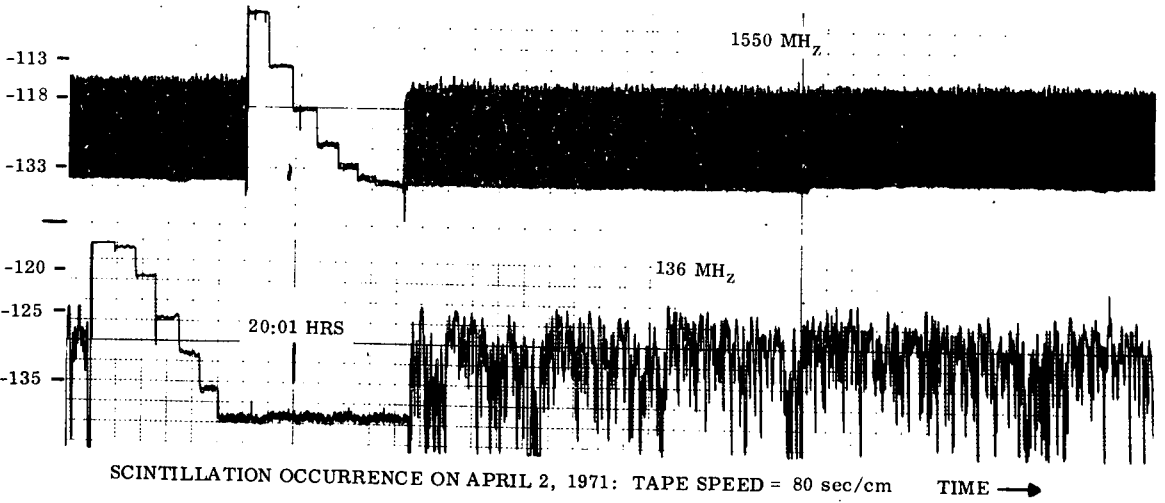
Figure 6. L-Band and VHF Scintillation Records Received from ATS 5
