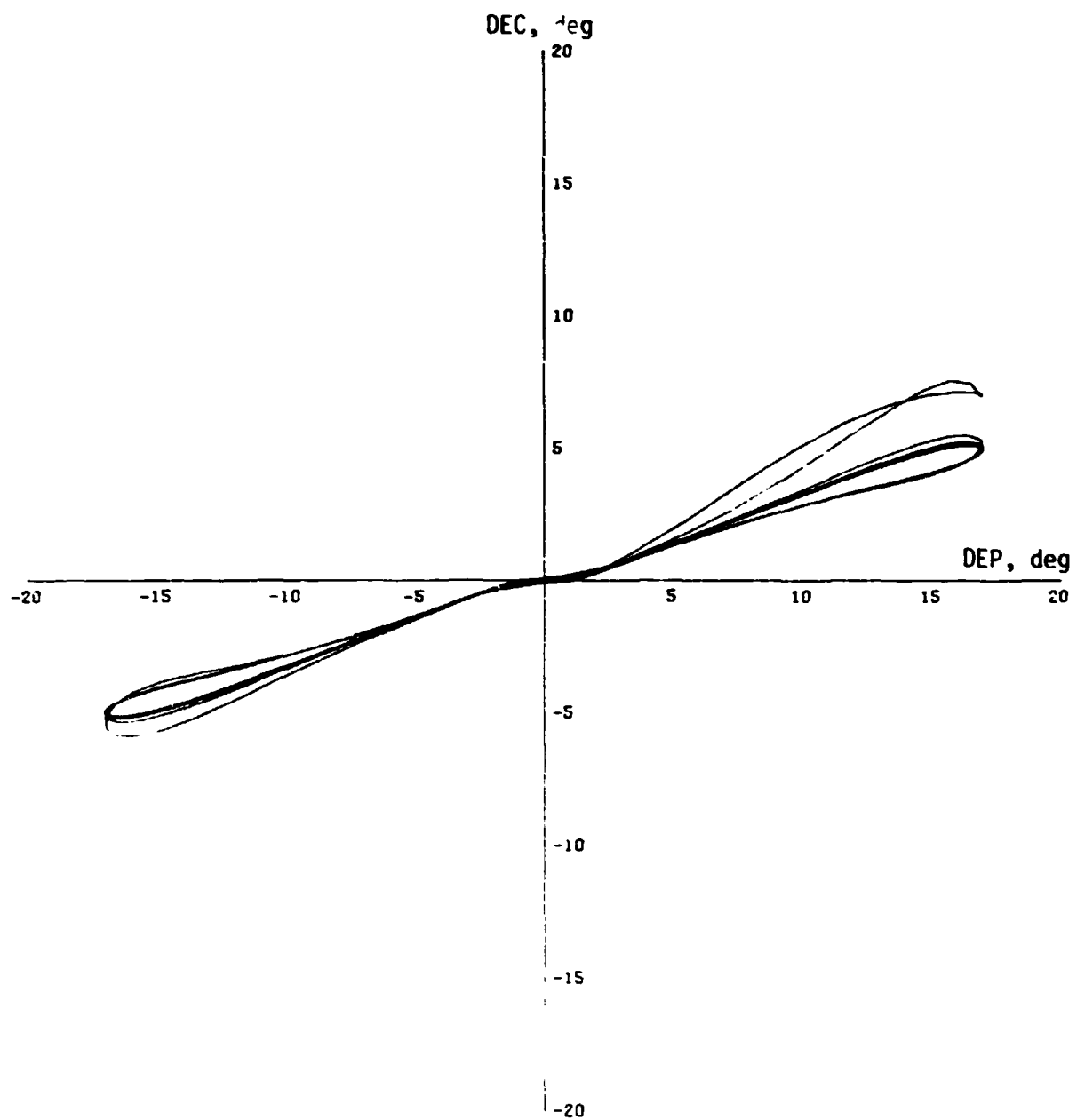
(a) DEP = 17^{\circ} \sin \omega t .
