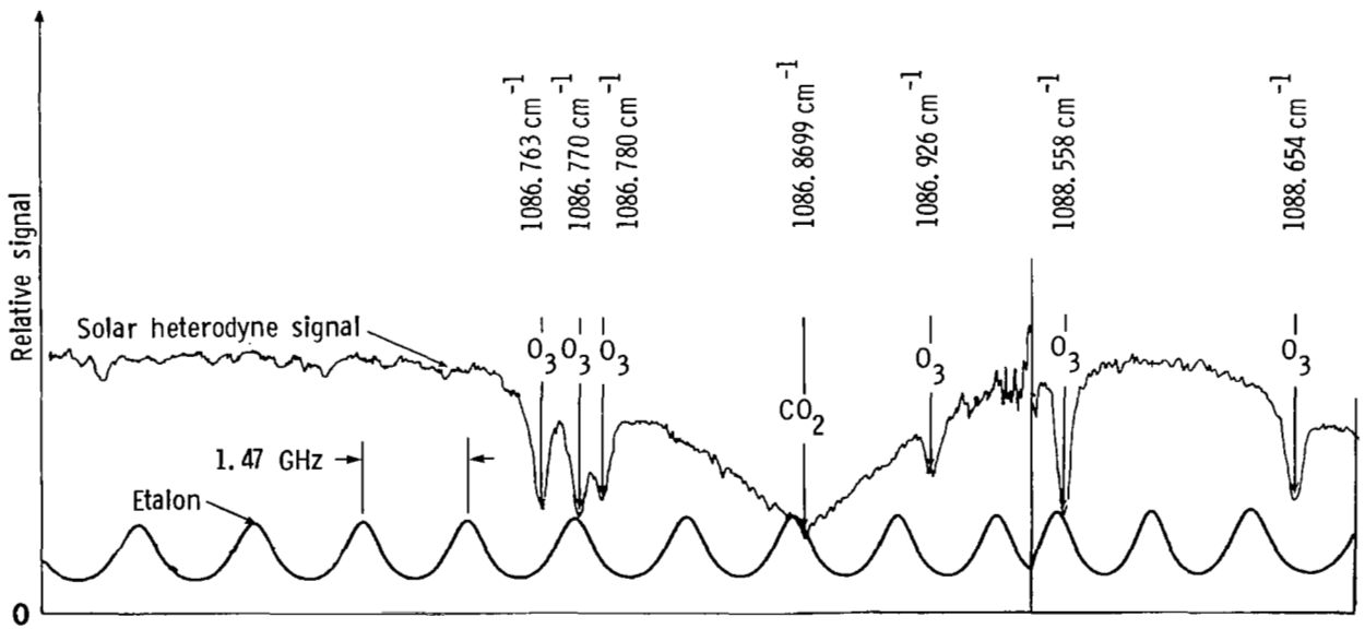
Figure 4.- Heterodyne solar absorption spectra of atmospheric ozone and CO 2 . The absolute wavelength was identified by the broad atmosphere R(34) (00 0 1 - 02 0 0 ) CO 2 line.
