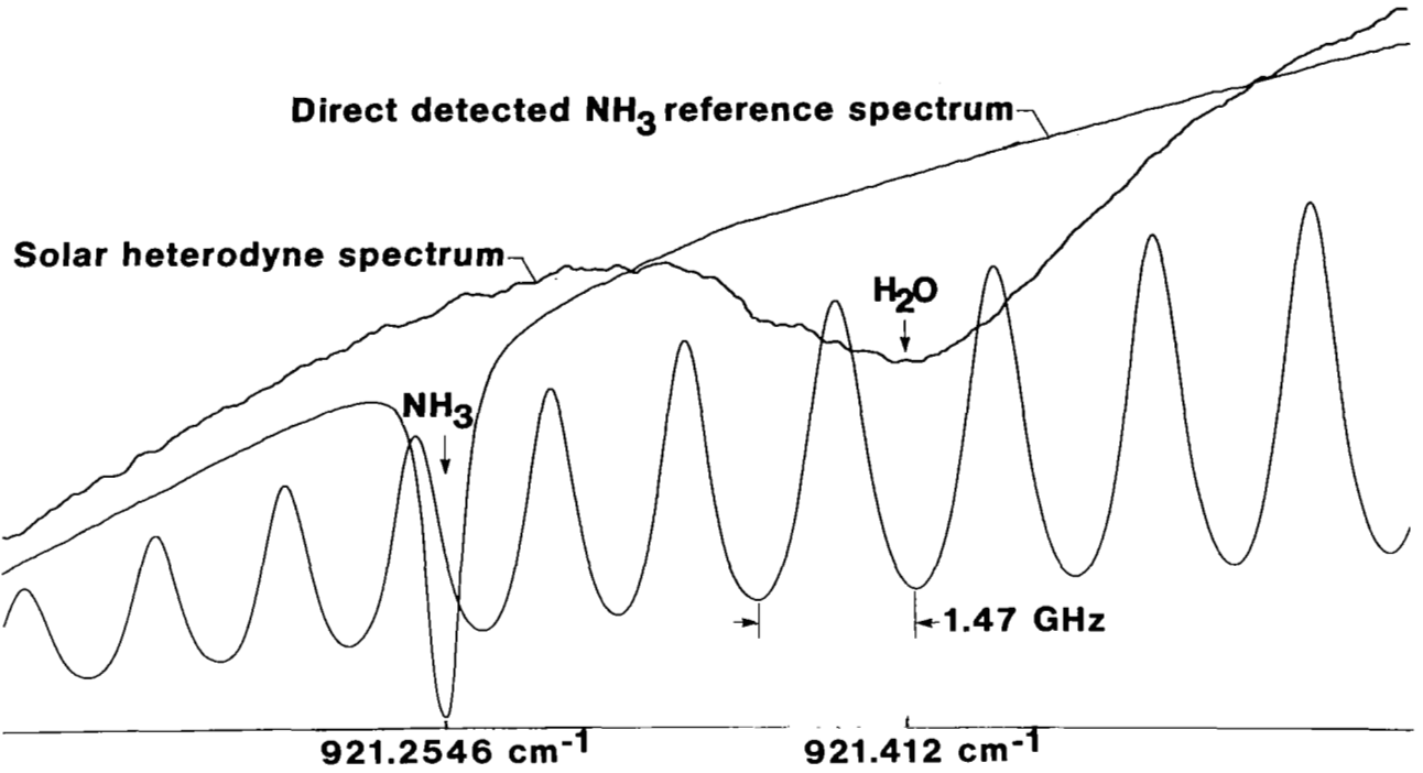
Figure 3.- Heterodyne solar absorption spectrum of atmospheric water vapor with NH 3 as the reference gas.
