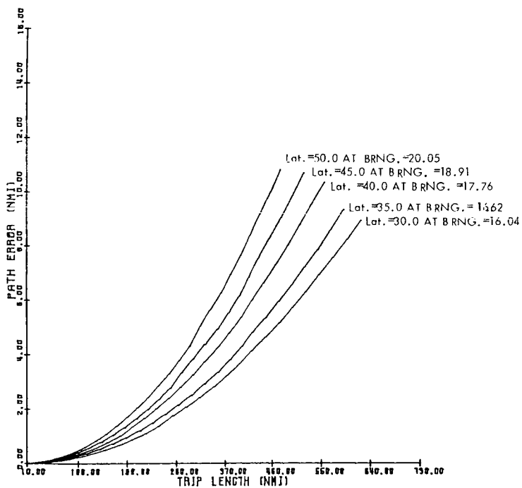
Figure 6. Path errors versus trip length at average bearing 18^{\circ} .
