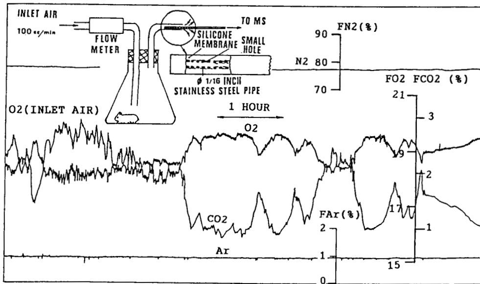
Fig.4. Over night monitoring of the exhtust gas concentration from the hamster chamber. The measurement was performed by employing a silicone membrane probe.
