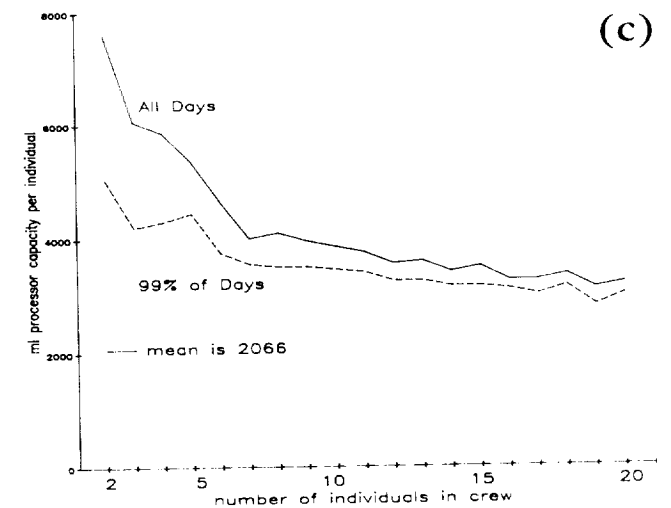
Fig. 3. 24-hour urine samples. (a) Dashed line is 24-hour samples, solid line is means of individuals. (b) Distribution of samples represented as a multiple of that individual's mean. The 39% of samples that exceed the mean are shown. (c) Required per-person urine processing capacity vs. crew size. The mean is included for comparison.
