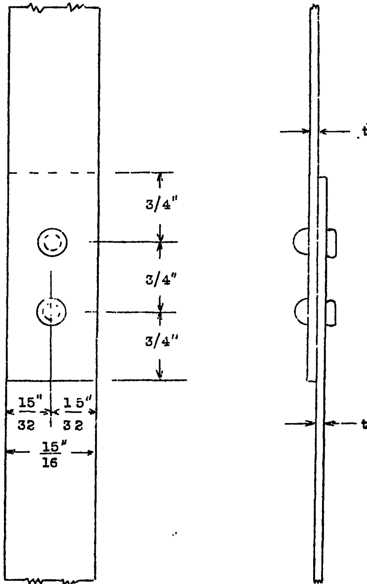
Figure 1.- Test specimen.
