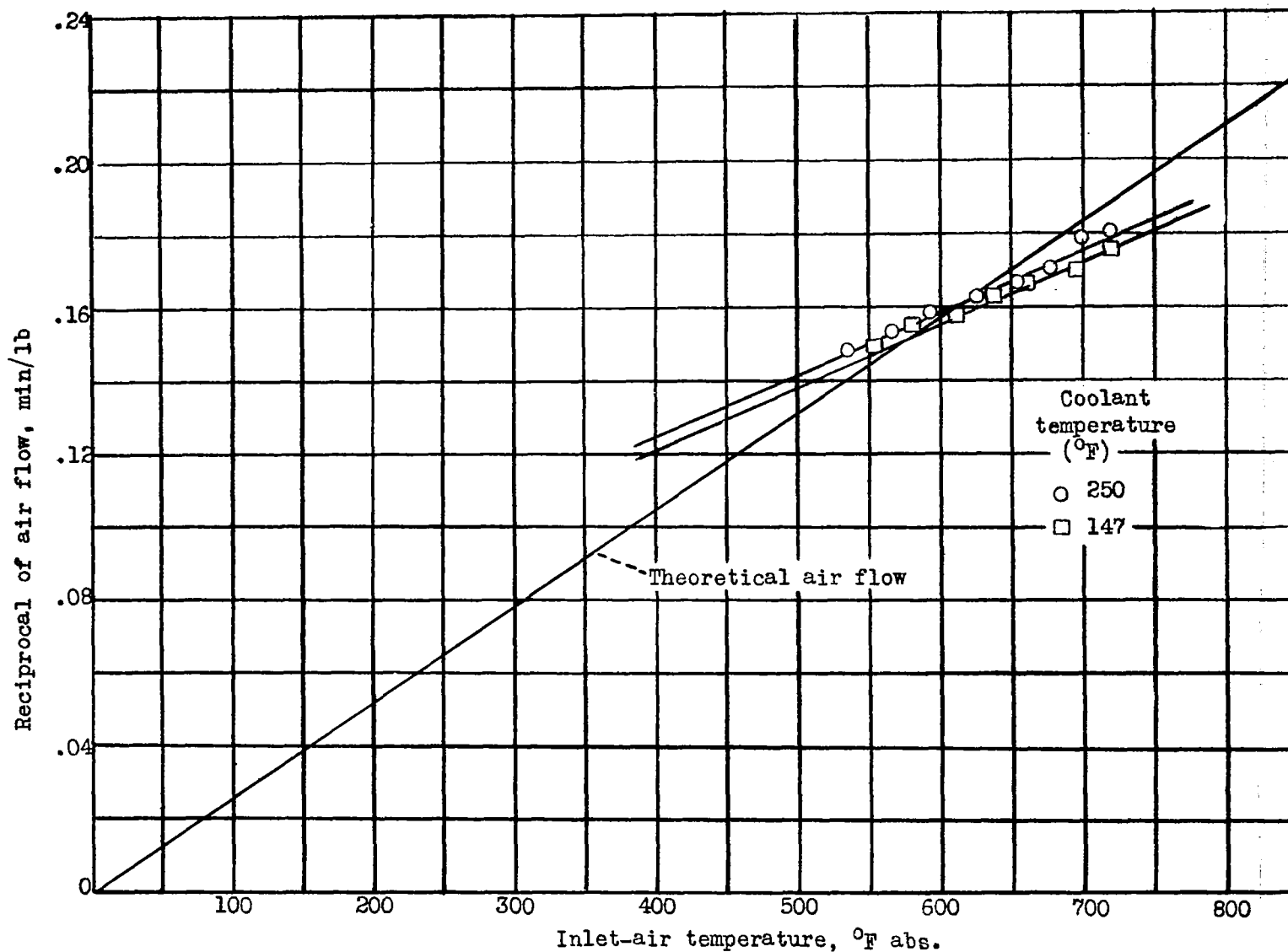
Figure 4.- Comparison of theoretical and measured air flow in an Allison V-1710 cylinder. Engine displacement, 142.5 cubic inches; compression ratio, 6.65; intake valve closes, 62° A.B.C.; engine speed, 2400 rpm; inlet-air pressure, 29.10 inches Hg absolute; exhaust pressure, 30 inches Hg absolute; fuel-air ratio, 0.08.
