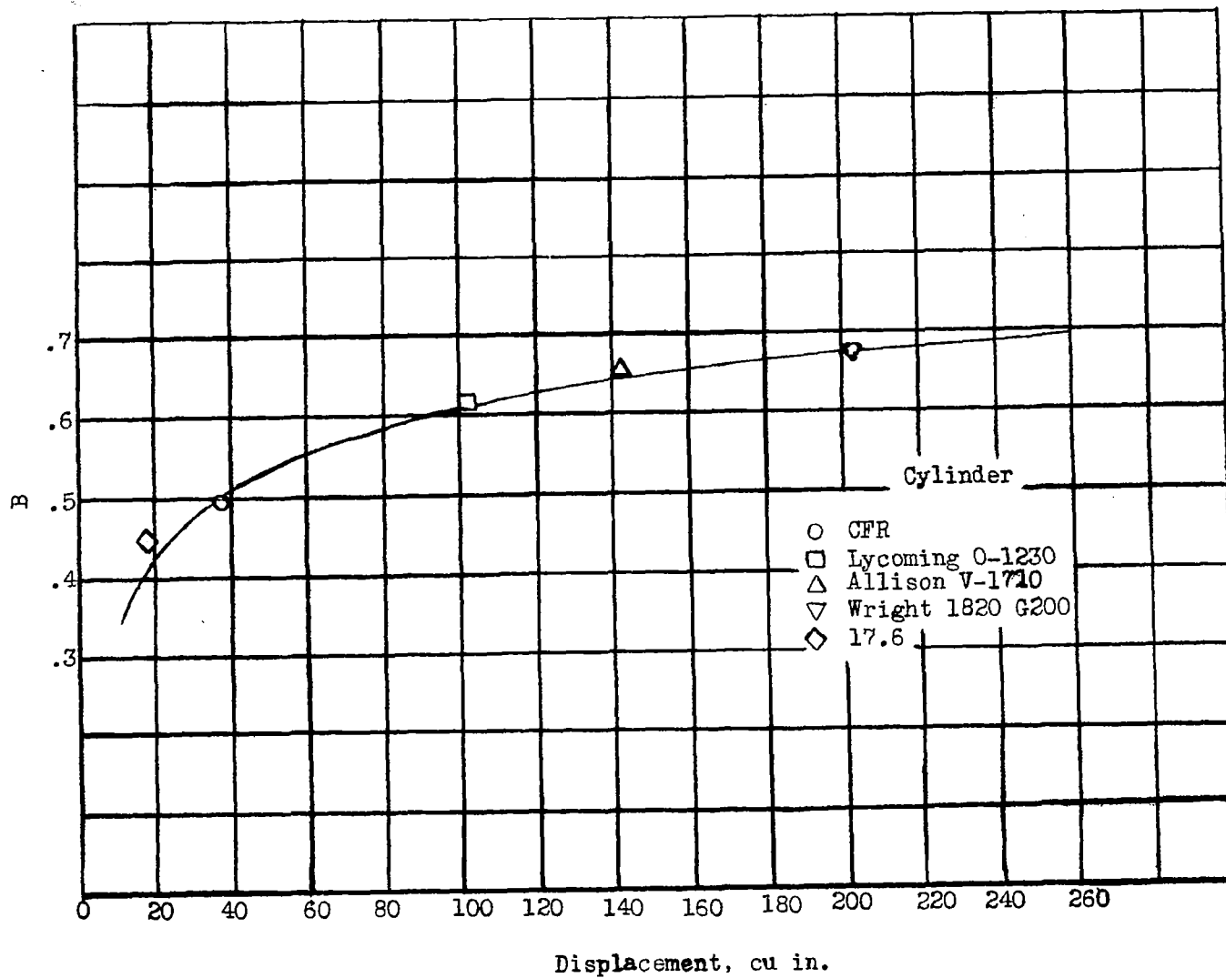
Figure 7.- Effect of cylinder displacement on heating of cylinder charge.
