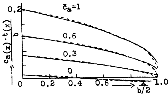
Figure 9.- Comparison curves for a wing with t_a:t_t=0.5 and b^2/F=6.67 for various values of c_a with a linear twist which is 0^\circ at the center and 3^\circ downwards at the wing tip.
