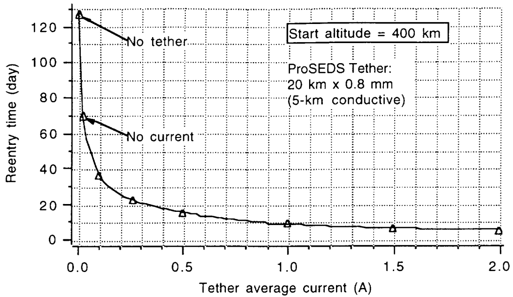
FIGURE 3. Predicted demonstration of ProSEDS propulsive drag thrust. The Delta II reentry time is shown as a function of tether average current. Data provided by Enrico Lorenzini/SAO.
