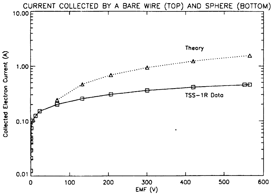
FIGURE 4. Current collected by a bare wire versus a sphere. Data provided by Jim Sorensen and Nobie Stone/NASA.
