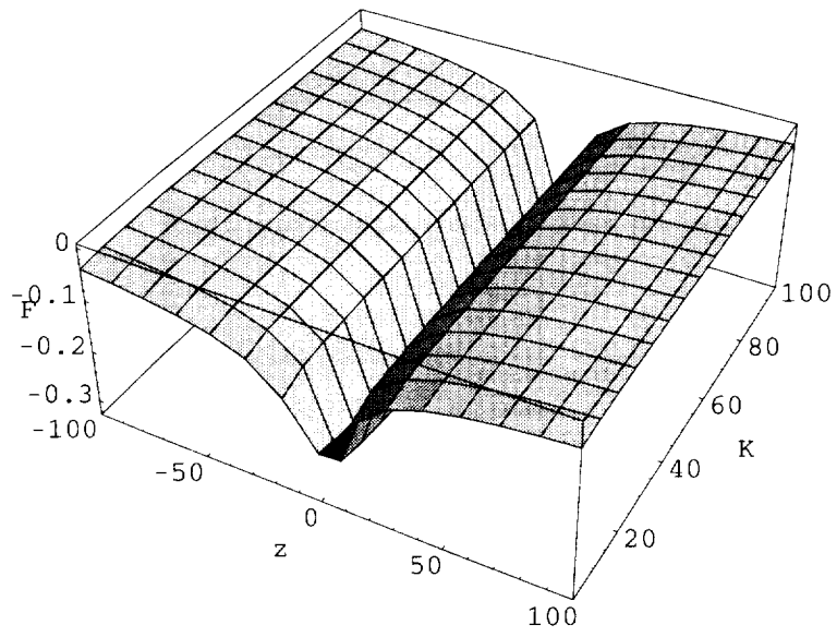
FIG. 4.1. Plot of F(z, K) at c = 1 .
