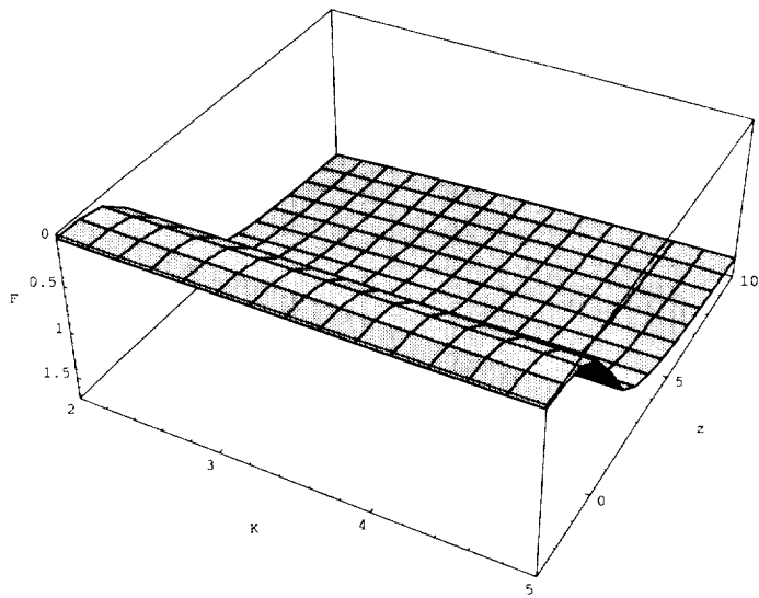
FIG. 4.2. Plot of F(z, K) .
