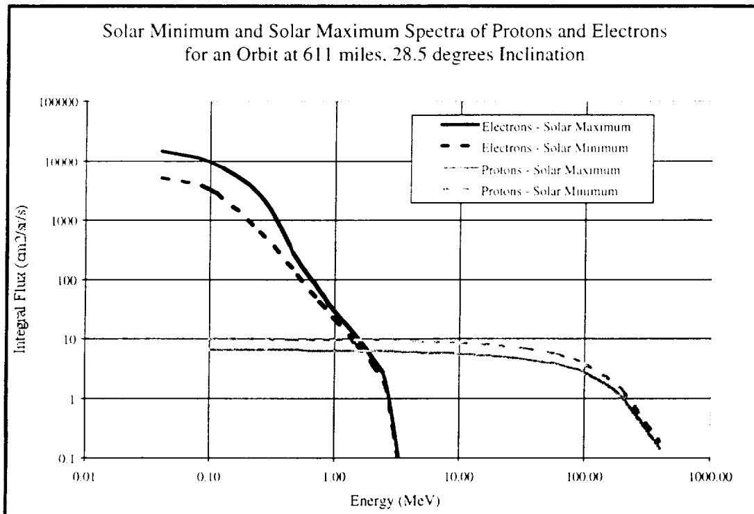
Figure 1. Trapped Proton and Electron Spectra for Solar Maximum and Solar Minimum Conditions.
