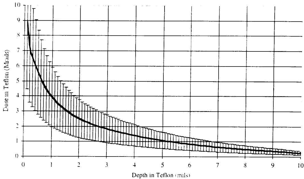
Trapped Electron Dose vs. Depth in Teflon for 10 years at the Hubble Orbit
