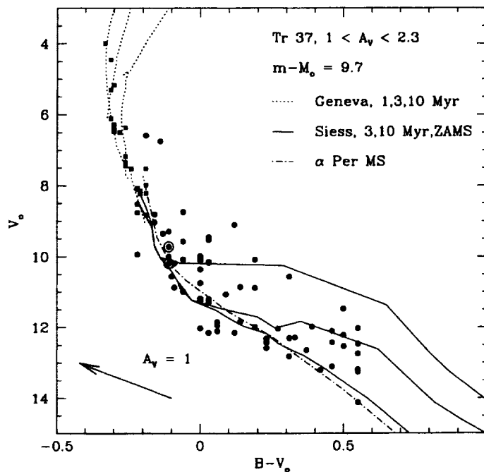
Figure 1: Color-magnitude diagram for probable members of Tr 37. The dotted curves are isochrones for high mass stars with Z = 0.02 from Schaller et al. (1992) for ages of 1, 3, and 10 Myr; the solid curves are isochrones from Siess et al. (2000) for 3 and 10 Myr, and the ZAMS; and the dot-dashed line is the dereddened main sequence of the \alpha Per cluster (J. Stauffer, personal communication; see also Pinsonneault et al. (1998). Circled objects are the emission-line stars in our survey; the large cross denotes MVA 805, which has no emission lines but exhibits an infrared excess. (MVA 60 = LkHa 349 has an uncertain spectral type and therefore cannot be dereddened; its large B-V=2 indicates that it is probably heavily extinguished.)
