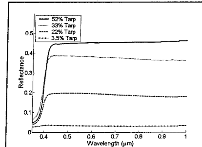
Figure 8. Measured tarp reflectance values
