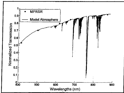
Figure 9. Atmospheric transmission
