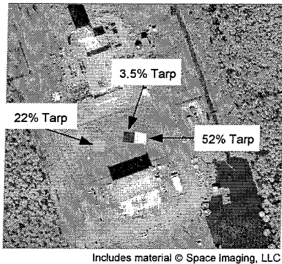
Figure 6. IKONOS image of tarp layout at SSC
