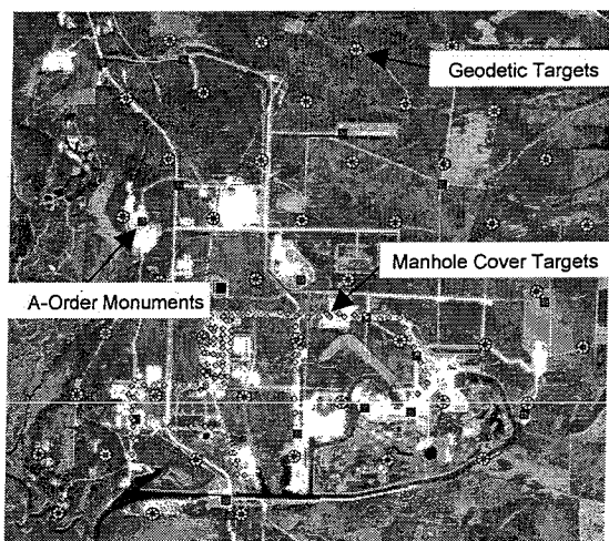
Figure 2. Target positions throughout SSC fee area
