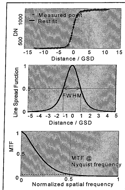
Figure 5. MTF calculation
