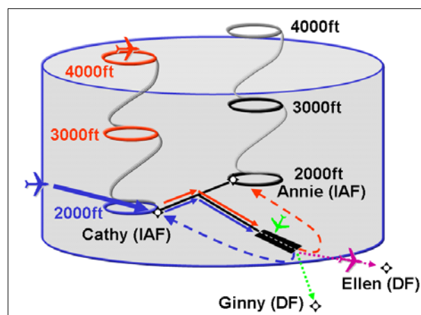
Fig. 1. Nominal SCA and approach geometry
