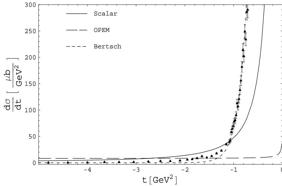
Figure 27: The OPEM ( g_{\pi NN} = 3.751 ), scalar theory ( g = 7.489 GeV) and the parameterization of Bertsch ( a = 25.67 mb/GeV 2 ) [13] compared to data from Baglin et al. [19] at p_{lab} = 9.0 GeV.
