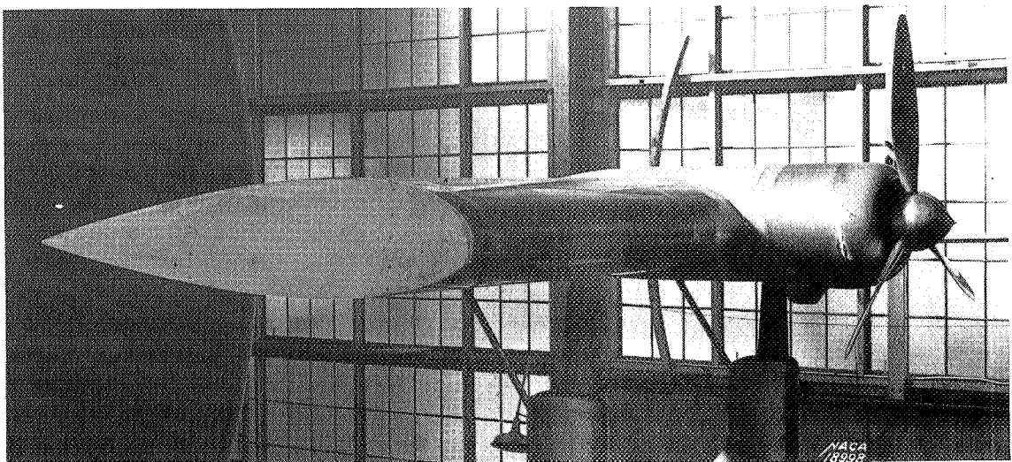
Figure 5.- Bottom opening with adjustable flap test set-up.
