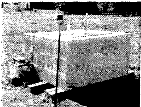
Figure 1: Experimental configuration with our PNG and a LaBr 3 gamma ray spectrometer on top of the granite formation at our test site.
