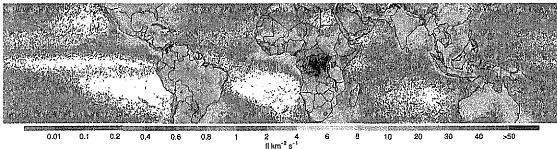
Figure 1 – Total lightning flash rate density ( \text{fl km}^{-2} \text{yr}^{-1} ) derived from 13 years (1998-2010) of TRMM LIS observations.
