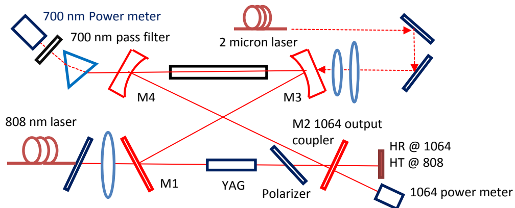
Figure 1. Schematic of up-conversion experimental setup
