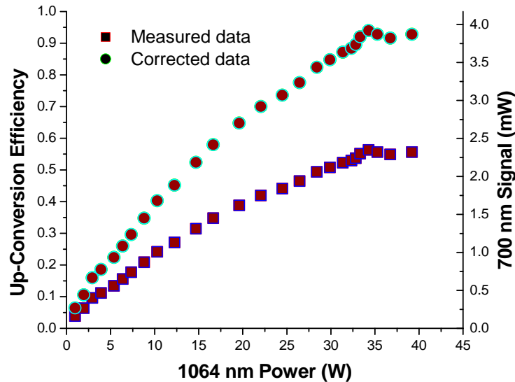
Figure 2. Pump laser power dependence and up-conversion efficiency
