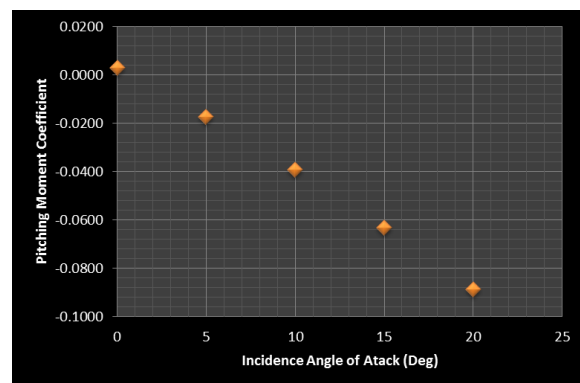
Figure 10: Static stability condition is satisfied for MIRCA
